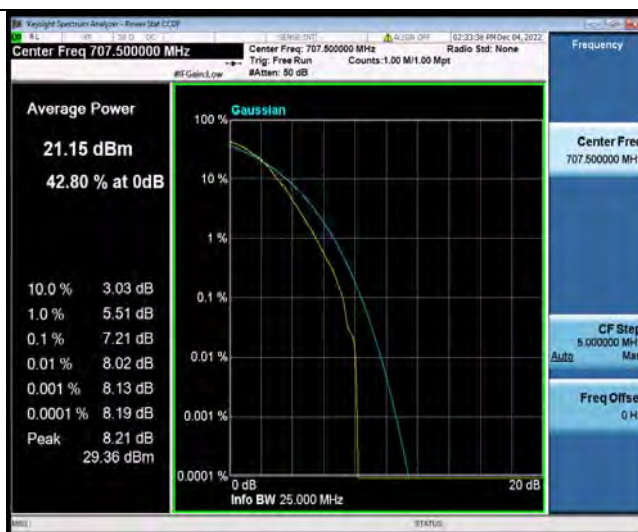
Band12-1.4MHz-64QAM-23095-6RB#0
