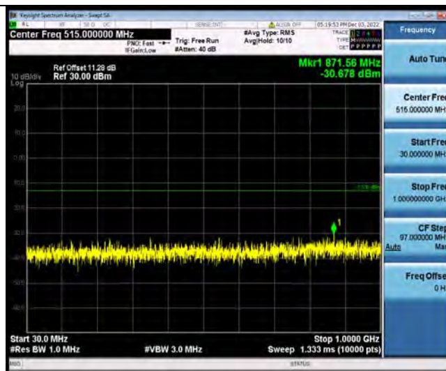
Band4-1.4MHz-64QAM-20175-1RB#0-Range2:1000~20000MHz
