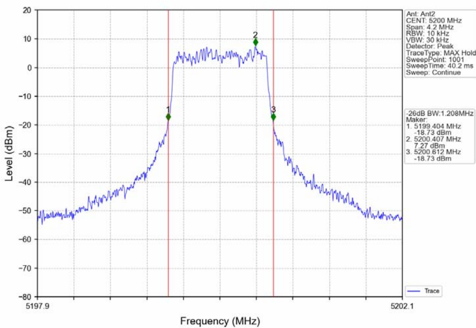
16QAM 1.4MHz_MCH_5200MHz_Ant2_NTNV
