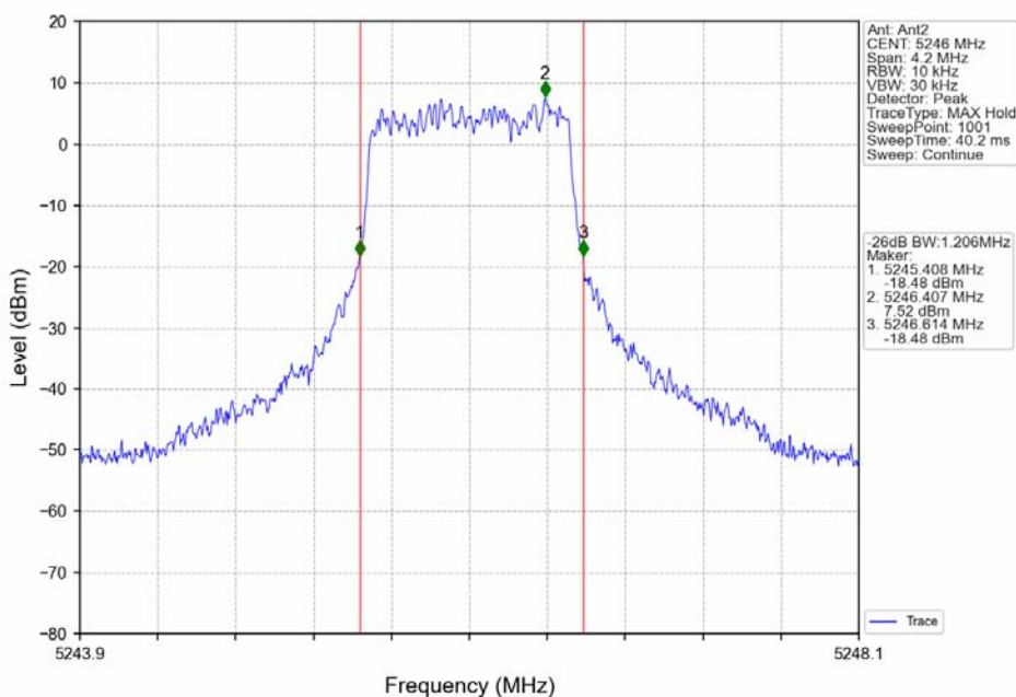
16QAM 1.4MHz_HCH_5246MHz_Ant2_NTNV
