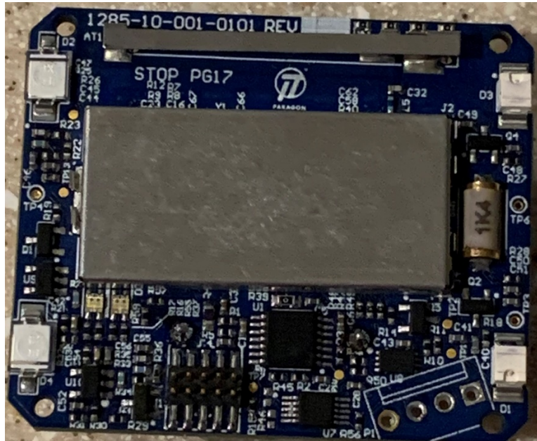
Top of BLUband with Shield Installed
