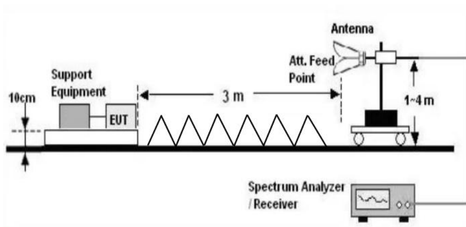
Figure 3. Above 1 GHz
