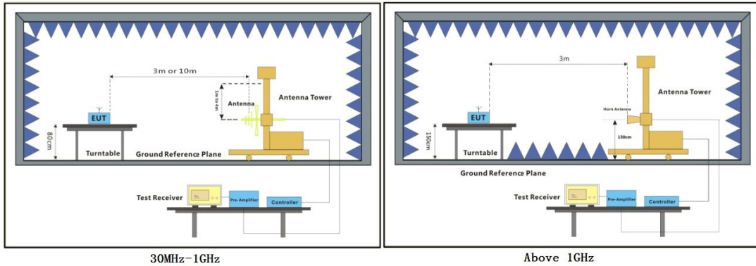
30MHz-1GHz
