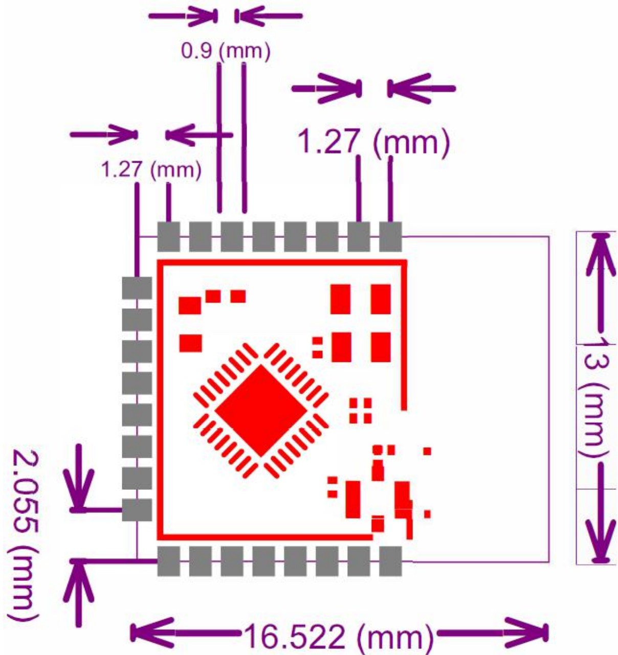
Figure 1 Chip Dimensions
