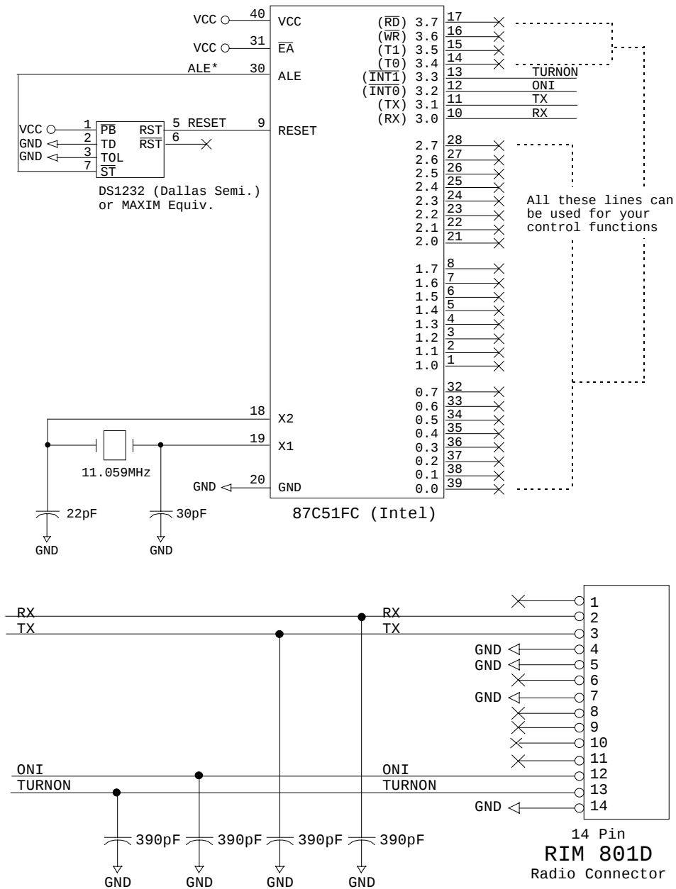
Figure 13: Simple 8051 Interface
