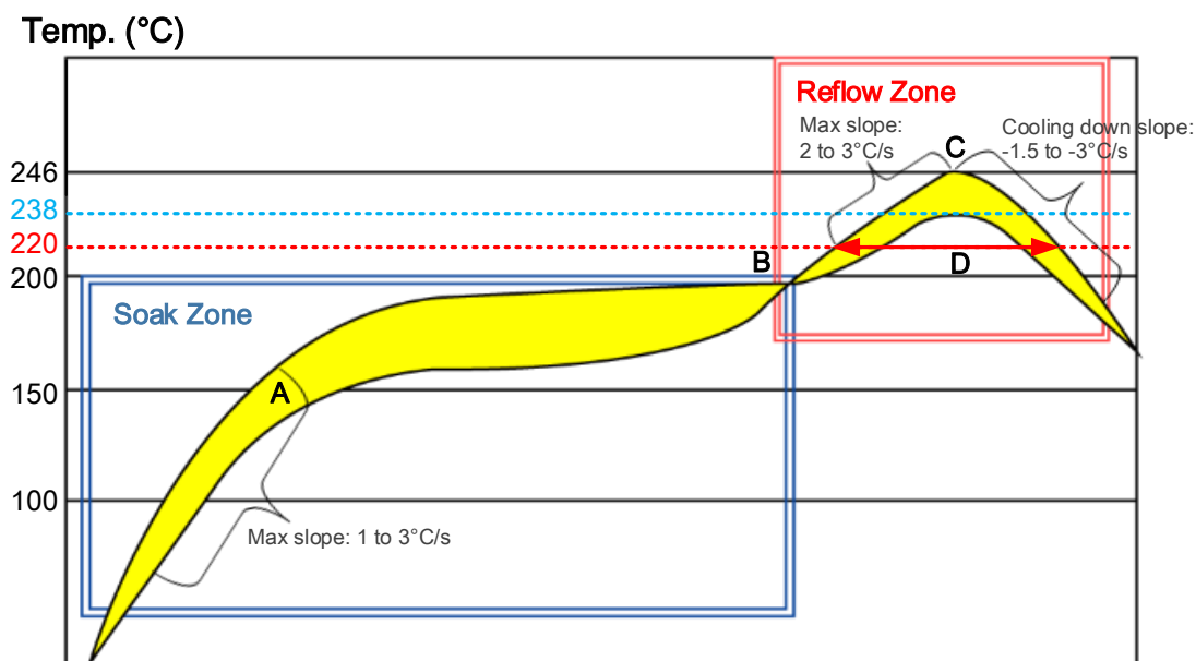
Figure 49: Reflow Soldering Thermal Profile
