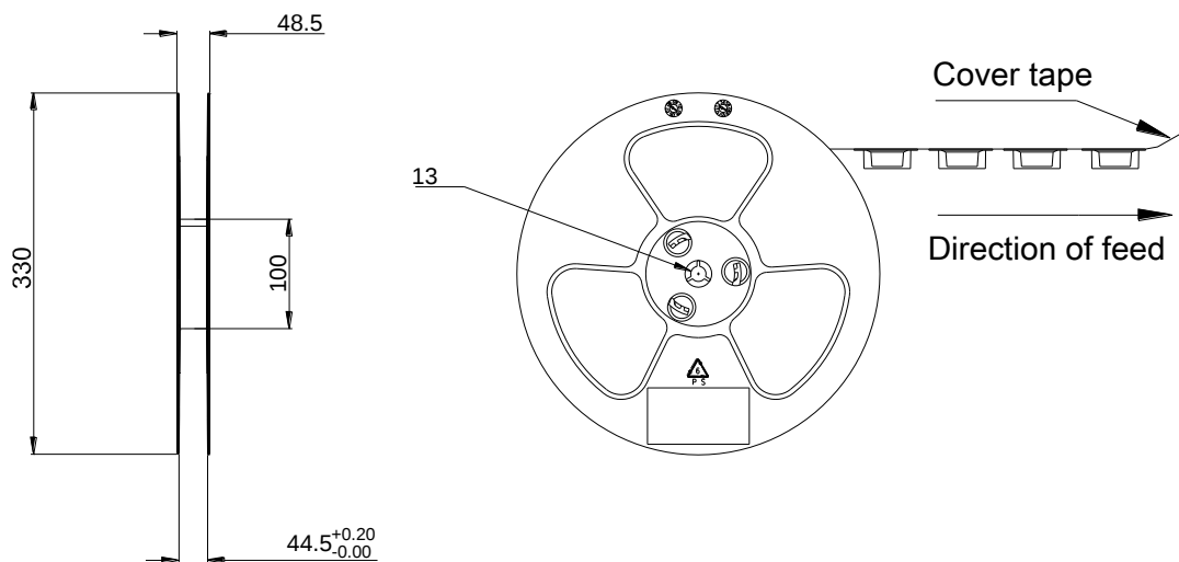
Figure 51: Reel Specifications
