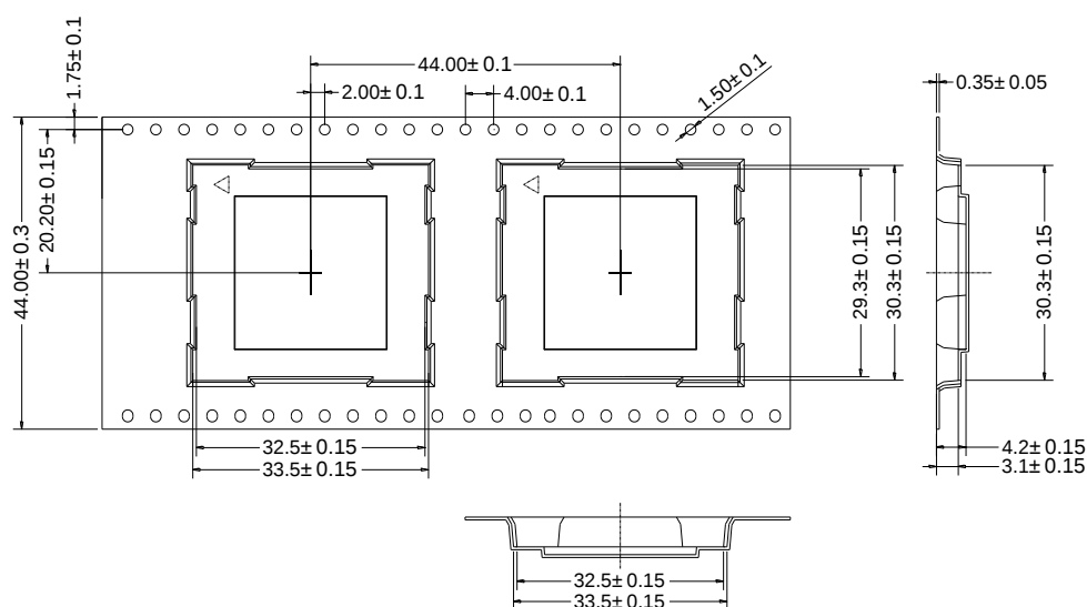
Figure 50: Tape Specifications
