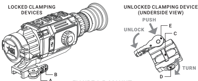
FIGURE 2-5. MOUNT
