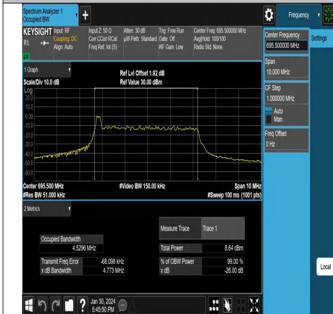
NTNV_N71_PC3_15_5_H_TID3_Ant1#1
