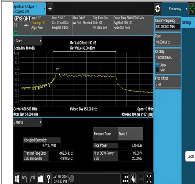
NTNV_N71_PC3_15_5_M_TID3_Ant1#1
