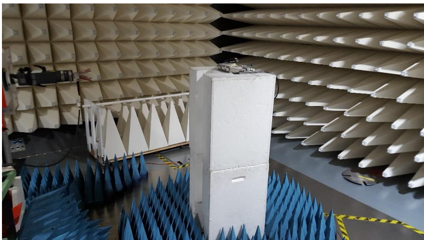
Figure D7. High Range Radiated Emission test setup 18-26GHz
