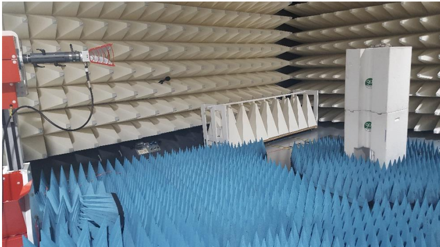
Figure D6. High Range Radiated Emission test setup 1-18GHz
