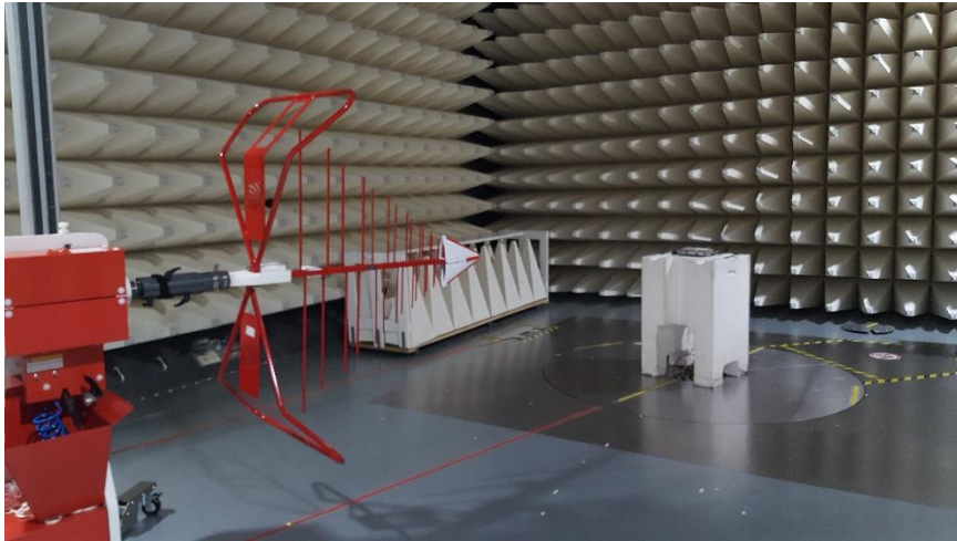
Figure D5. Low Range Radiated Emission test setup
