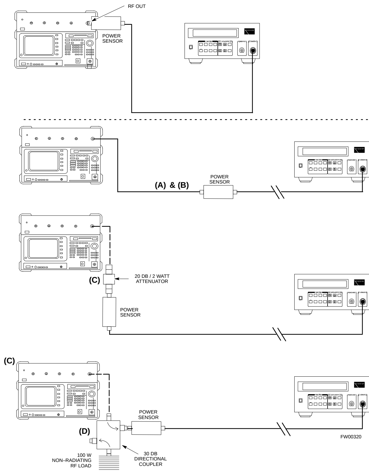
Figure F-6: Cable Calibration using Advantest R3465
