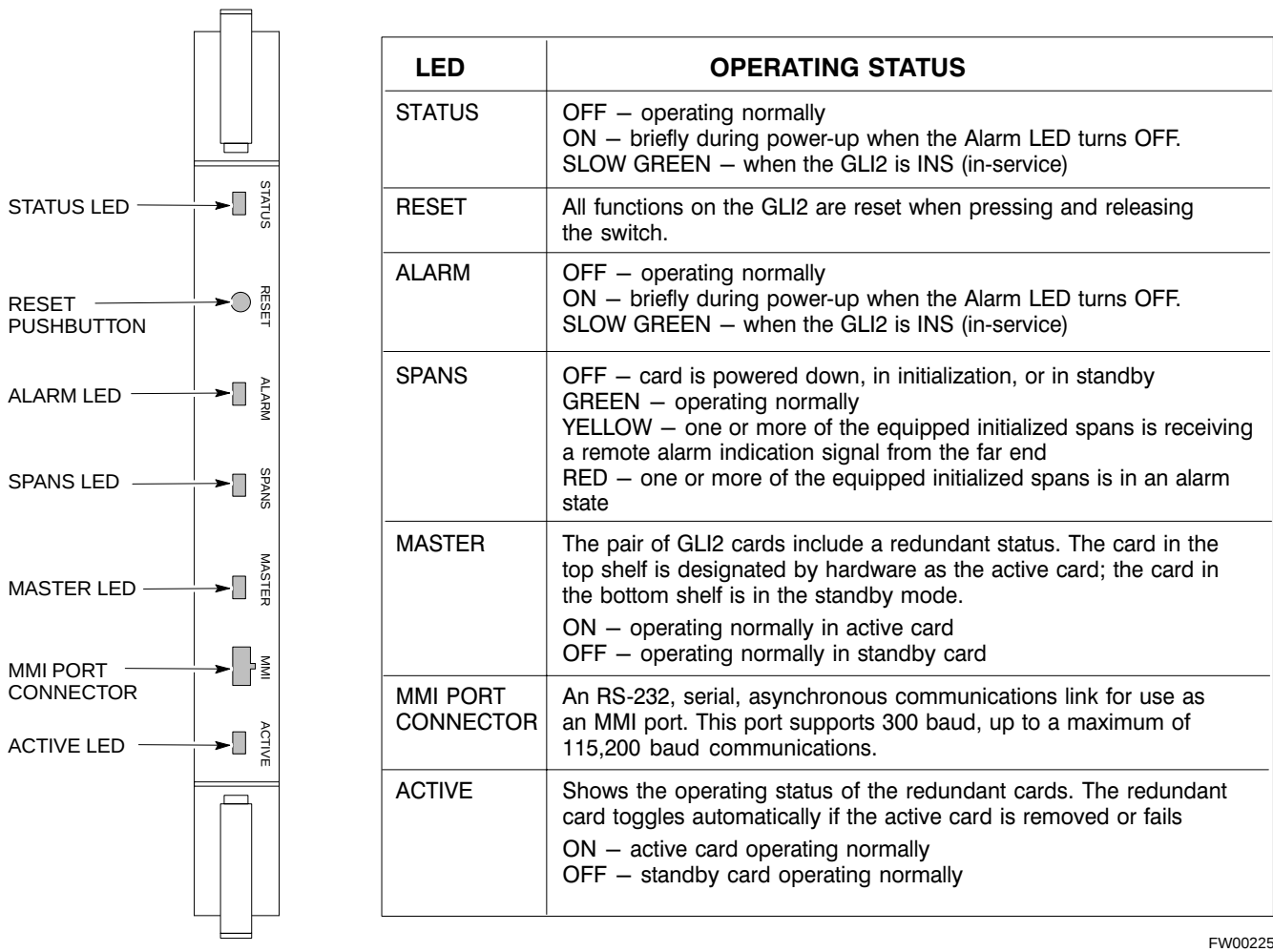
Figure 6-2: GLI2 Front Panel Operating Indicators
