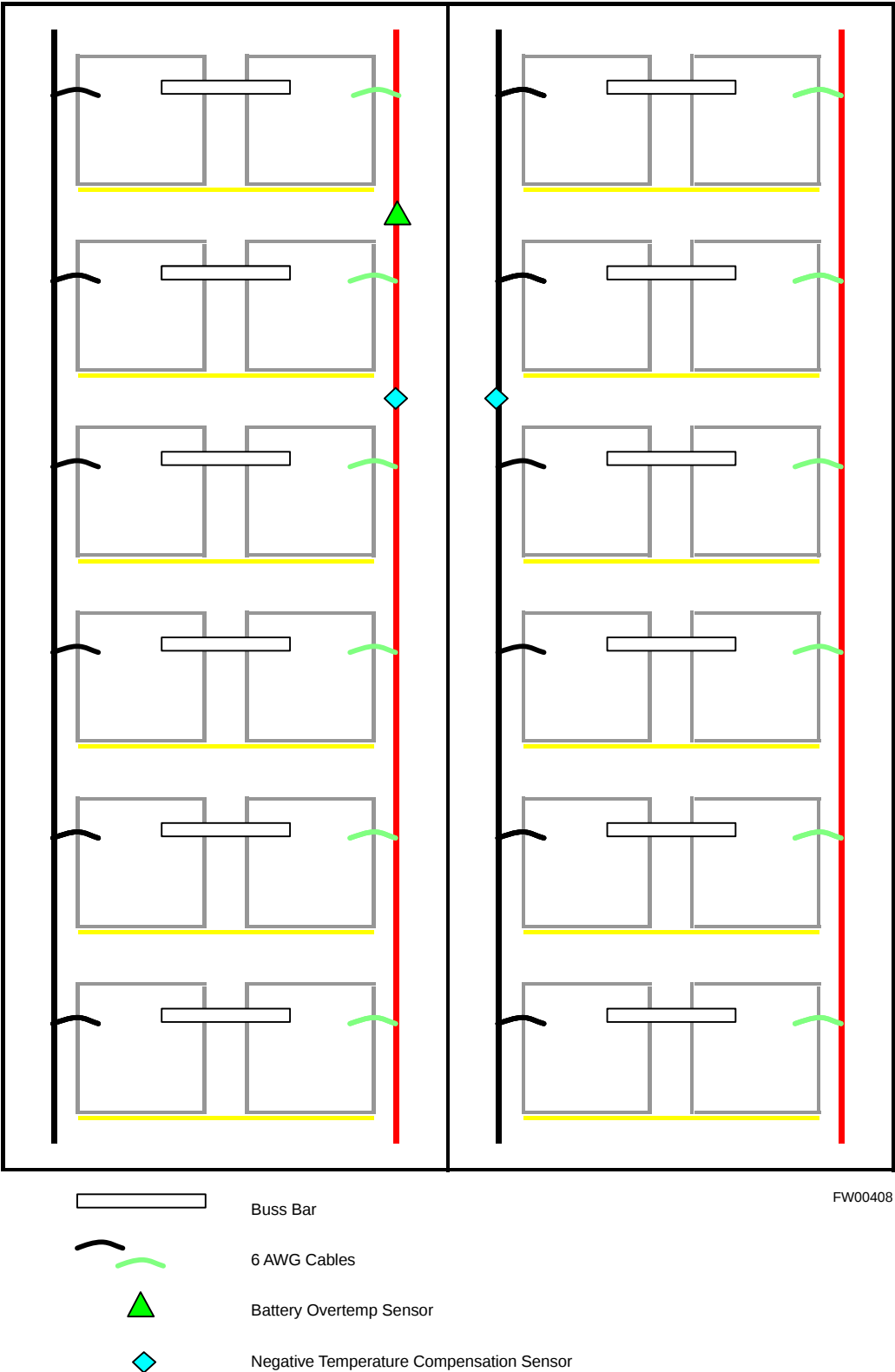
Figure 3-15: Battery Overtemperature Sensor
