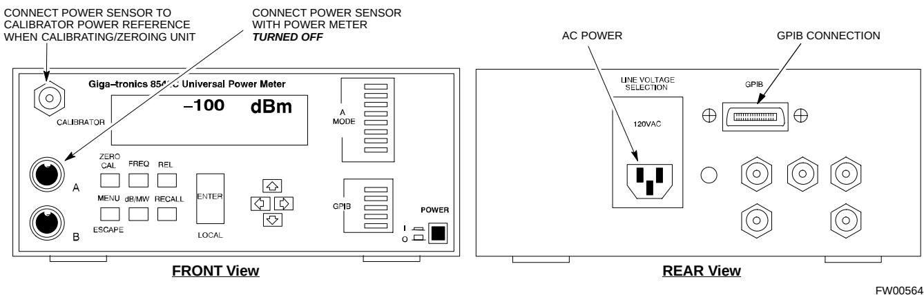
Figure F-8: Gigatronics 8542C Power Meter Detail
