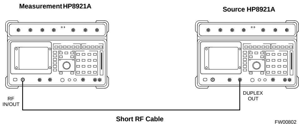
Figure G-2: Delta Calibration Setup – HP8921A to HP8921A
