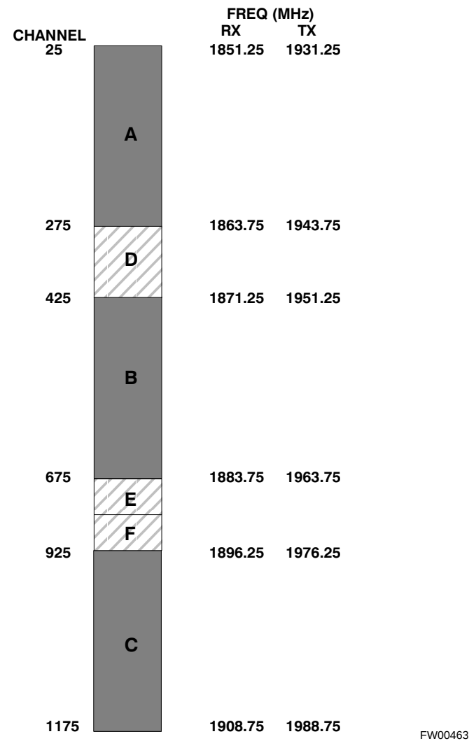
Figure D-1: North America PCS Frequency Spectrum (CDMA Allocation)
