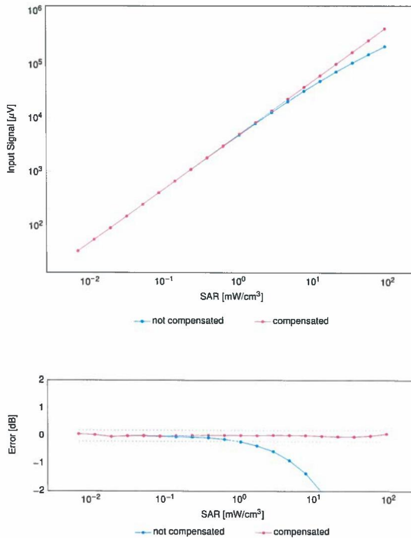
Dynamic Range f(\text{SAR}_{\text{head}}) (TEM cell, f_{\text{eval}} = 1900\text{MHz} )
