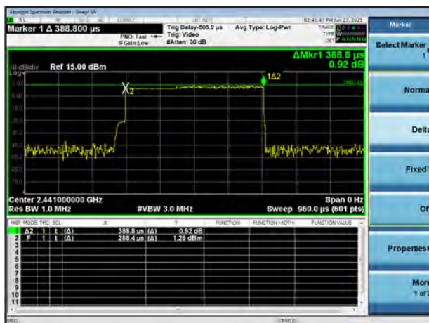
8-DPSK DH1
