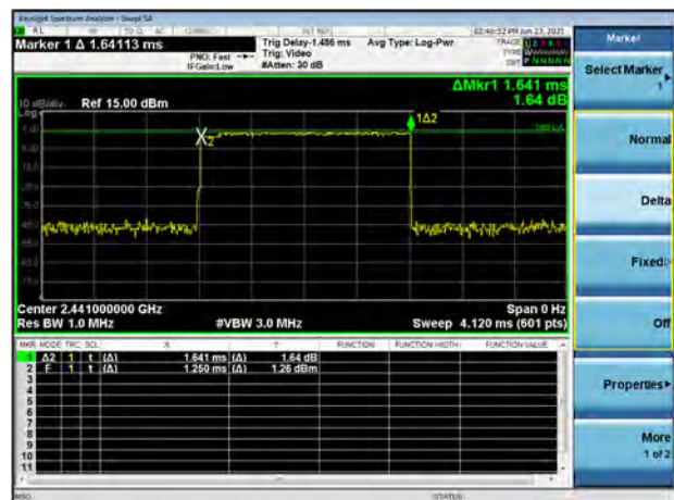
8-DPSK DH3
