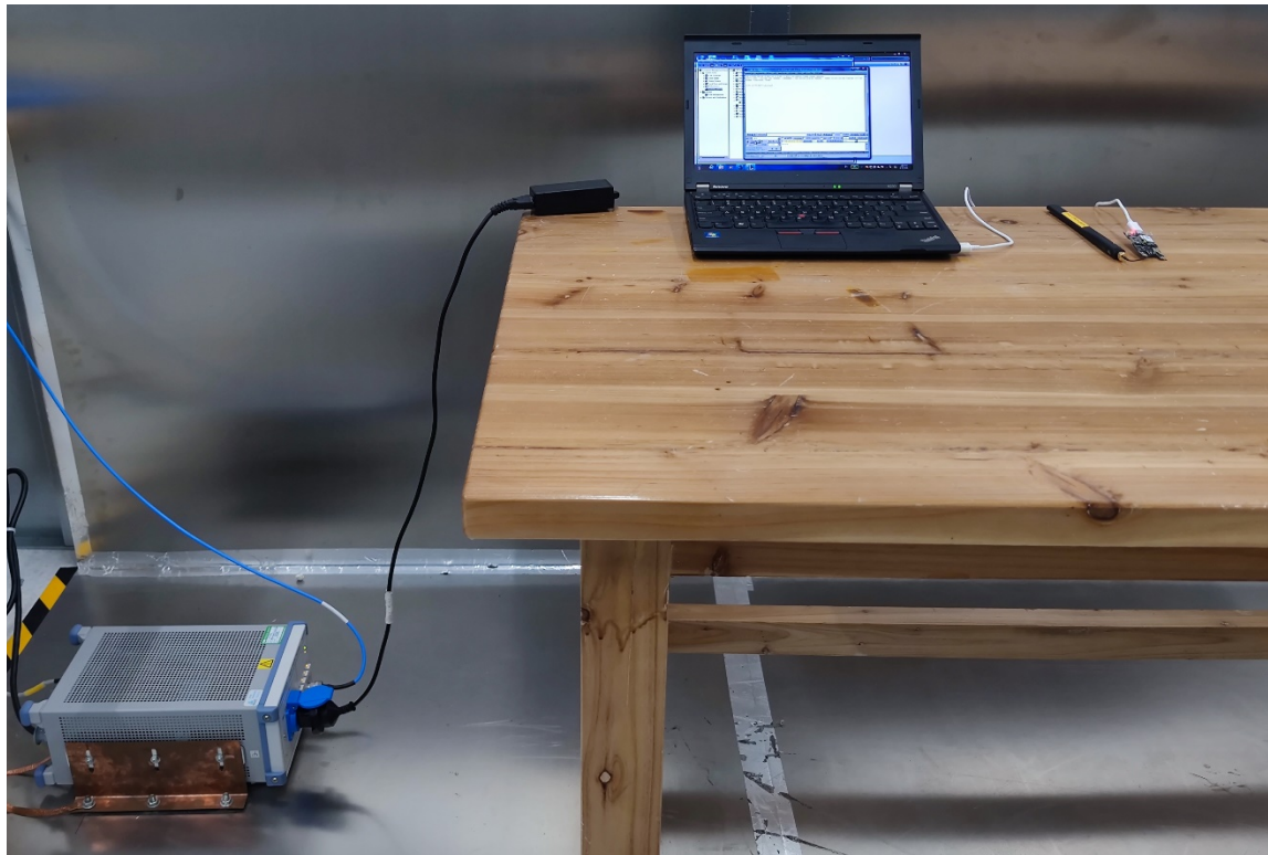
Photograph 3: Set-up for Conducted Emission on AC mains
