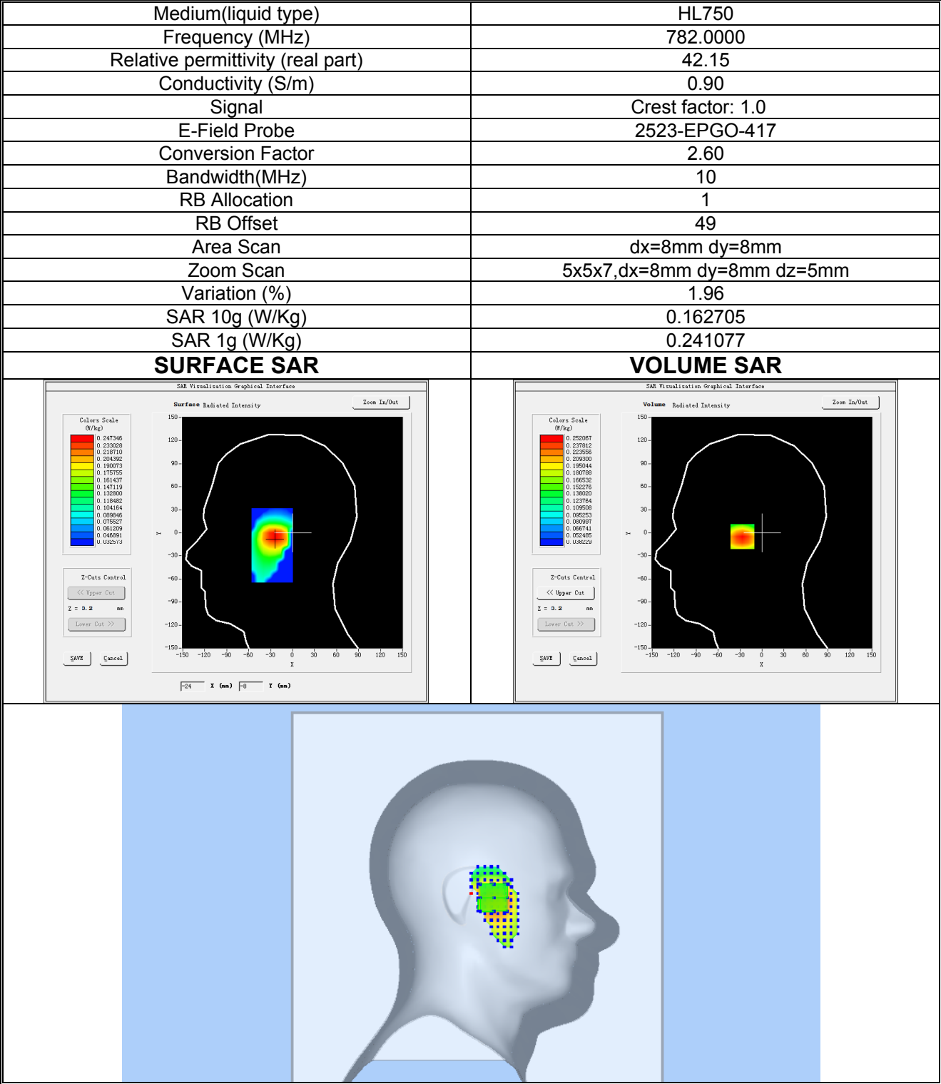
Plot 21:LTE BAND 13, Low channel (Left Head Cheek) Product Description: Smart Phone Test Date: 2024-04-01
