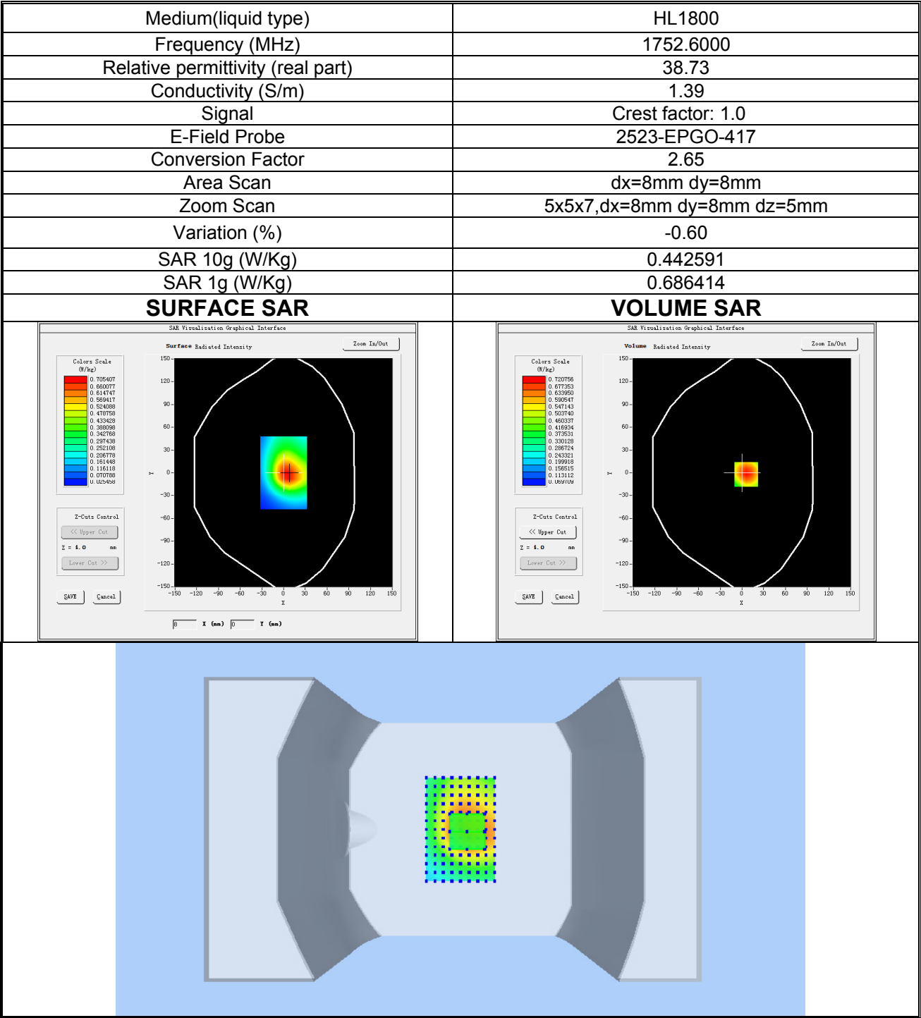
Plot 8: WCDMA BAND IV, High channel (Body-worn/Hotspot, Front Side) Product Description: Smart Phone Test Date: 2024-03-26
