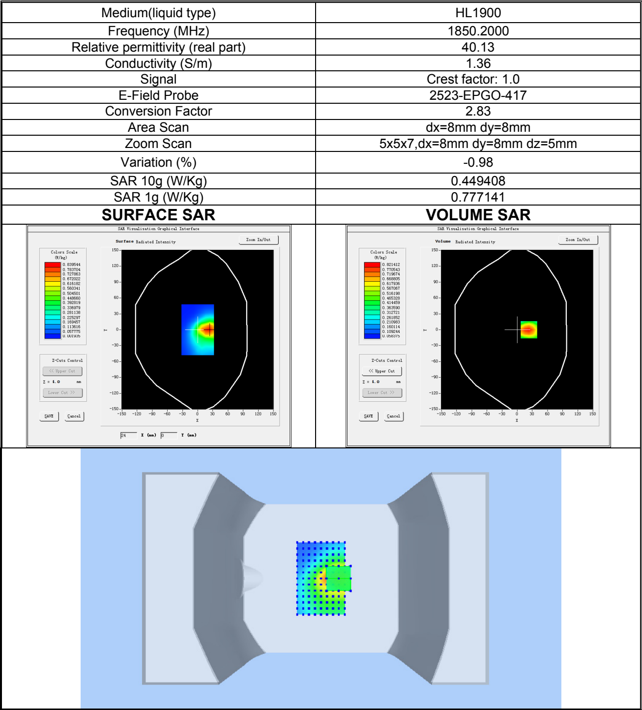
Plot 4: GPRS1900, Low channel (Body-worn /Hotspot, Back Side) Product Description: Smart Phone Test Date: 2024-03-27
