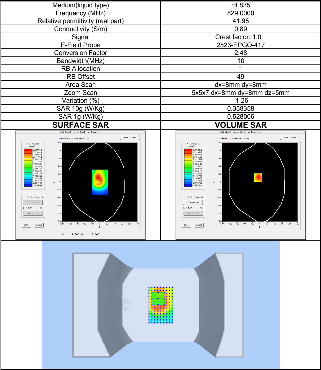
Plot 16: LTE BAND 5, Low channel (Body-worn/ Hotspot, Back Side) Product Description: Smart Phone Test Date: 2024-04-01
