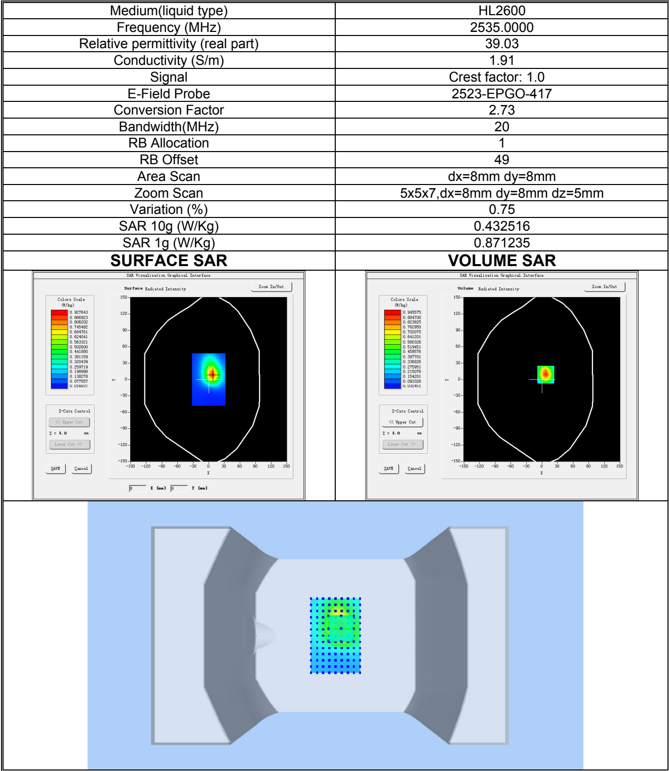
Plot 18: LTE BAND 7, Middle channel (Body-worn/ Hotspot, Bottom Edge) Product Description: Smart Phone Test Date: 2024-03-30
