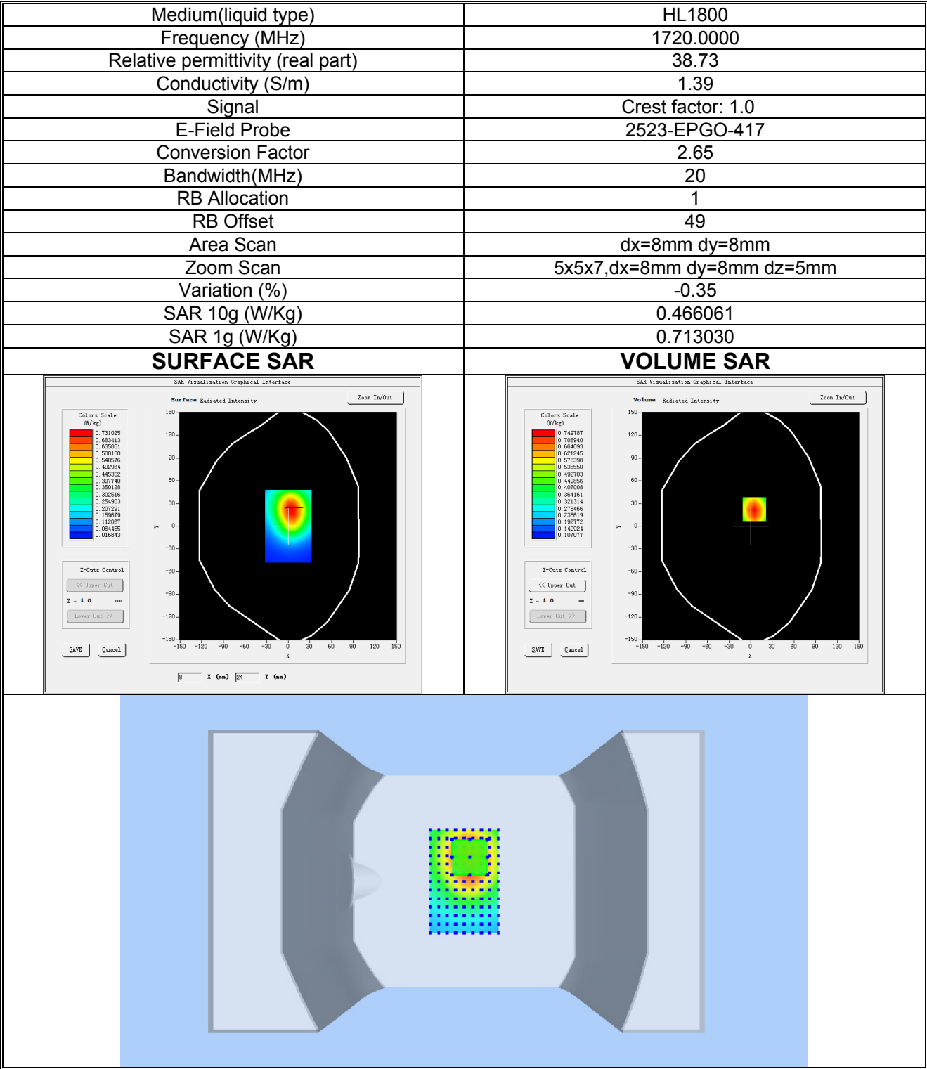
Plot 14: LTE BAND 4, Low channel (Body-worn/ Hotspot, Bottom Edge) Product Description: Smart Phone Test Date: 2024-03-26
