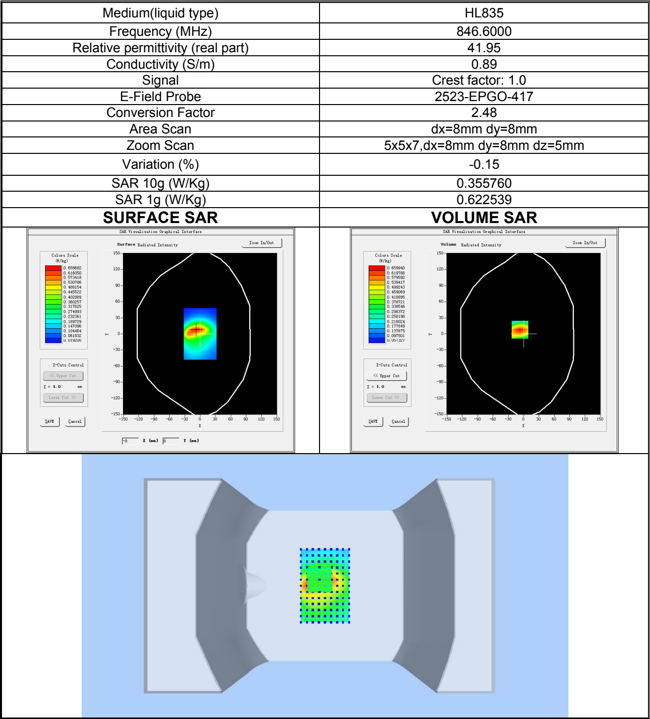
Plot 10: WCDMA BAND V, High channel (Body-worn/Hotspot, Front Side) Product Description: Smart Phone Test Date: 2024-04-01
