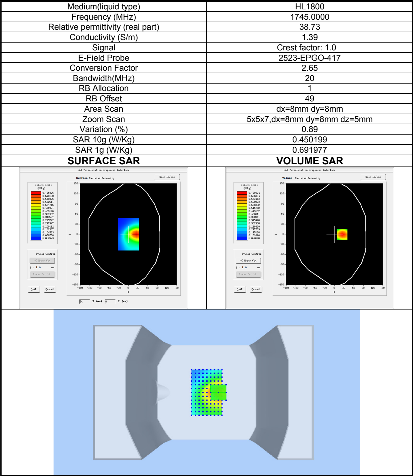
Plot 24: LTE BAND 66, Middle channel (Body-worn/ Hotspot, Back Side) Product Description: Smart Phone Test Date: 2024-03-26
