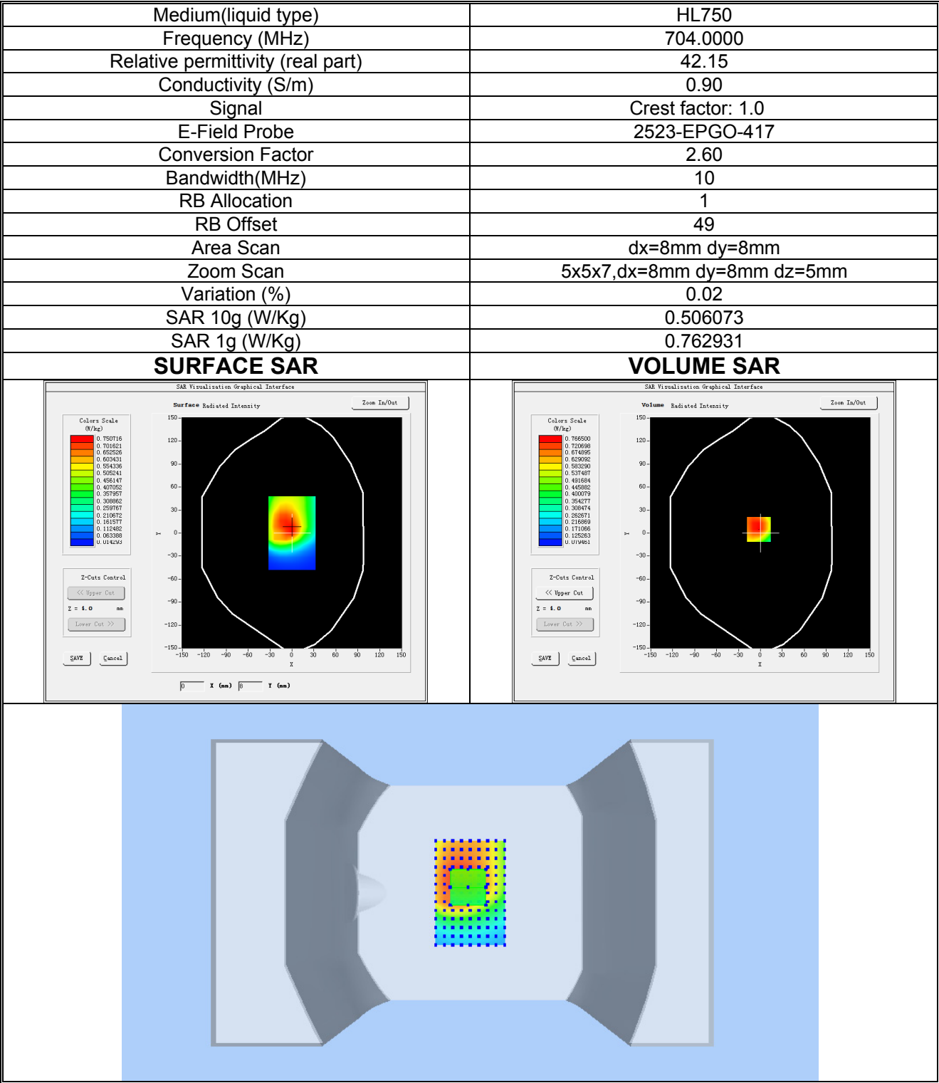
Plot 20: LTE BAND 12, Low channel (Body-worn/ Hotspot, Back Side) Product Description: Smart Phone Test Date: 2024-04-01
