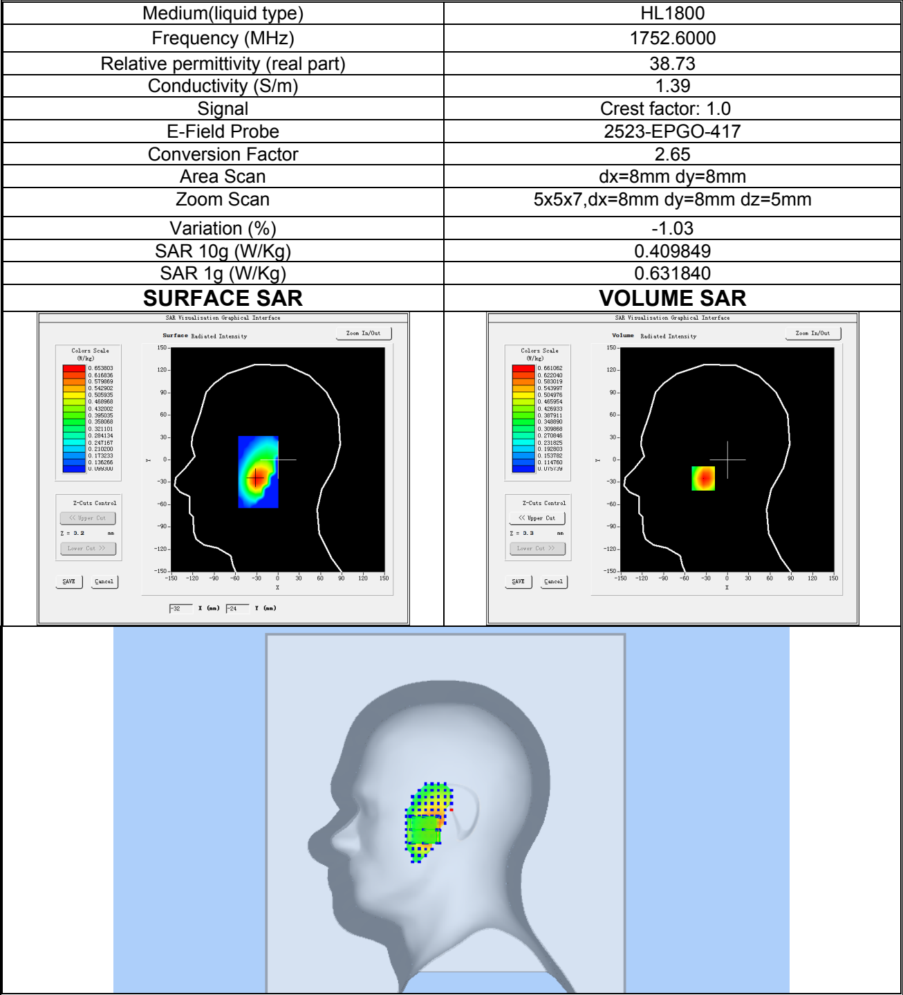
Plot 7: WCDMA BAND IV, High channel (Right Head Cheek) Product Description: Smart Phone Test Date: 2024-03-26
