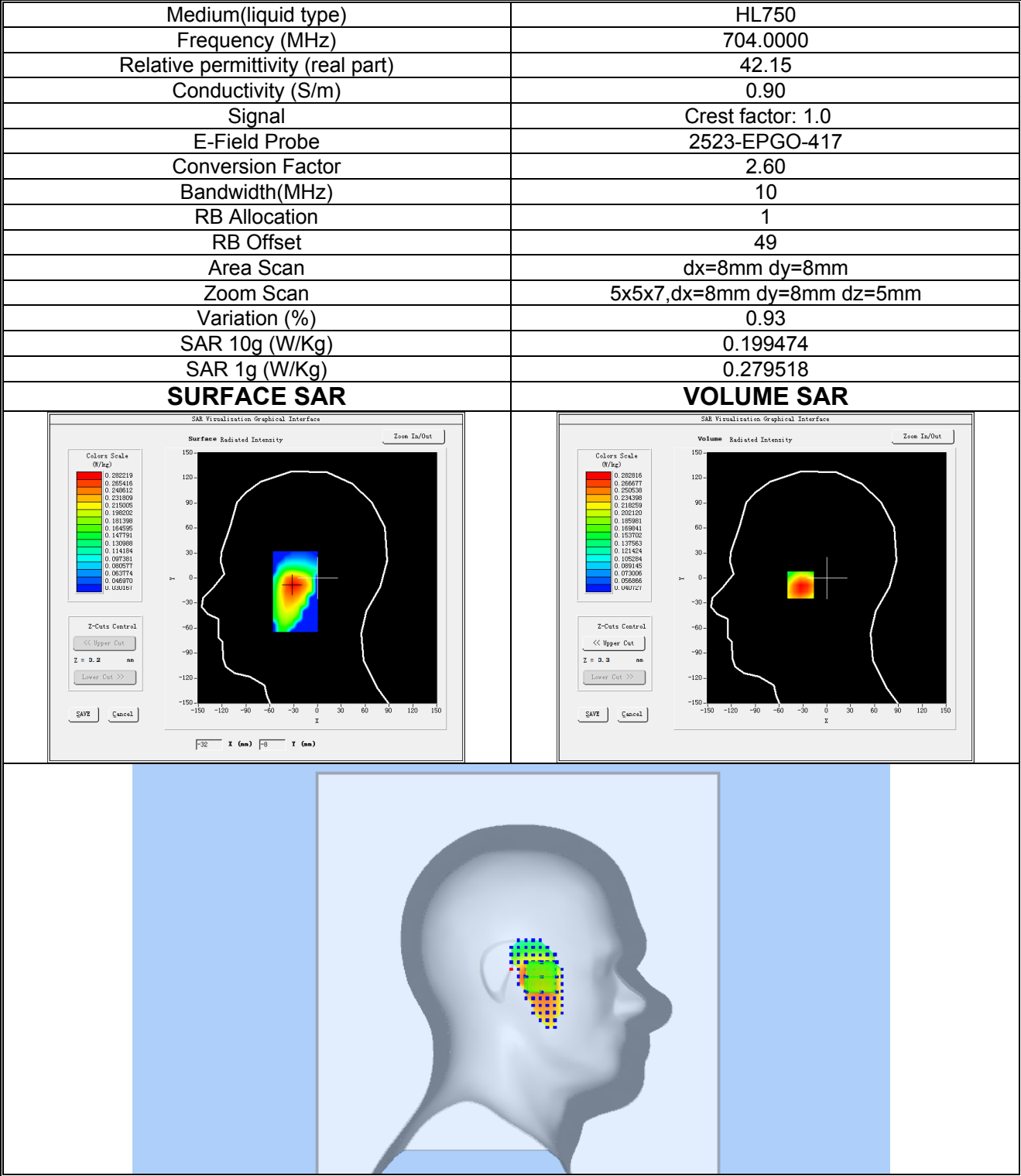
Plot 19:LTE BAND 12, Low channel (Left Head Cheek) Product Description: Smart Phone Test Date: 2024-04-01
