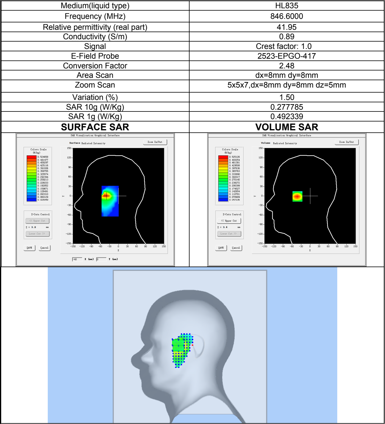
Plot 9: WCDMA BAND V, High channel (Right Head Cheek) Product Description: Smart Phone Test Date: 2024-04-01
