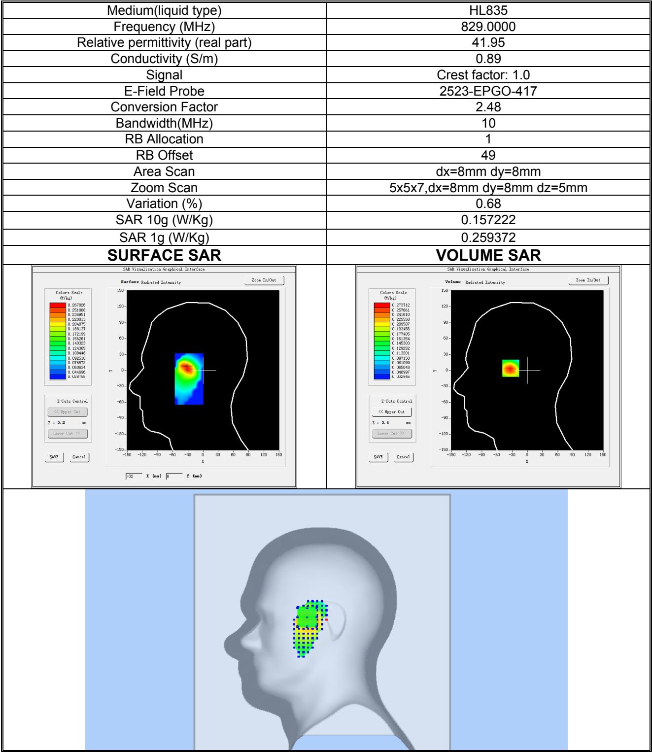
Plot 15:LTE BAND 5, Low channel (Right Head Cheek) Product Description: Smart Phone Test Date: 2024-04-01
