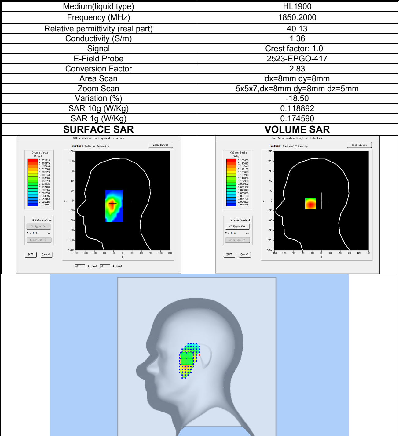
Plot 3: GPRS1900, Low channel (Right Head Cheek) Product Description: Smart Phone Test Date: 2024-03-27
