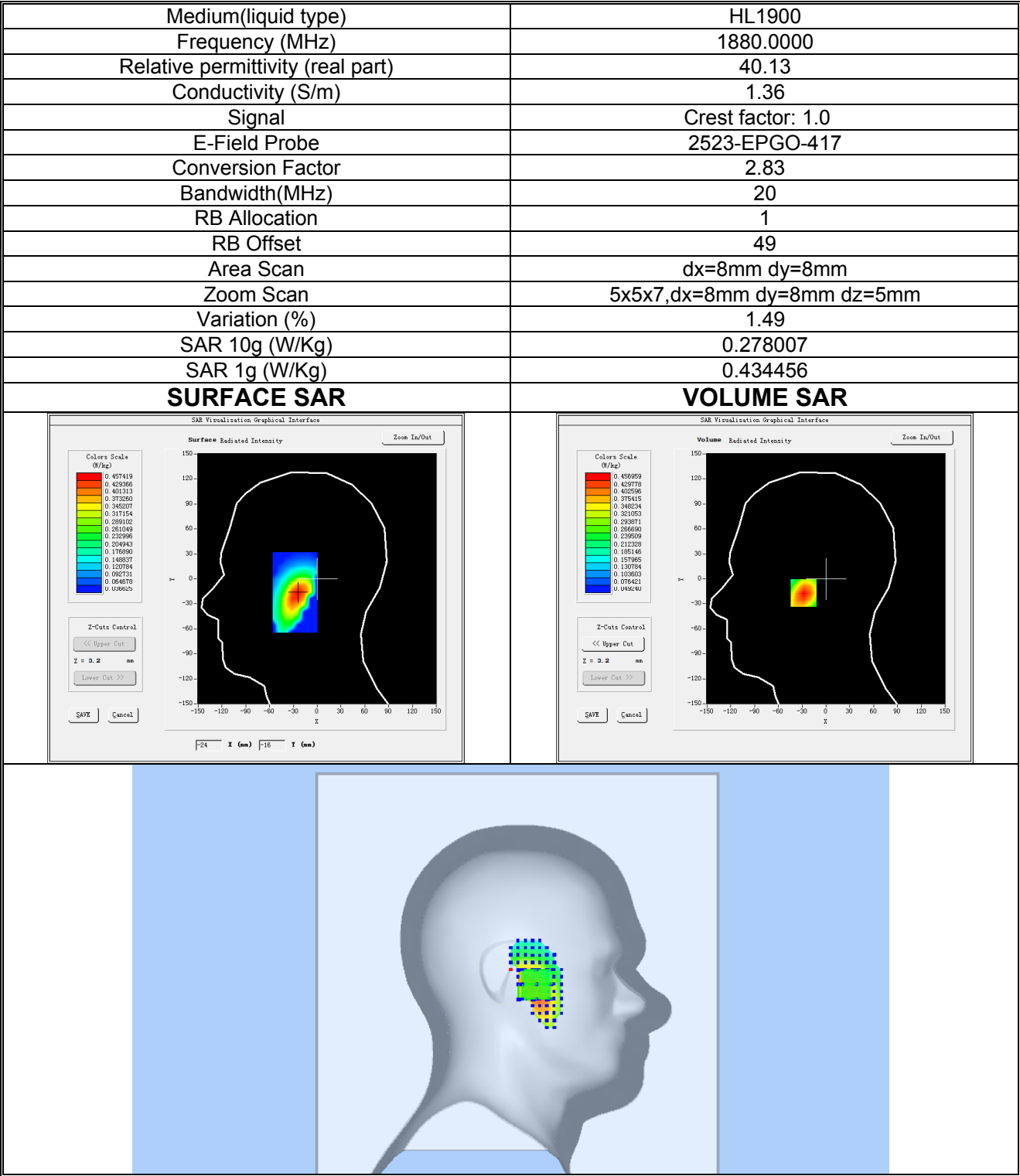
Plot 11:LTE BAND 2, Middle channel (Left Head Cheek) Product Description:Smart Phone Test Date: 2024-03-27
