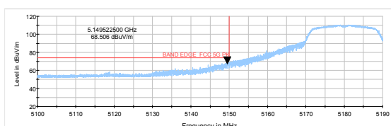
802.11n HT20-Channel 36: Peak
