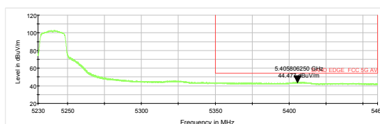
802.11n HT20-Channel 48: Peak
