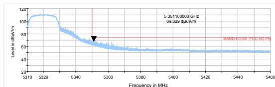
802.11a-Channel 64: Average
