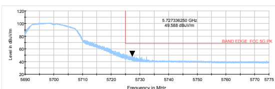
802.11a-Channel 140: Peak
