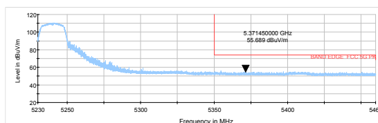
802.11a-Channel 48: Average
