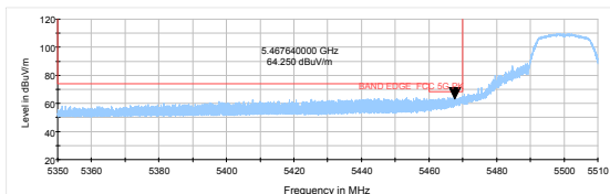
802.11a-Channel 100: Peak
