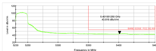
802.11n HT20-Channel 48: Average
