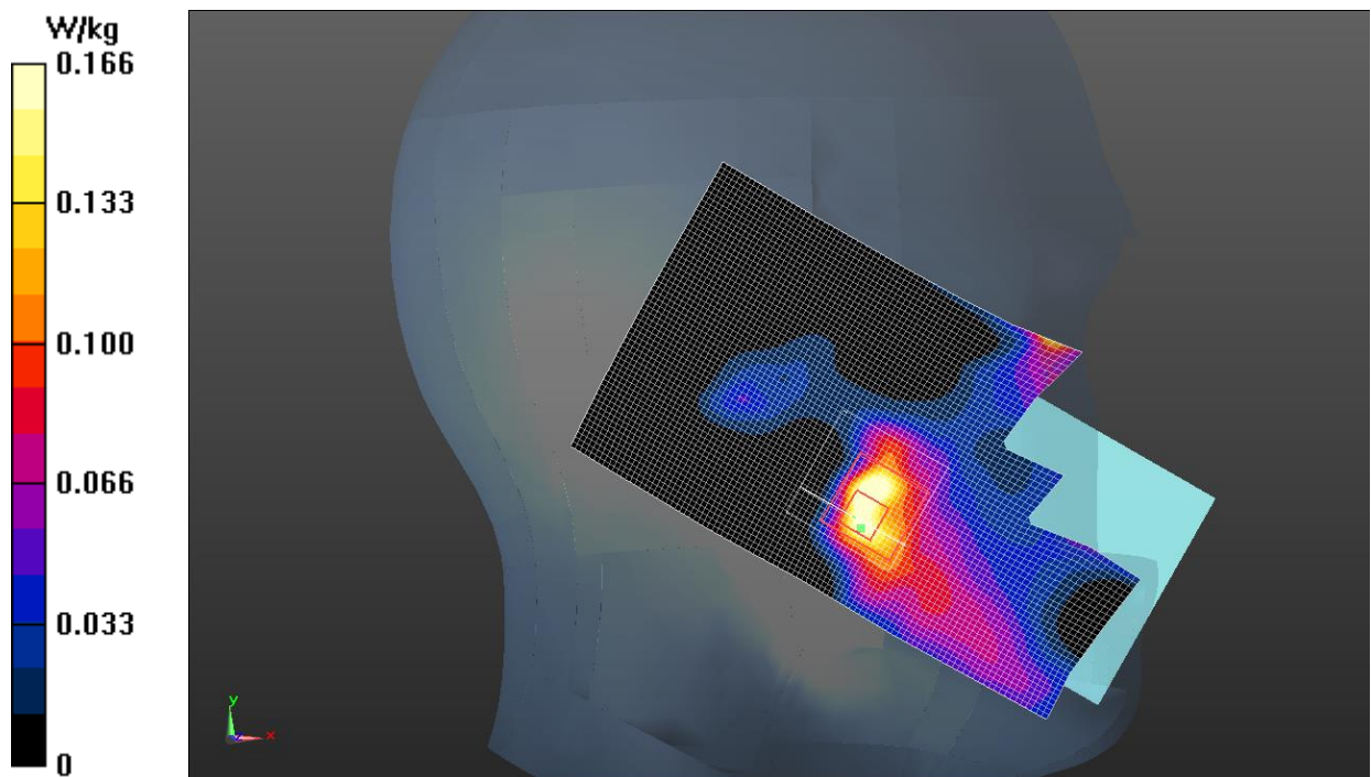
Fig.23 LTE Band 7
