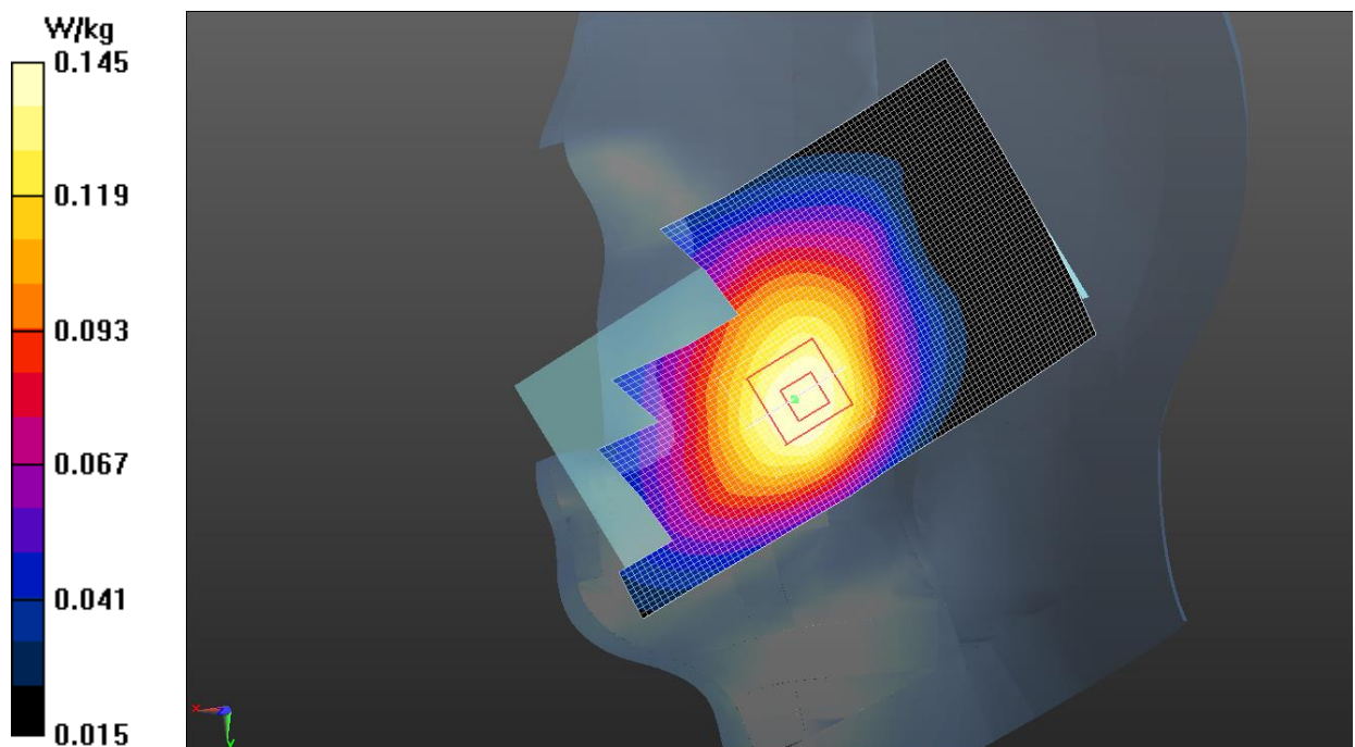
Fig.27 LTE Band 13
