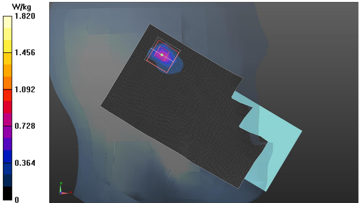
Fig.41 Wi-Fi 5G
