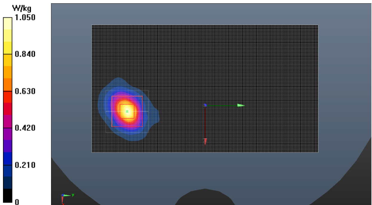
Fig.42 Wi-Fi 5G
