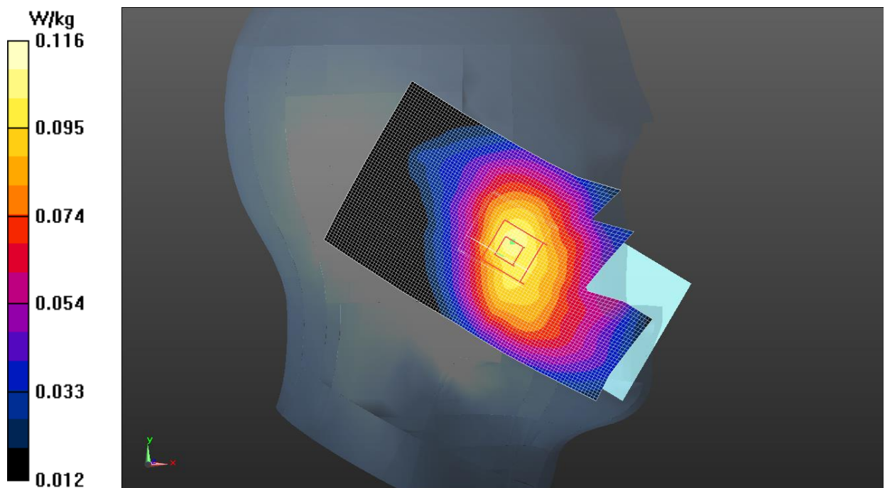
Fig.25 LTE Band 12
