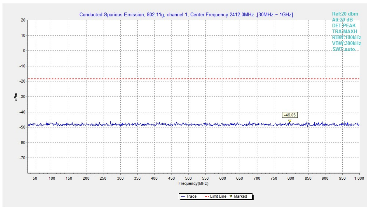
Fig.B.6.1.26 Transmitter Spurious Emission - Conducted (802.11g, Ch1, 30 MHz-1 GHz)
