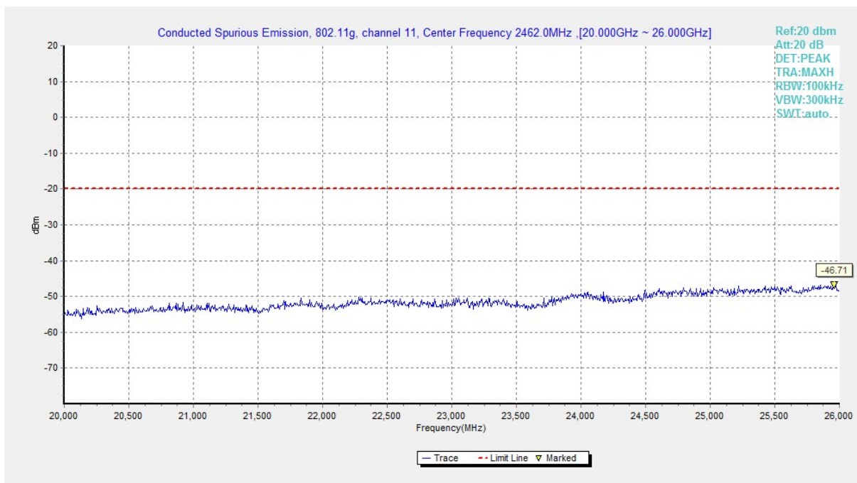
Fig.B.6.1.48 Transmitter Spurious Emission - Conducted (802.11g, Ch11, 20 GHz-26 GHz)
