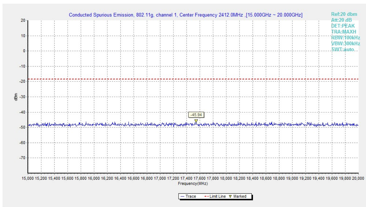
Fig.B.6.1.31 Transmitter Spurious Emission - Conducted (802.11g, Ch1, 15 GHz-20 GHz)
