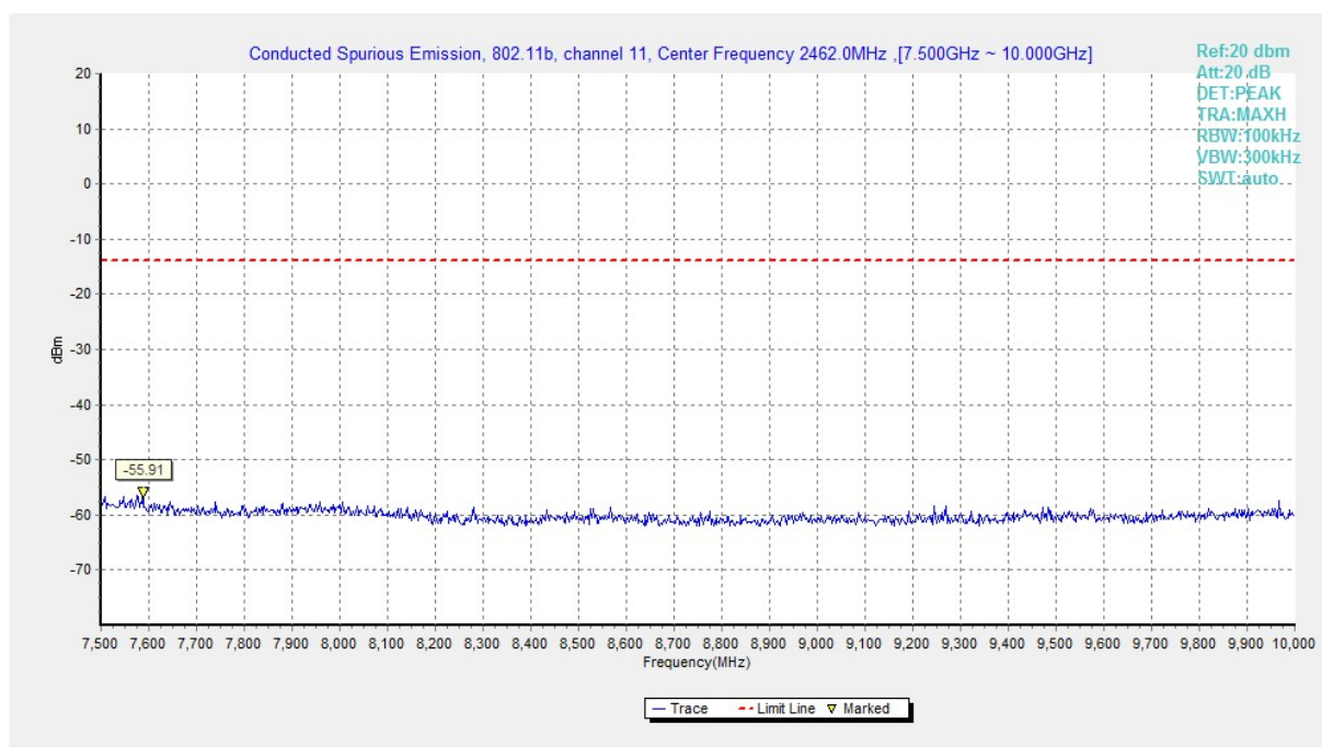
Fig.B.6.1.21 Transmitter Spurious Emission - Conducted (802.11b, Ch11, 7.5 GHz-10 GHz)
