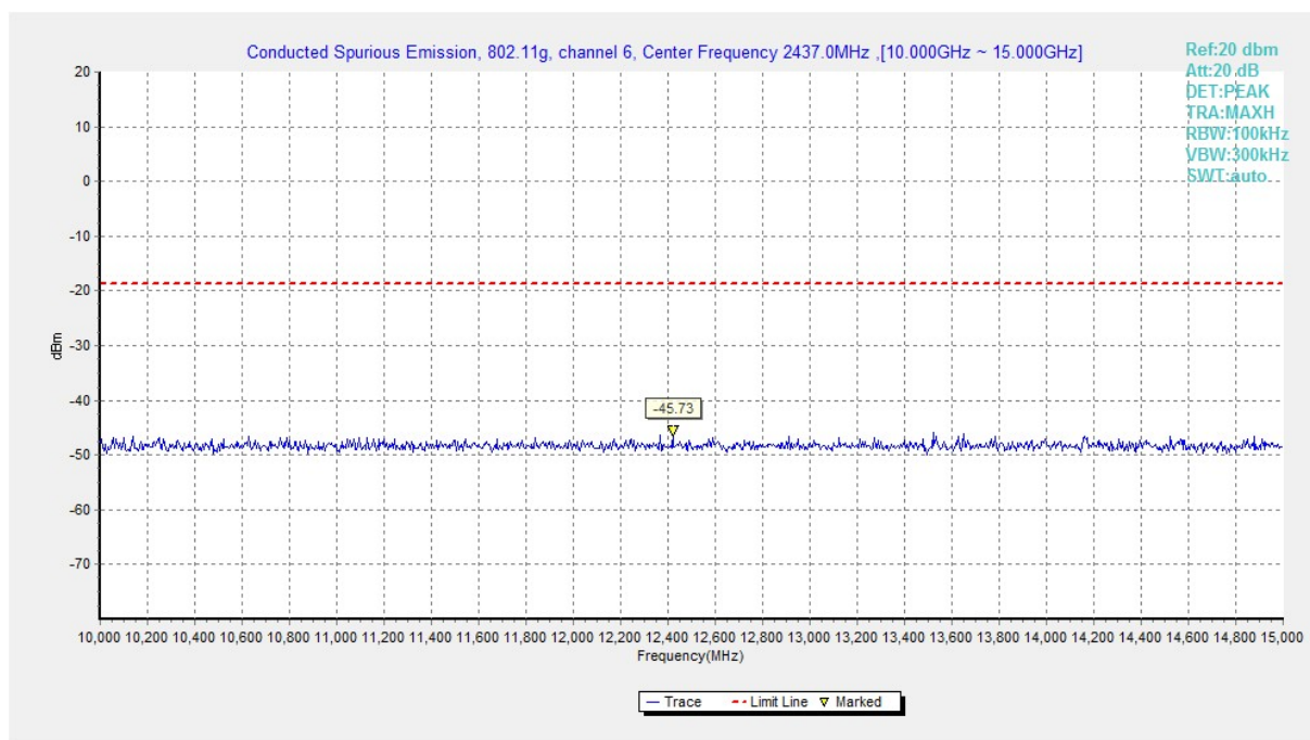
Fig.B.6.1.38 Transmitter Spurious Emission - Conducted (802.11g, Ch6, 10 GHz-15 GHz)
