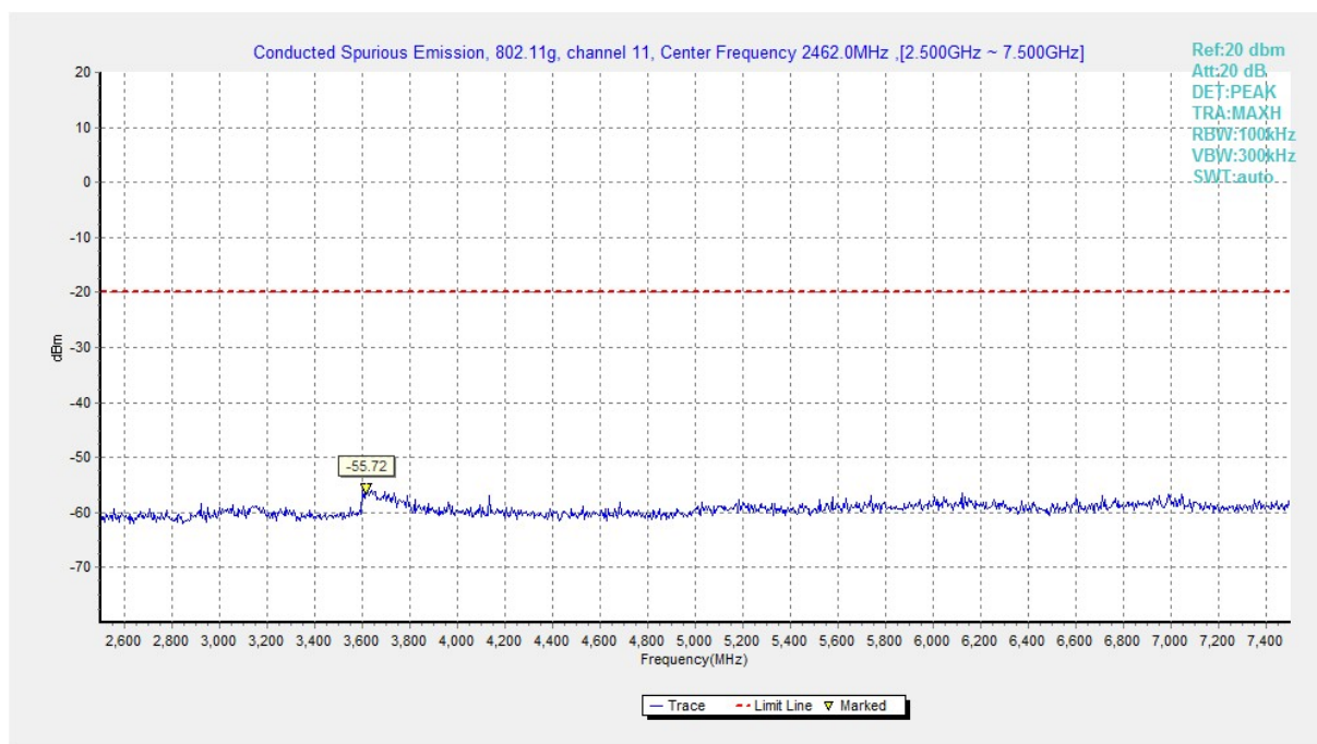
Fig.B.6.1.44 Transmitter Spurious Emission - Conducted (802.11g, Ch11, 2.5 GHz-7.5 GHz)
