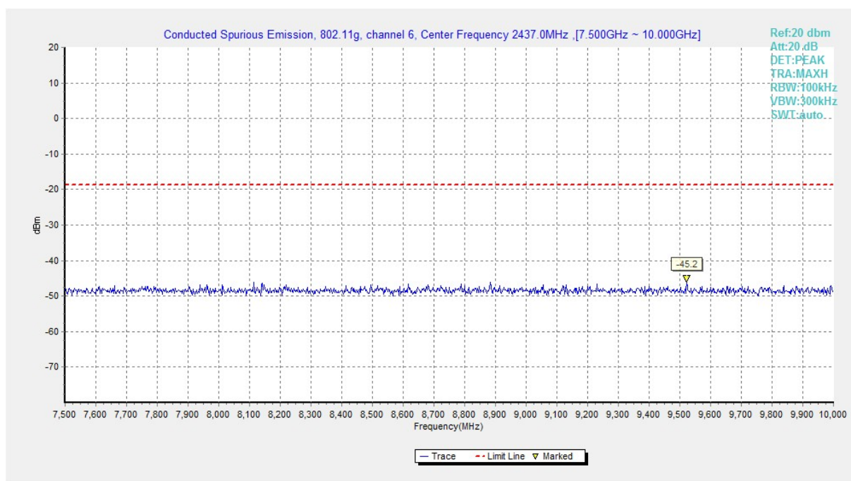
Fig.B.6.1.37 Transmitter Spurious Emission - Conducted (802.11g, Ch6, 7.5 GHz-10 GHz)
