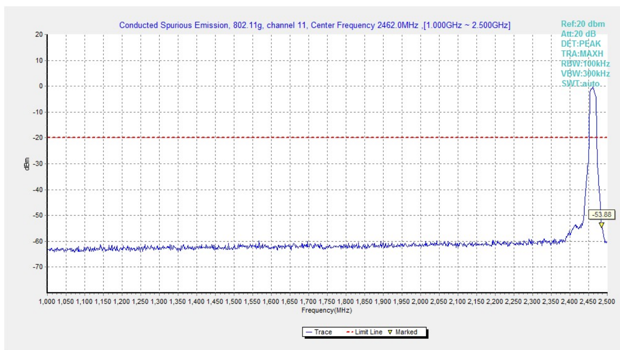
Fig.B.6.1.43 Transmitter Spurious Emission - Conducted (802.11g, Ch11, 1 GHz-2.5 GHz)
