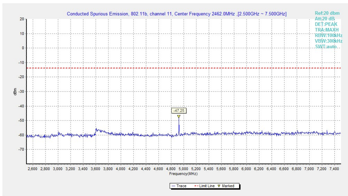
Fig.B.6.1.20 Transmitter Spurious Emission - Conducted (802.11b, Ch11, 2.5 GHz-7.5 GHz)
