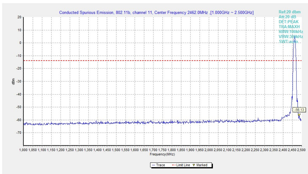
Fig.B.6.1.19 Transmitter Spurious Emission - Conducted (802.11b, Ch11, 1 GHz-2.5 GHz)
