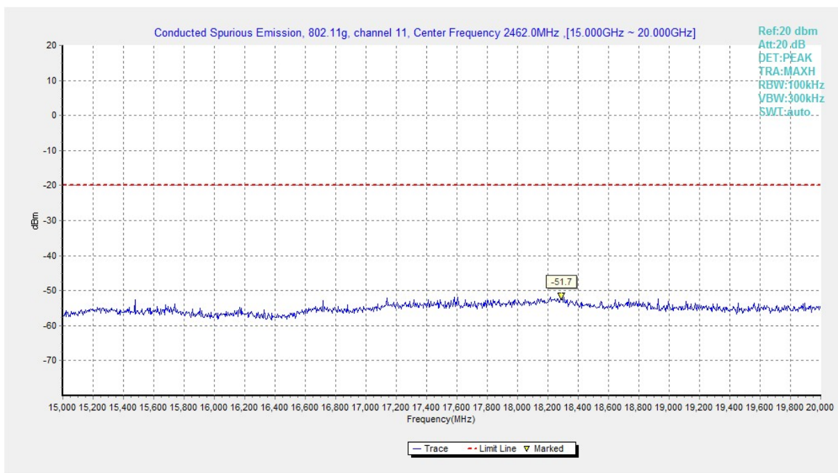
Fig.B.6.1.47 Transmitter Spurious Emission - Conducted (802.11g, Ch11, 15 GHz-20 GHz)
