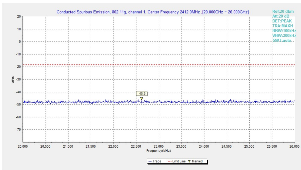
Fig.B.6.1.32 Transmitter Spurious Emission - Conducted (802.11g, Ch1, 20 GHz-26 GHz)
