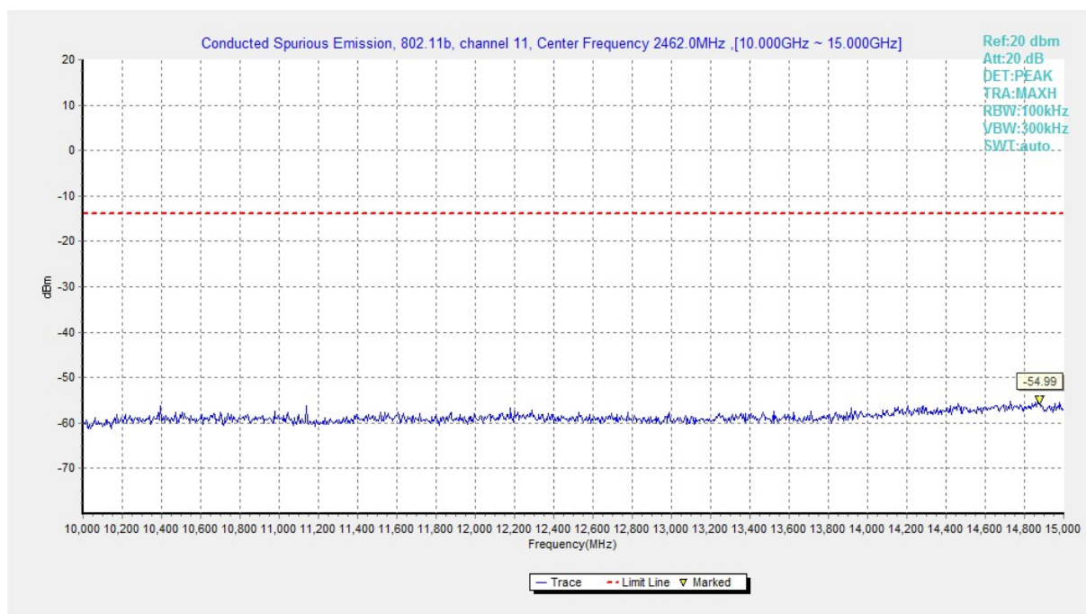
Fig.B.6.1.22 Transmitter Spurious Emission - Conducted (802.11b, Ch11, 10 GHz-15 GHz)
