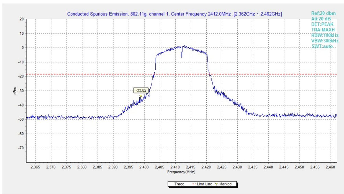
Fig.B.6.1.25 Transmitter Spurious Emission - Conducted (802.11g, Ch1, Center Frequency)
