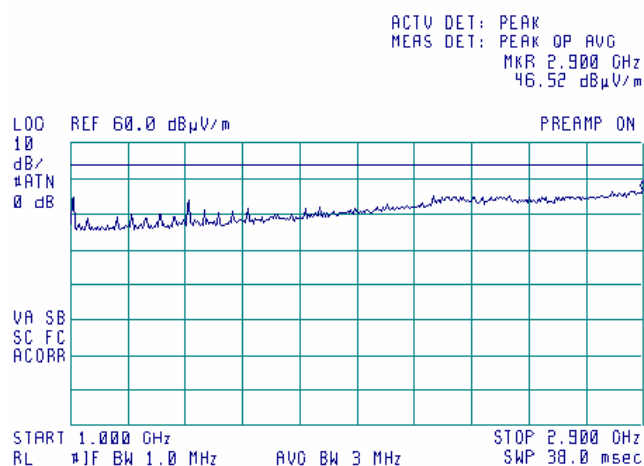
Plot 8.2.4 Radiated emission measurements in 1000- 2900 MHz range, horizontal antenna polarization
