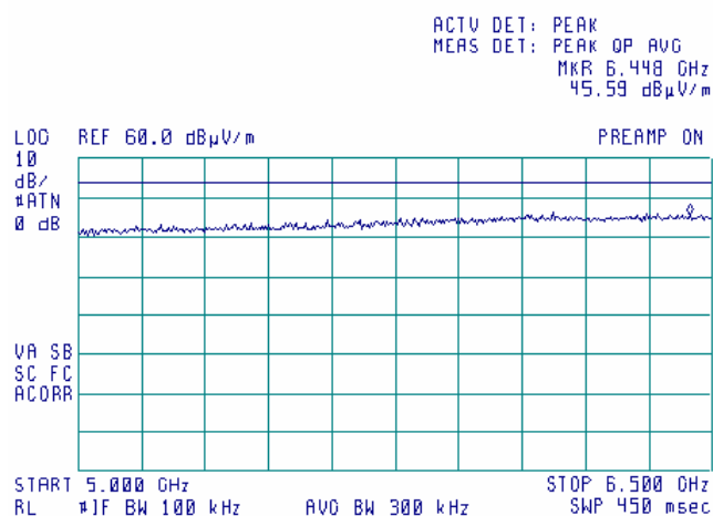
Plot 8.2.8 Radiated emission measurements in 5 - 6.5 GHz range, horizontal antenna polarization
