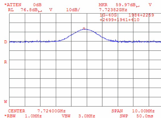
Plot 7.4.35 Radiated emission measurements at the forth harmonic of mid carrier frequency
