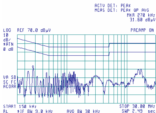
Plot 8.1.4 Conducted emission measurements
