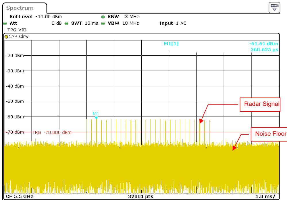
Radar Signal 2
