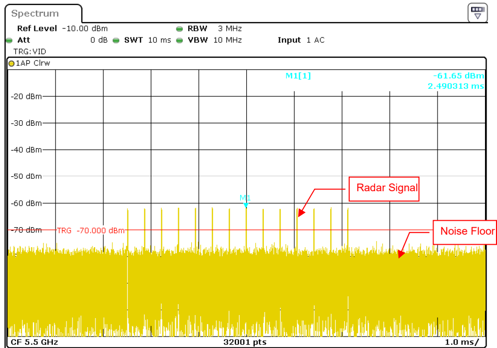
Radar Signal 4
