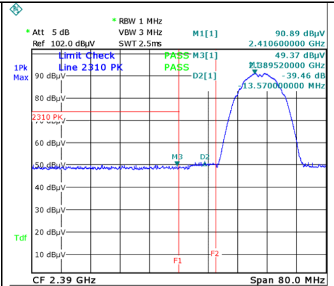
Band Edge, Left Side (Peak) - 802.11b
