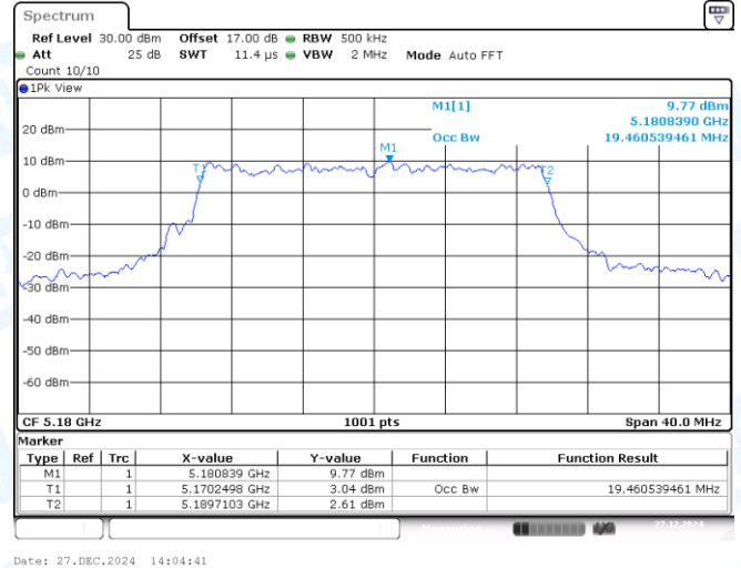
11AX20MIMO-Ant2-5180
