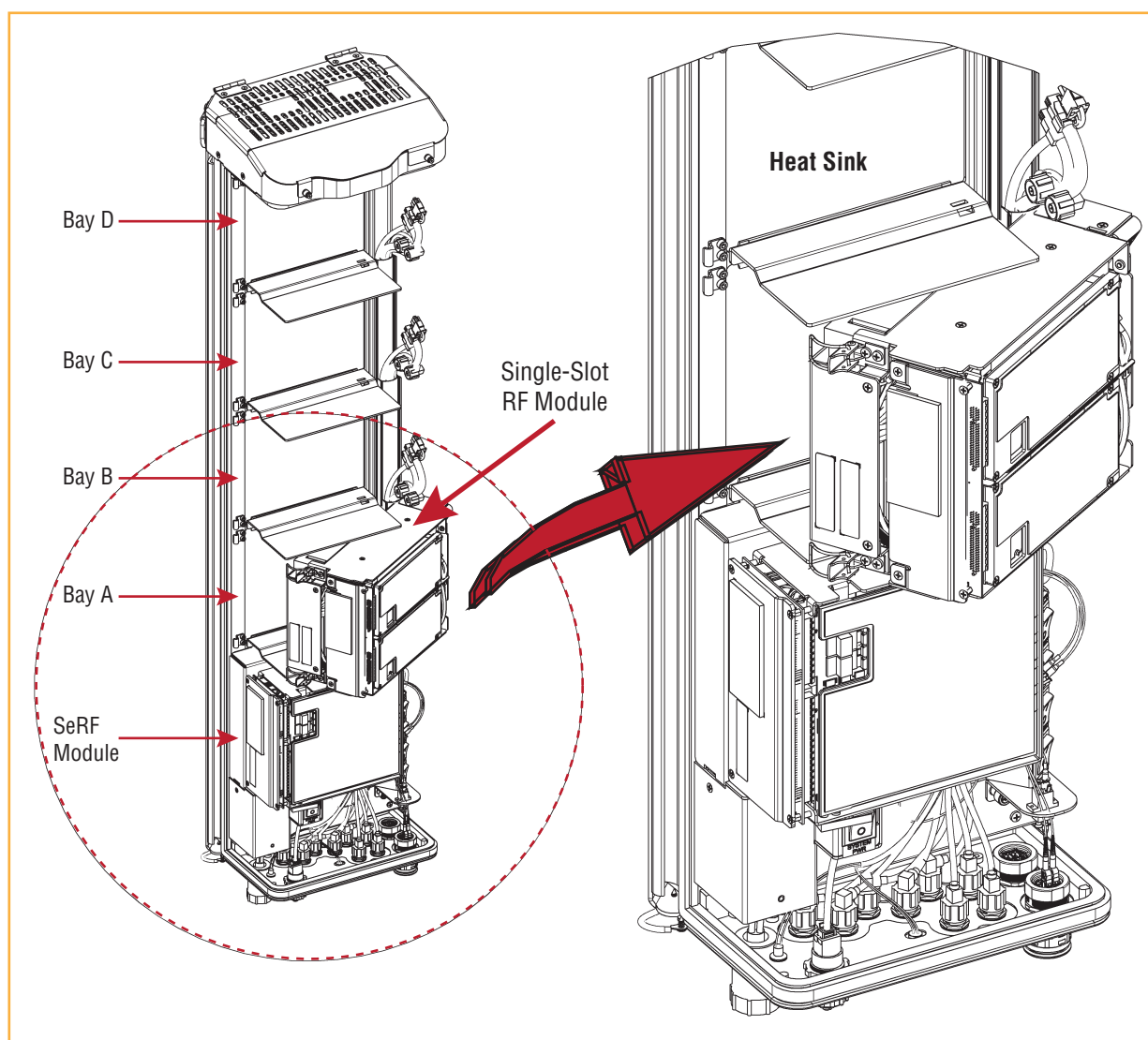
Figure 11. Installing a Single-Bay RF Module
