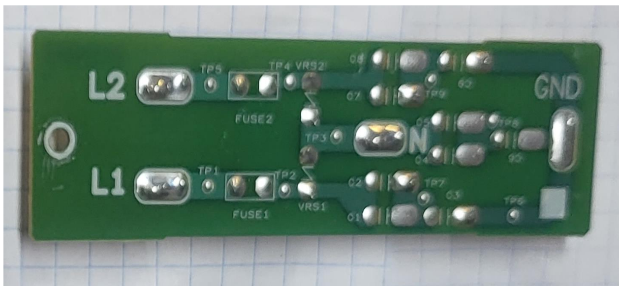
Figure 16. 240V Power Input Filter Bottom Top Side
