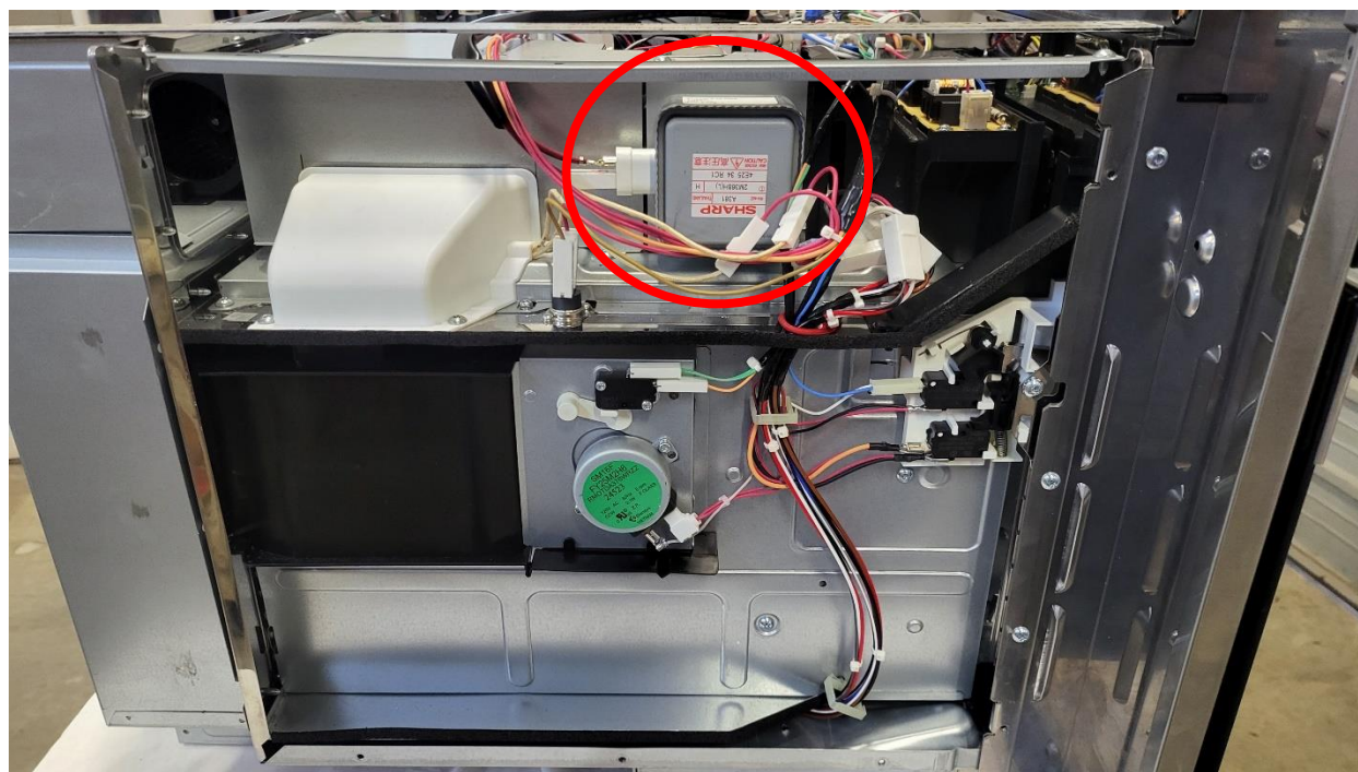
Figure 4. Left Side
