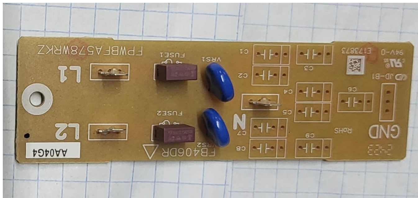
Figure 15. 240V Power Line Filter Top Side
