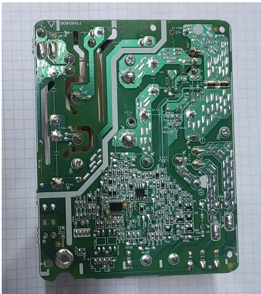
Figure 8. Inverter Bottom Side
