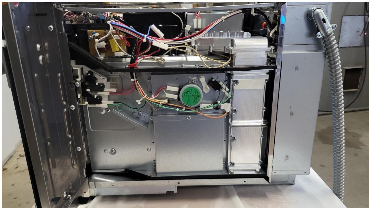
Figure 5. Right Side
