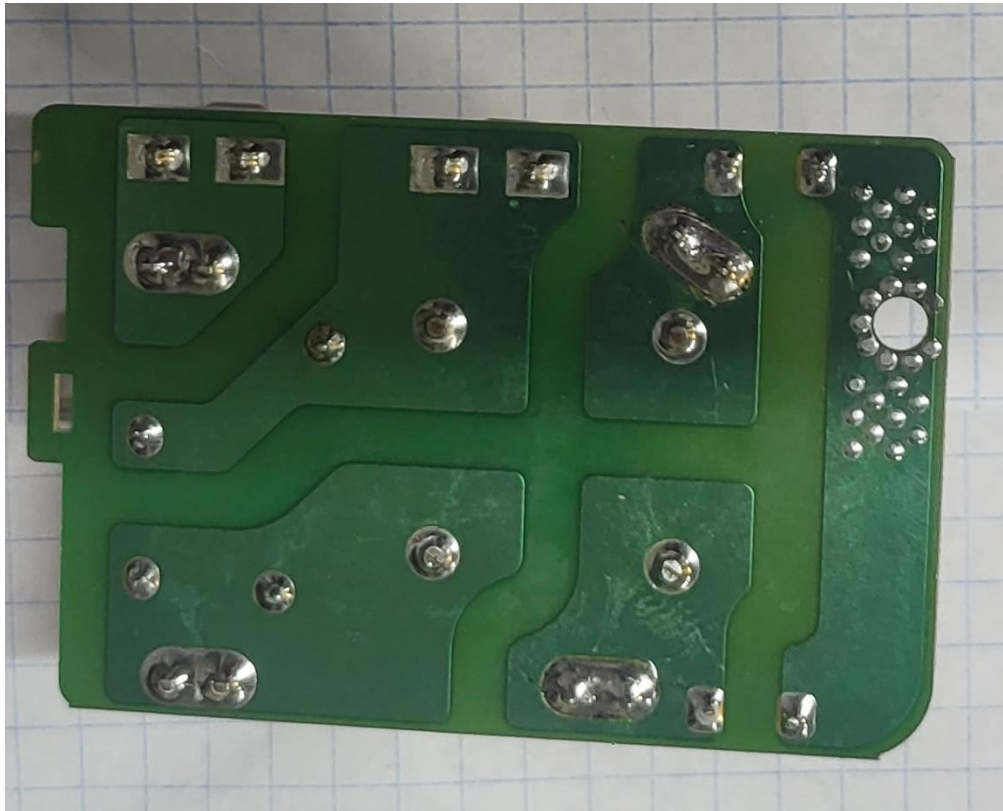
Figure 14. 120V Power Input Filter Bottom Side
