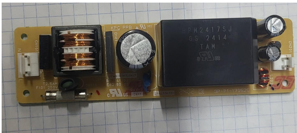
Figure 9. Auxiliary Power Supply Top Side
