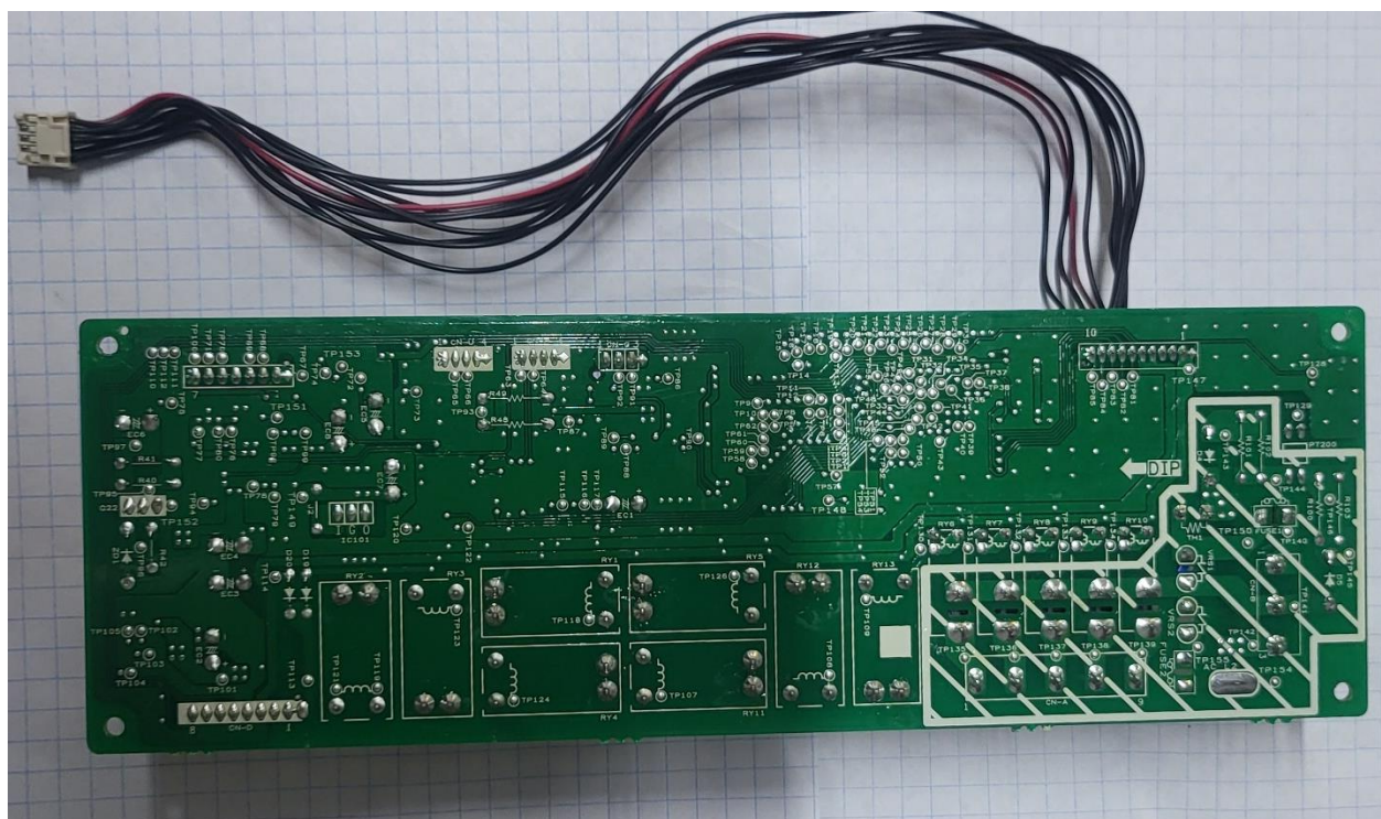
Figure 18. Power Control Board Bottom Side
