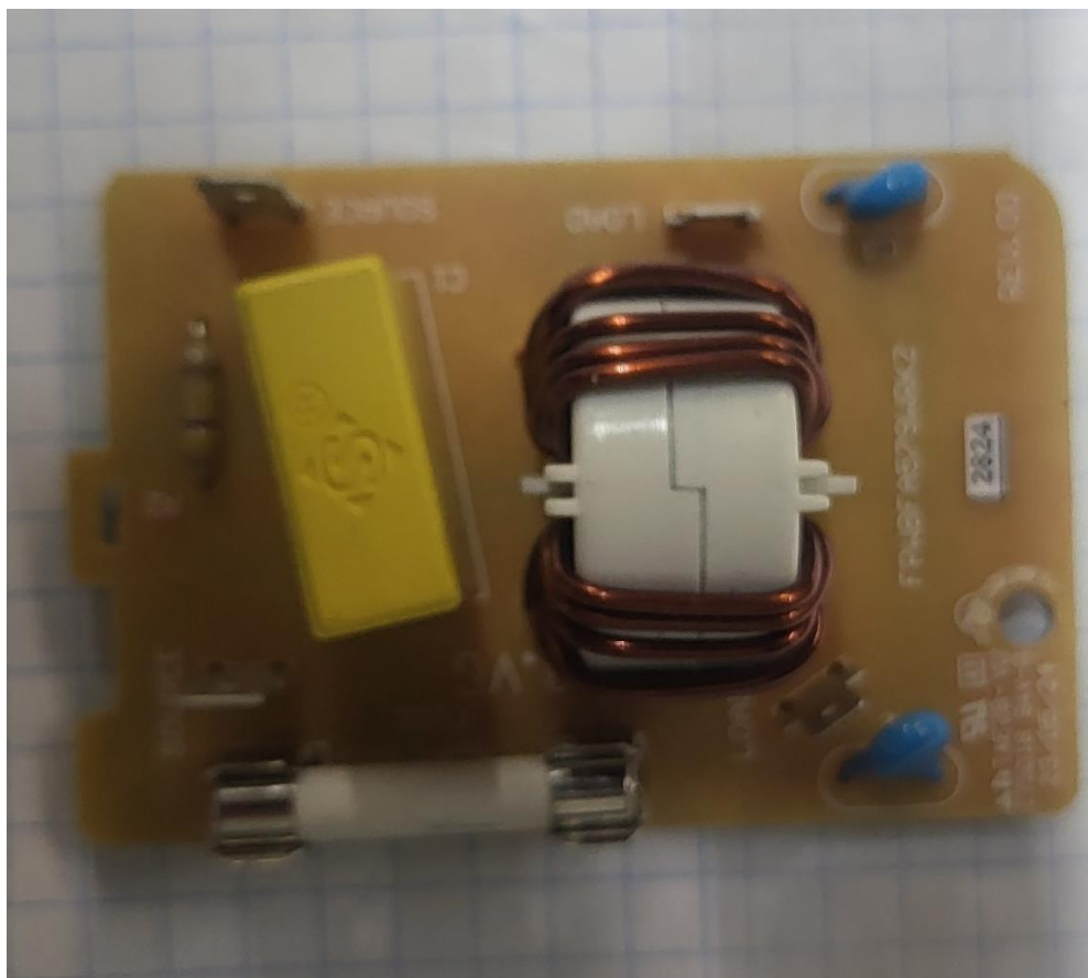
Figure 13. 120V Power Input Filter Top Side
