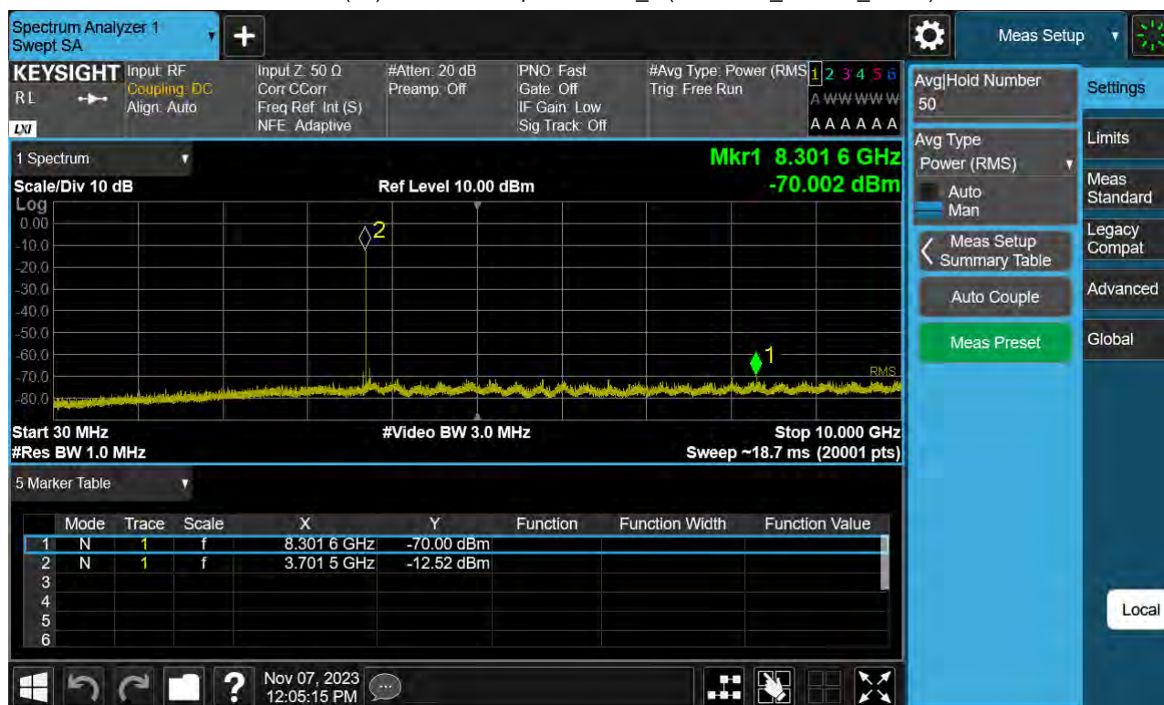
Sub6 n77(78). Conducted Spurious Plot_1 (648334ch_50 MHz_BPSK)
