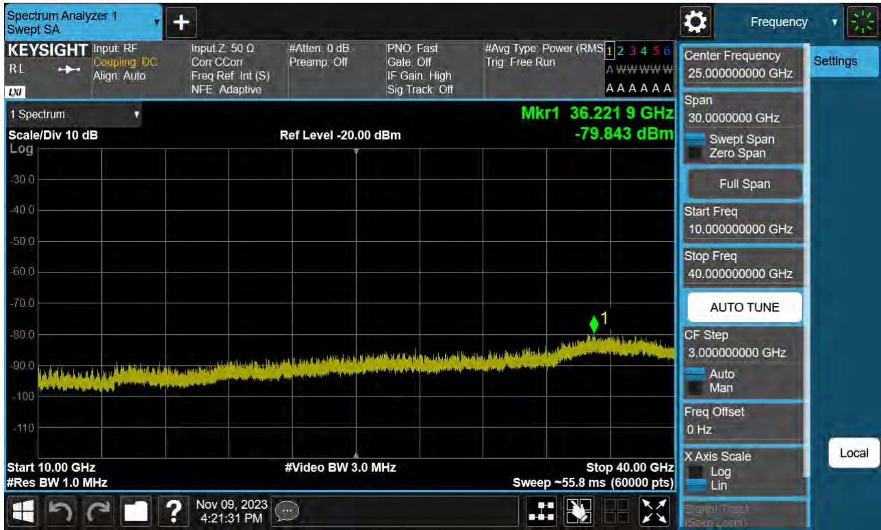
Sub6 n77(78). Conducted Spurious Plot_2 (647500ch_25 MHz_BPSK)
