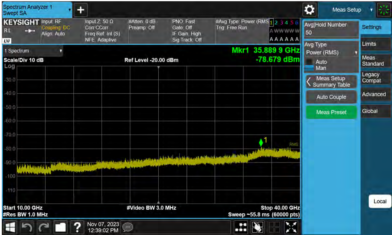
Sub6 n77(78). Conducted Spurious Plot_2 (663000ch_70 MHz_BPSK)
