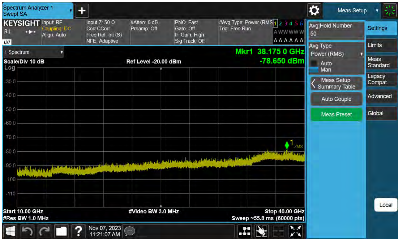
Sub6 n77(78). Conducted Spurious Plot_2 (664832ch_15 MHz_BPSK)
