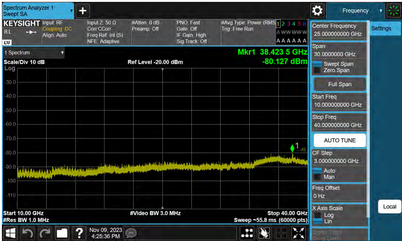
Sub6 n77(78). Conducted Spurious Plot_2 (656000ch_25 MHz_BPSK)
