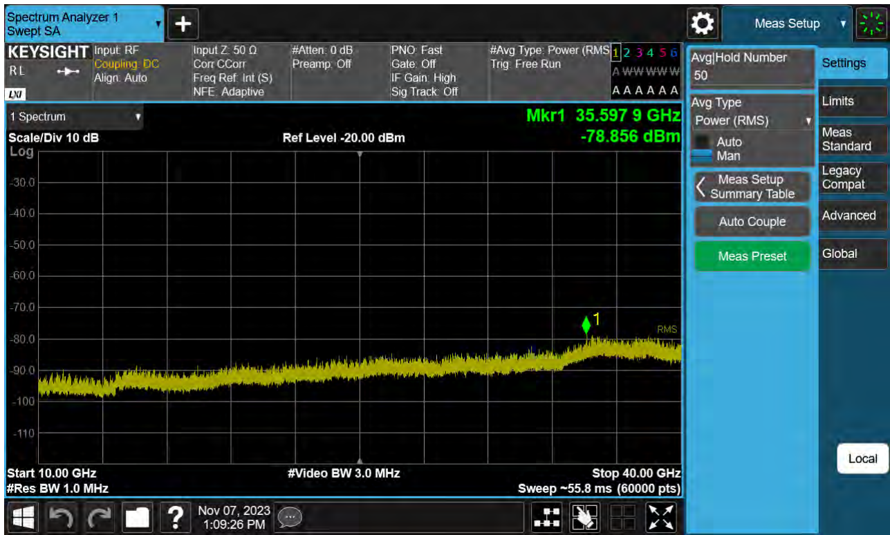
Sub6 n77(78). Conducted Spurious Plot_2 (650000ch_100 MHz_BPSK)
