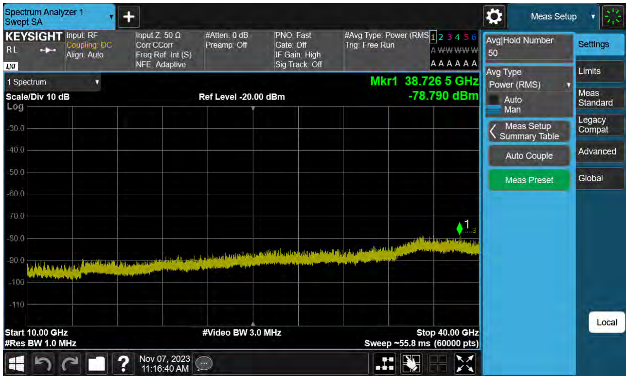
Sub6 n77(78). Conducted Spurious Plot_2 (656000ch_15 MHz_BPSK)
