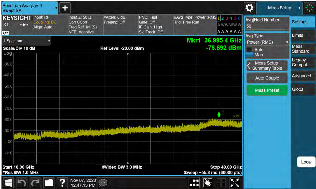
Sub6 n77(78). Conducted Spurious Plot_2 (656000ch_80 MHz_BPSK)
