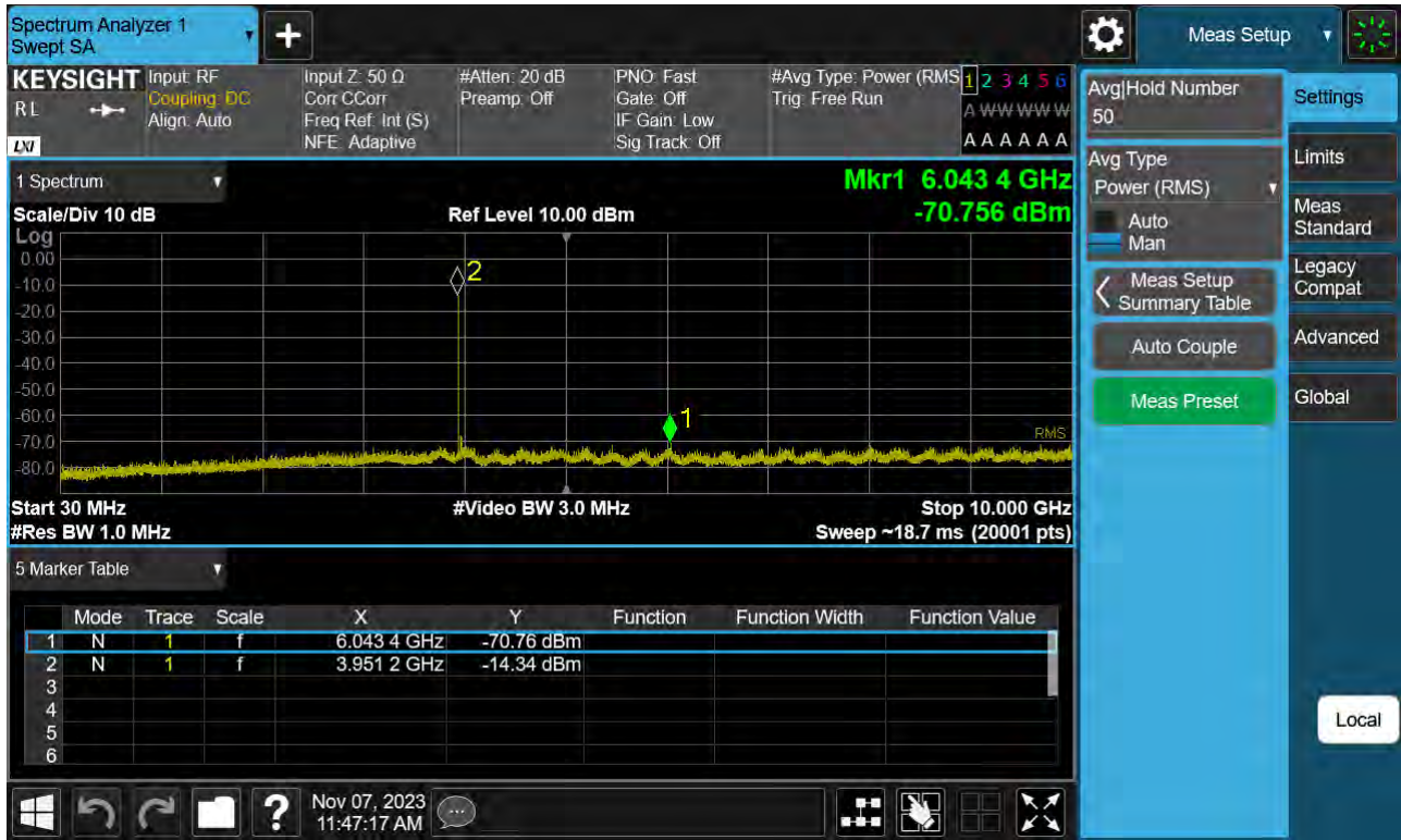
Sub6 n77(78). Conducted Spurious Plot_1 (664332ch_30 MHz_BPSK)
