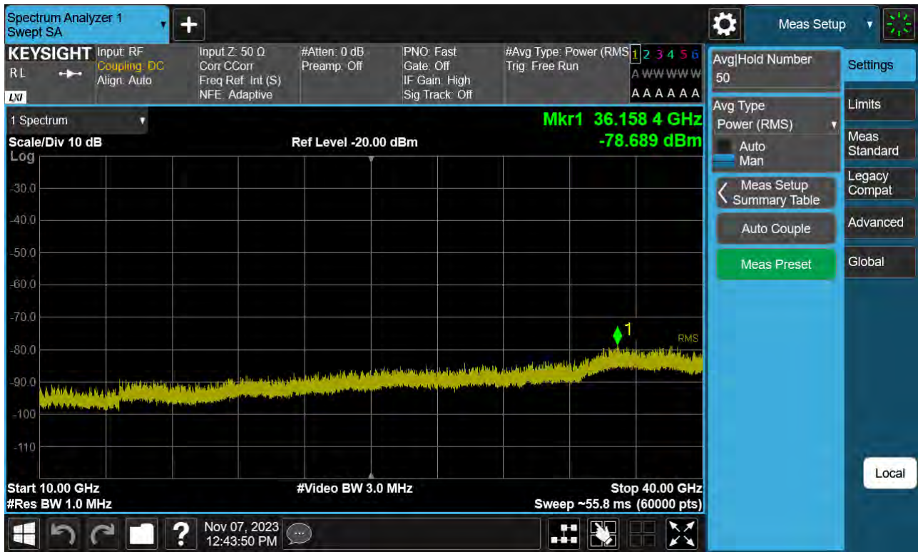
Sub6 n77(78). Conducted Spurious Plot_2 (649334ch_80 MHz_BPSK)
