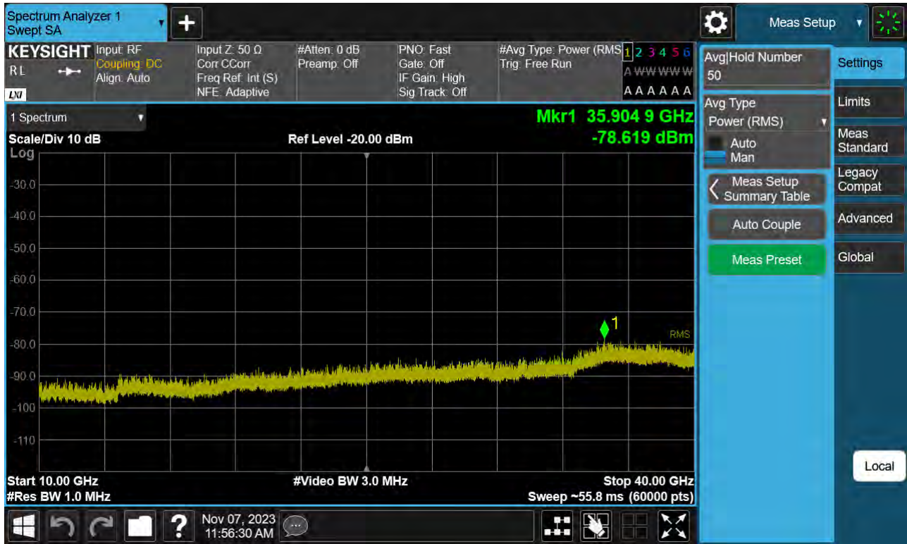
Sub6 n77(78). Conducted Spurious Plot_2 (656000ch_40 MHz_BPSK)
