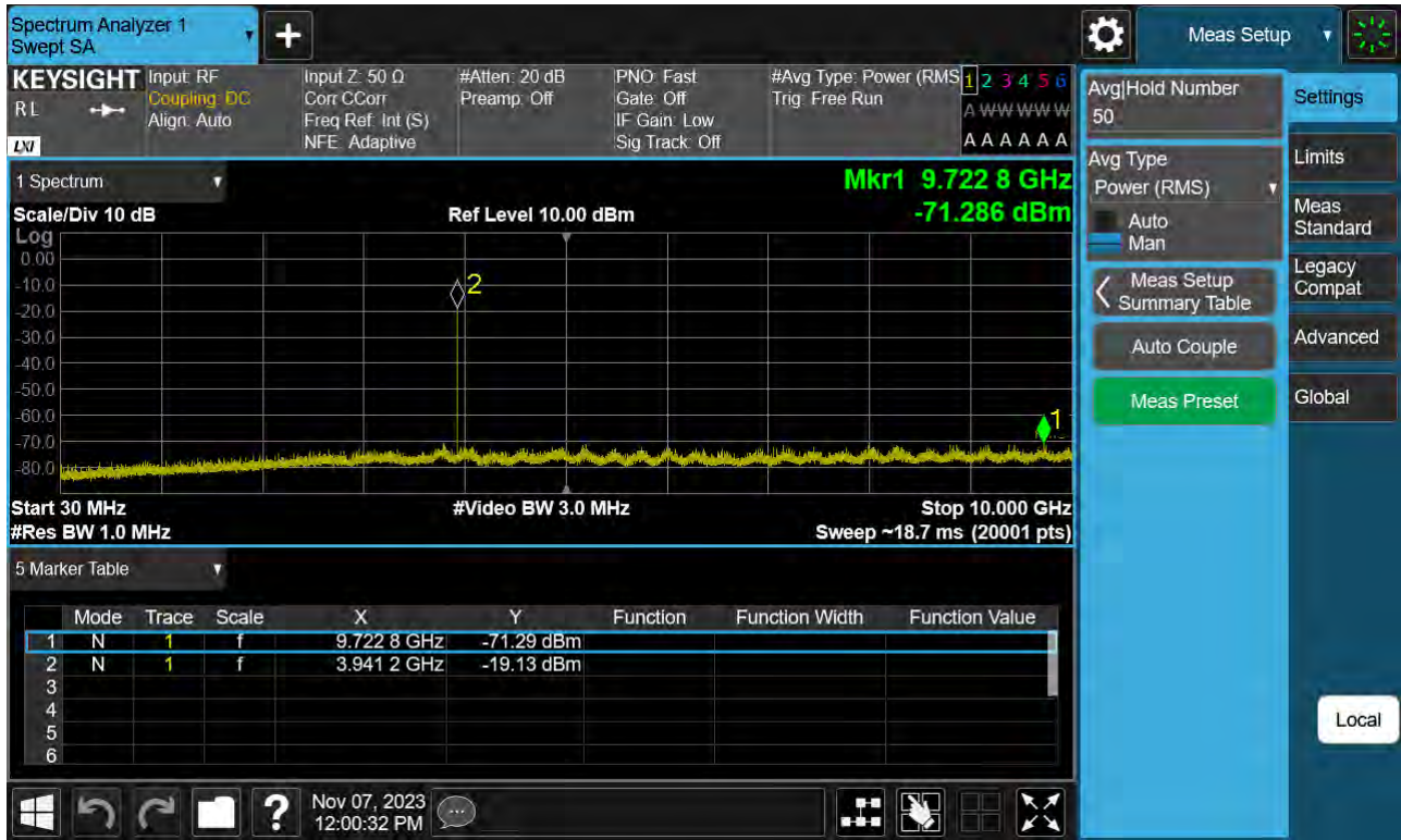
Sub6 n77(78). Conducted Spurious Plot_1 (664000ch_40 MHz_BPSK)
