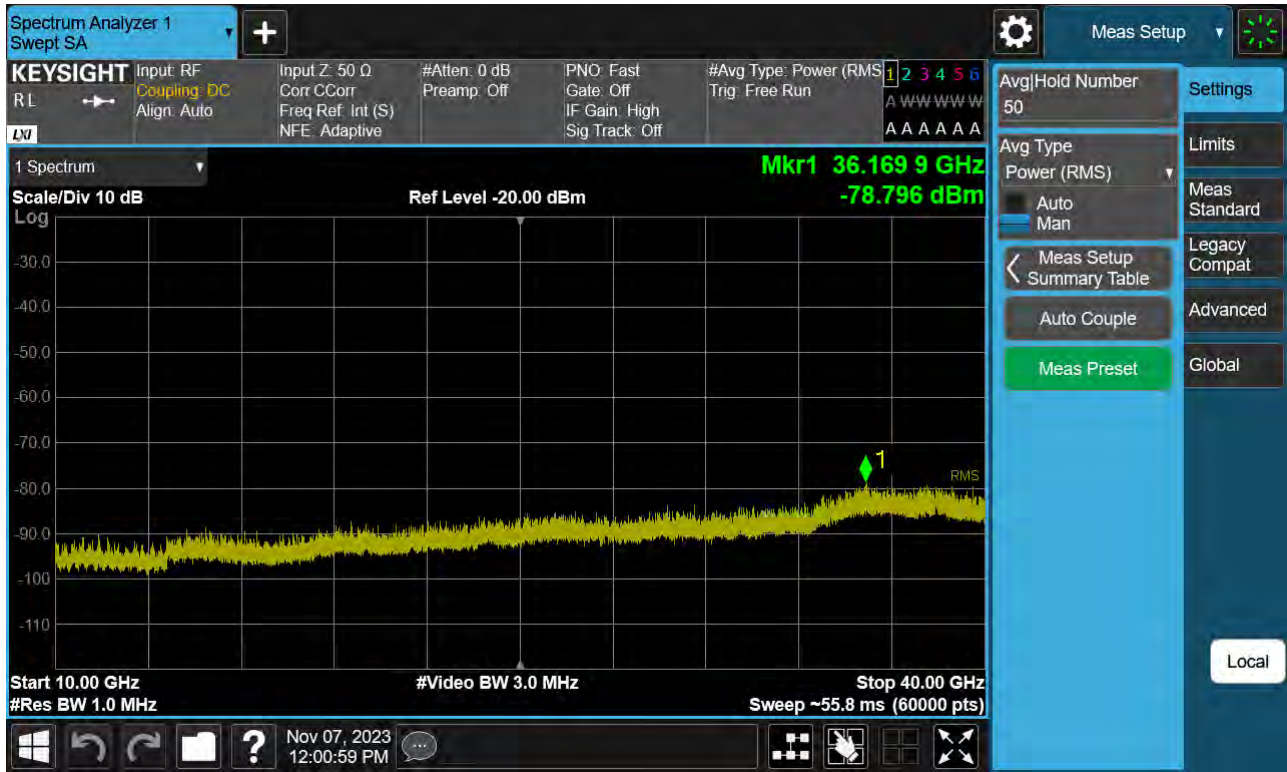
Sub6 n77(78). Conducted Spurious Plot_2 (664000ch_40 MHz_BPSK)
