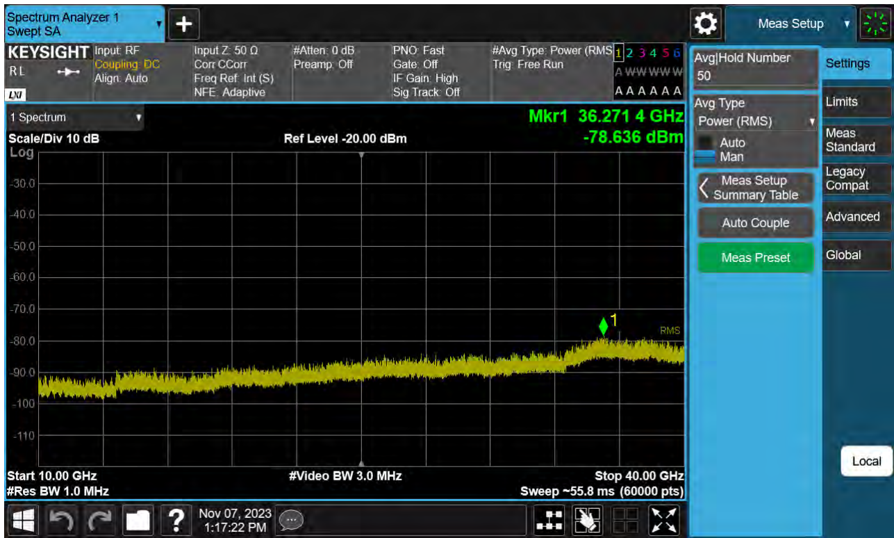
Sub6 n77(78). Conducted Spurious Plot_2 (662000ch_100 MHz_BPSK)
