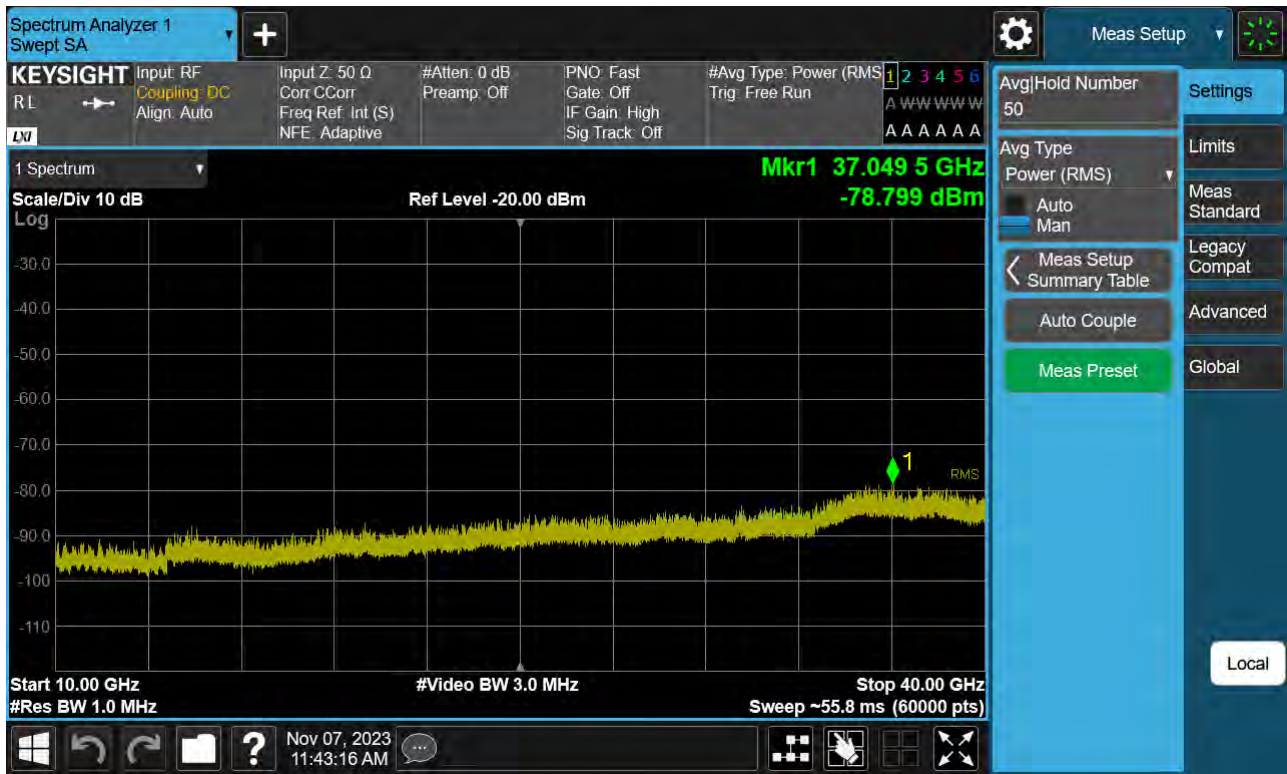
Sub6 n77(78). Conducted Spurious Plot_2 (656000ch_30 MHz_BPSK)
