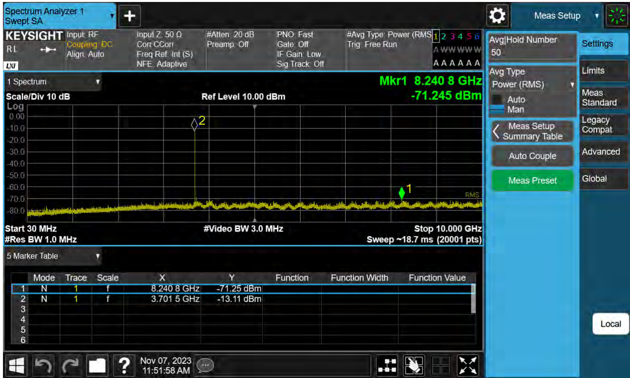
Sub6 n77(78). Conducted Spurious Plot_1 (648000ch_40 MHz_BPSK)
