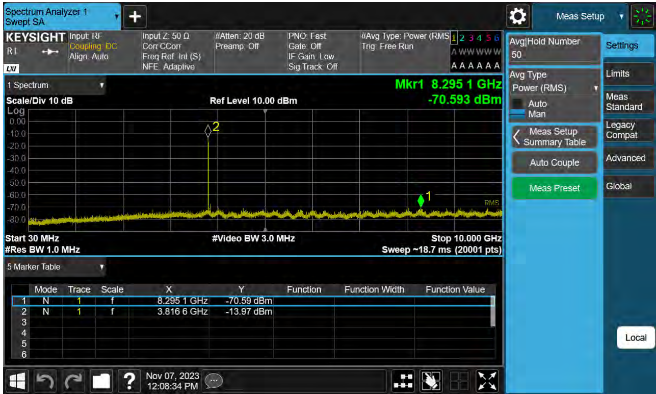
Sub6 n77(78). Conducted Spurious Plot_1 (656000ch_50 MHz_BPSK)
