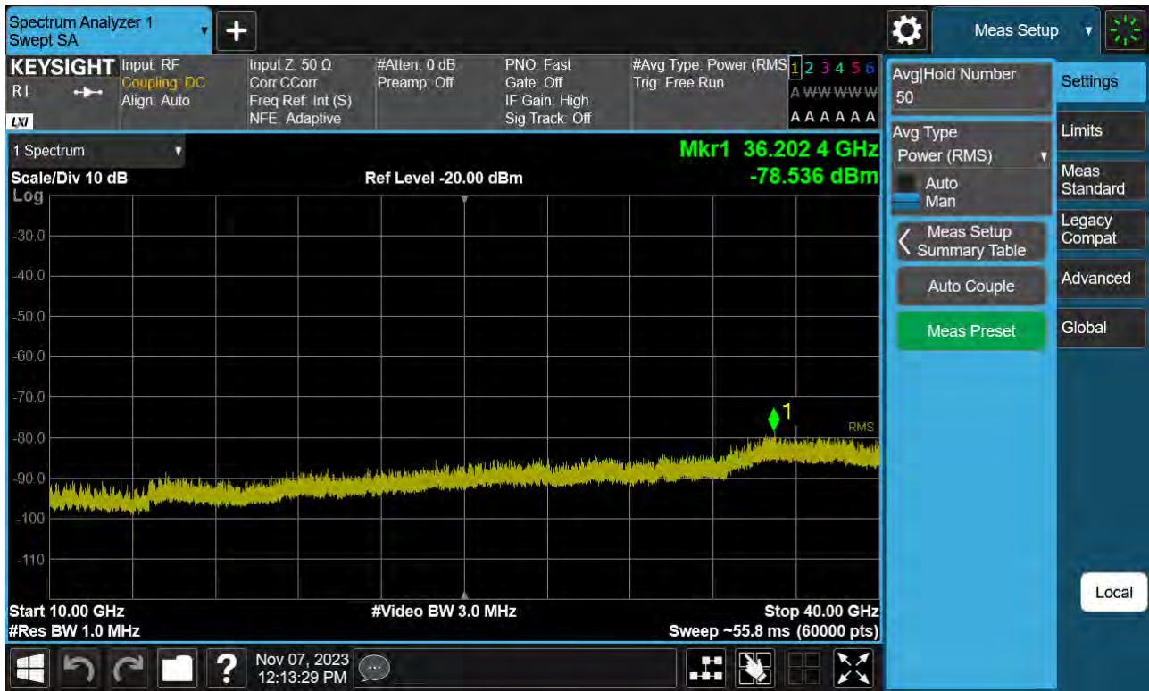
Sub6 n77(78). Conducted Spurious Plot_2 (663666ch_50 MHz_BPSK)
