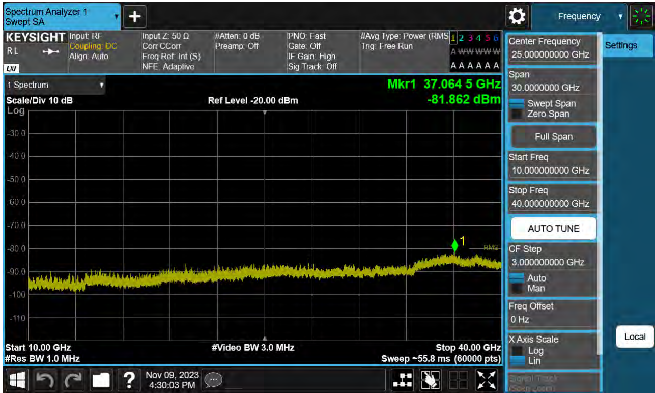
Sub6 n77(78). Conducted Spurious Plot_2 (664500ch_25 MHz_BPSK)
