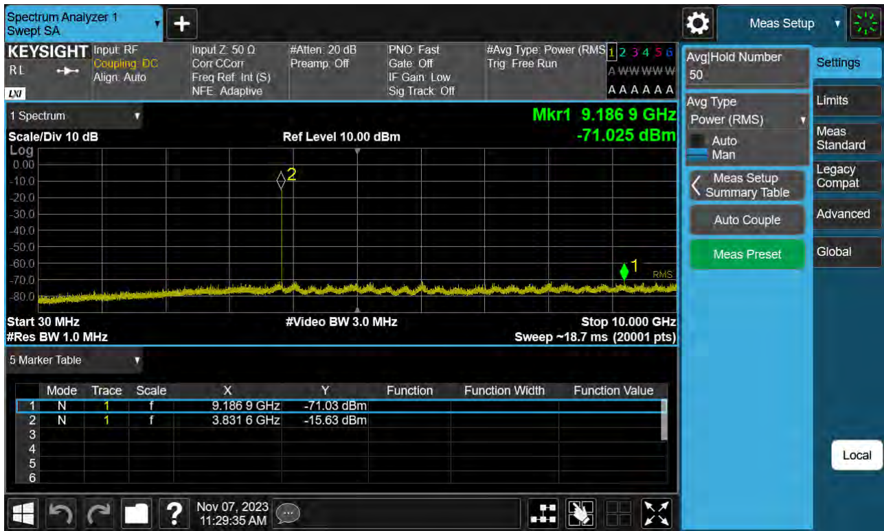
Sub6 n77(78). Conducted Spurious Plot_1 (656000ch_20 MHz_BPSK)
