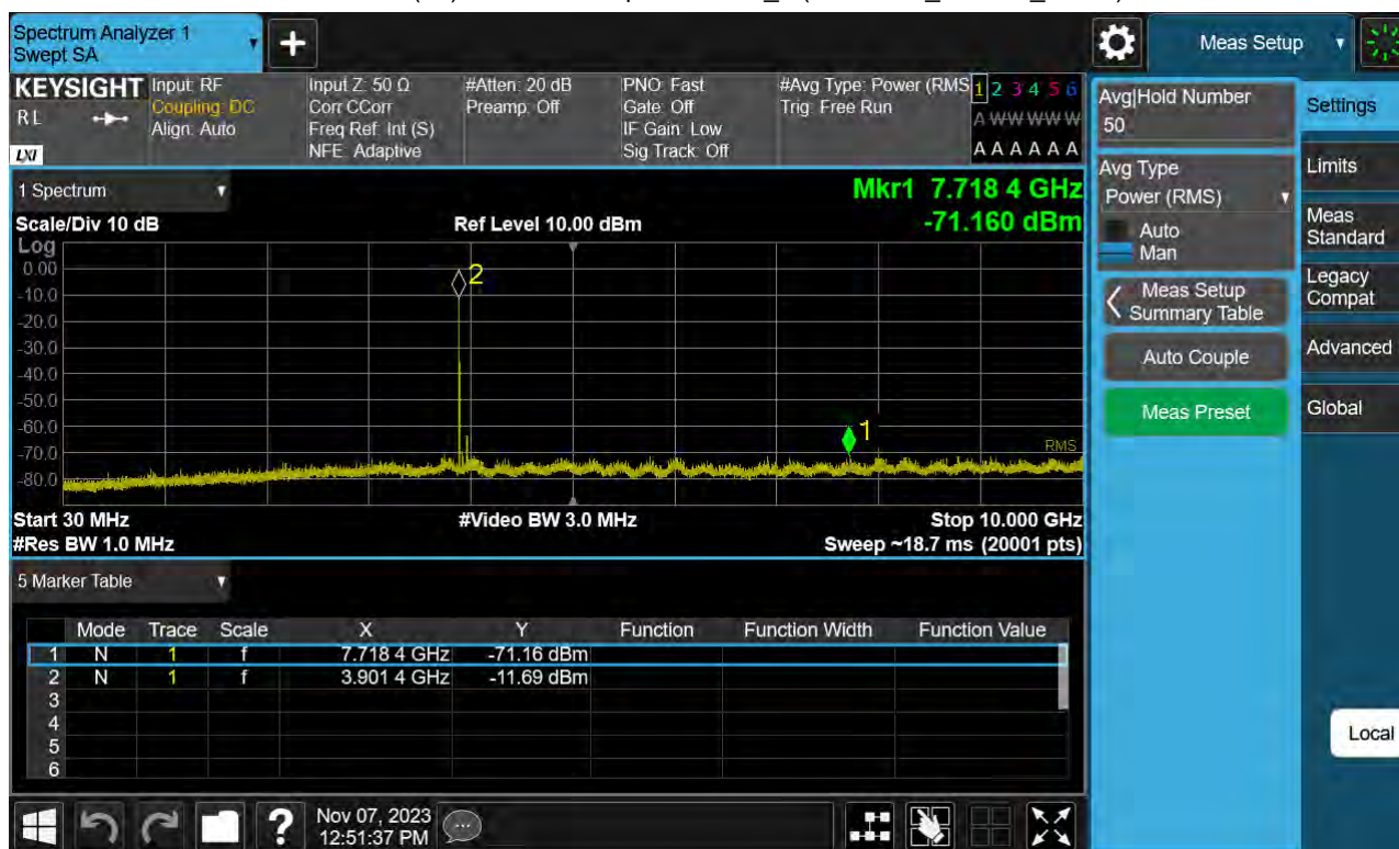
Sub6 n77(78). Conducted Spurious Plot_1 (662666ch_80 MHz_BPSK)
