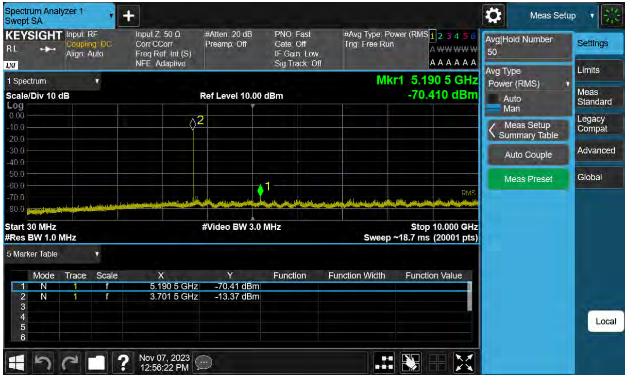
Sub6 n77(78). Conducted Spurious Plot_1 (649668ch_90 MHz_BPSK)
