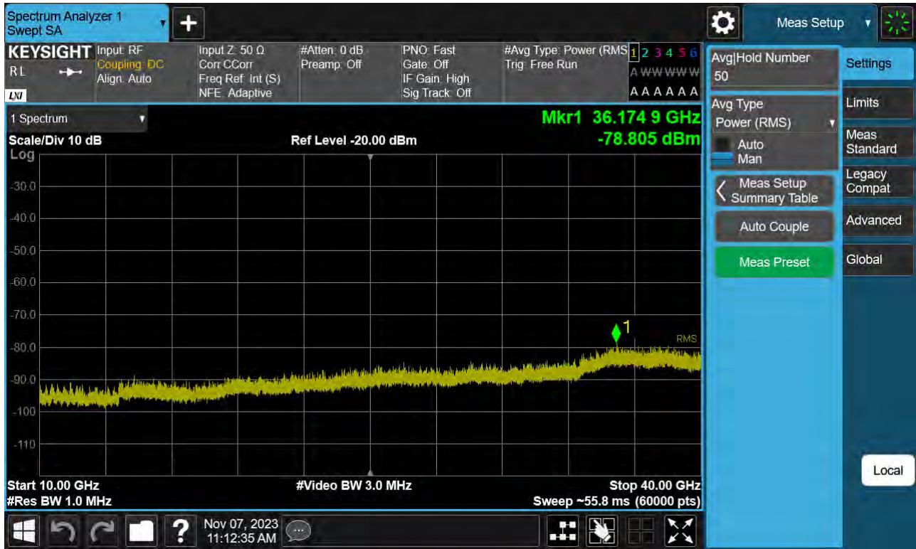
Sub6 n77(78). Conducted Spurious Plot_2 (647168ch_15 MHz_BPSK)
