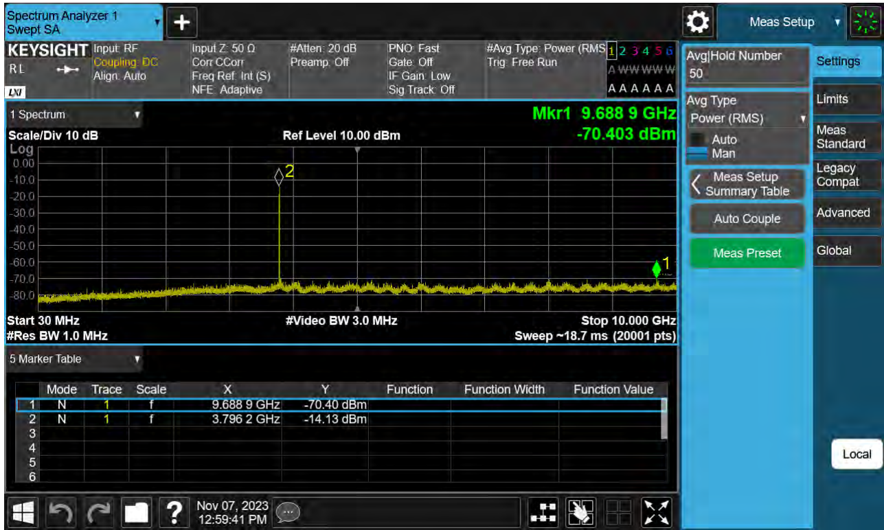
Sub6 n77(78). Conducted Spurious Plot_1 (656000ch_90 MHz_BPSK)
