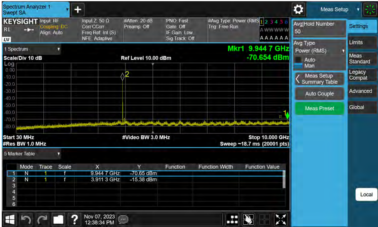
Sub6 n77(78). Conducted Spurious Plot_1 (663000ch_70 MHz_BPSK)
