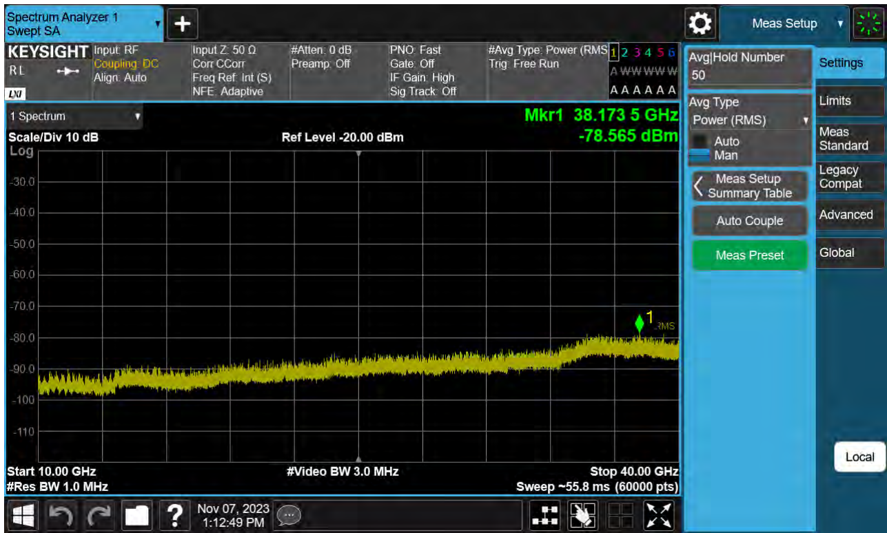
Sub6 n77(78). Conducted Spurious Plot_2 (656000ch_100 MHz_BPSK)
