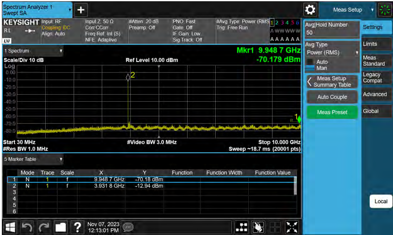
Sub6 n77(78). Conducted Spurious Plot_1 (663666ch_50 MHz_BPSK)
