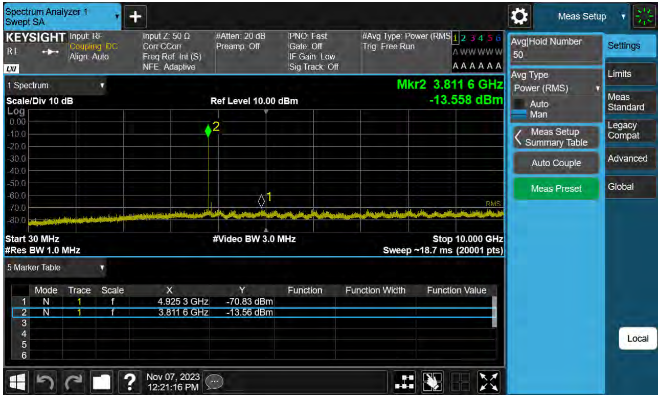
Sub6 n77(78). Conducted Spurious Plot_1 (656000ch_60 MHz_BPSK)
