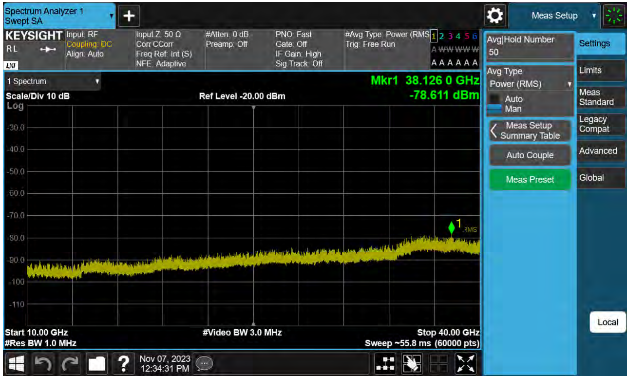
Sub6 n77(78). Conducted Spurious Plot_2 (656000ch_70 MHz_BPSK)
