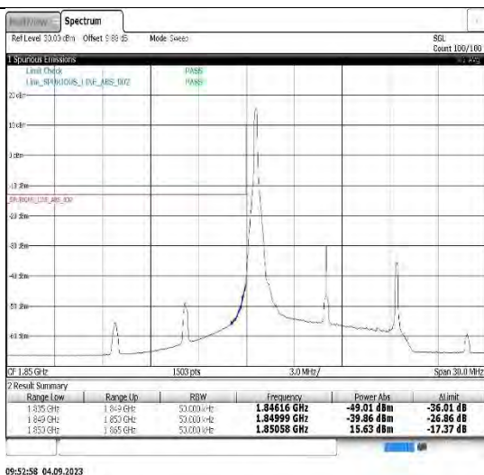
Band2-10MHz-16QAM-18650-50RB#0
