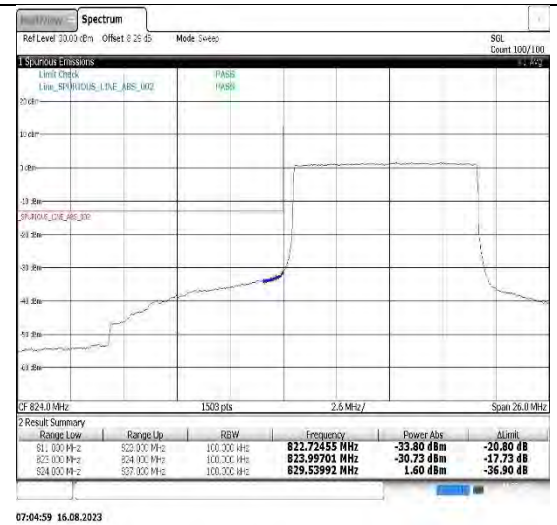
Band5-10MHz-16QAM-20450-50RB#0
