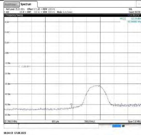
Band14-5MHz-16QAM-23355-1RB#0
