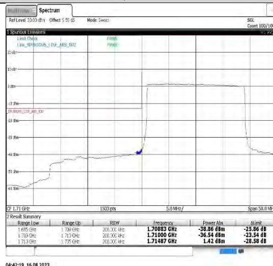
Band4-20MHz-16QAM-20050-100RB#0
