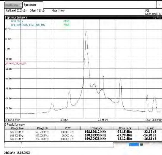
Band12-5MHz-16QAM-23035-1RB#0
