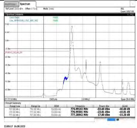
Band13-5MHz-16QAM-23205-1RB#0
