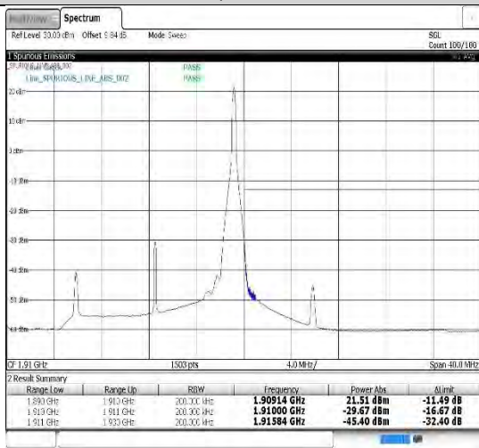
Band2-15MHz-QPSK-19125-1RB#74
