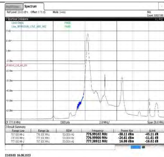
Band14-5MHz-QPSK-23305-1RB#24
