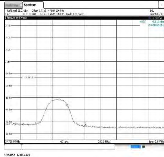
Band14-5MHz-16QAM-23355-25RB#0
