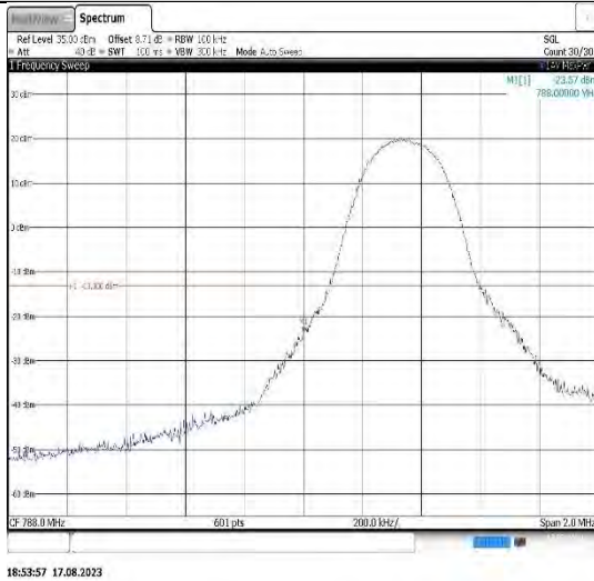
Band14-5MHz-16QAM-23305-25RB#0
