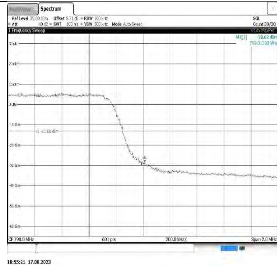
Band14-5MHz-16QAM-23305-1RB#24
