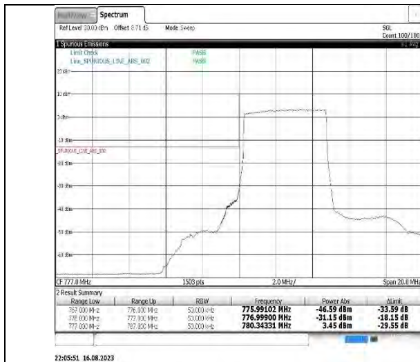
Band13-5MHz-16QAM-23205-25RB#0
