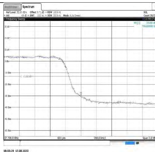
Band14-10MHz-QPSK-23330-1RB#49
