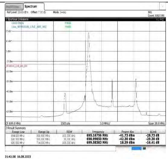
Band12-10MHz-16QAM-23060-1RB#0
