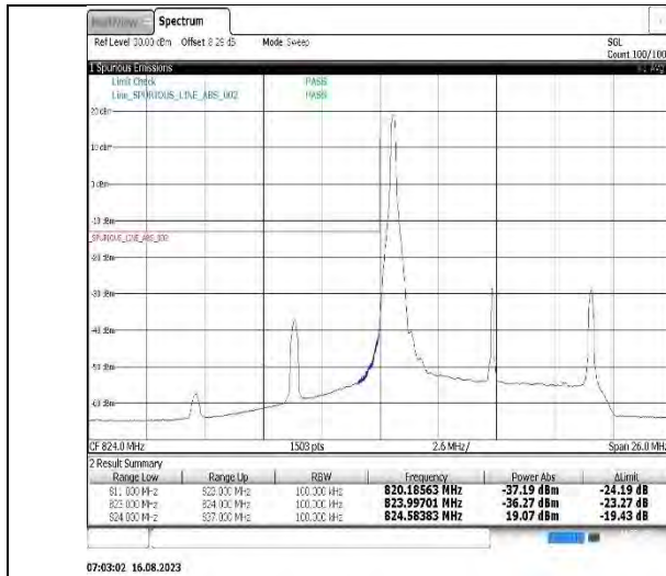
Band5-10MHz-16QAM-20450-1RB#0
