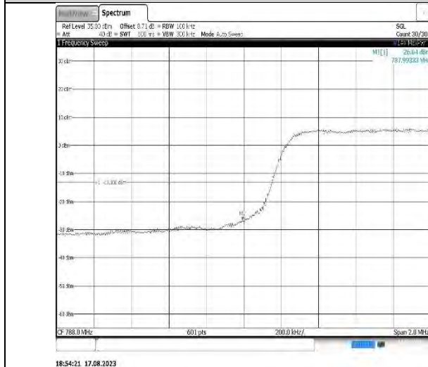
Band14-5MHz-QPSK-23355-1RB#24
