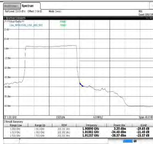
Band2-15MHz-QPSK-19125-75RB#0
