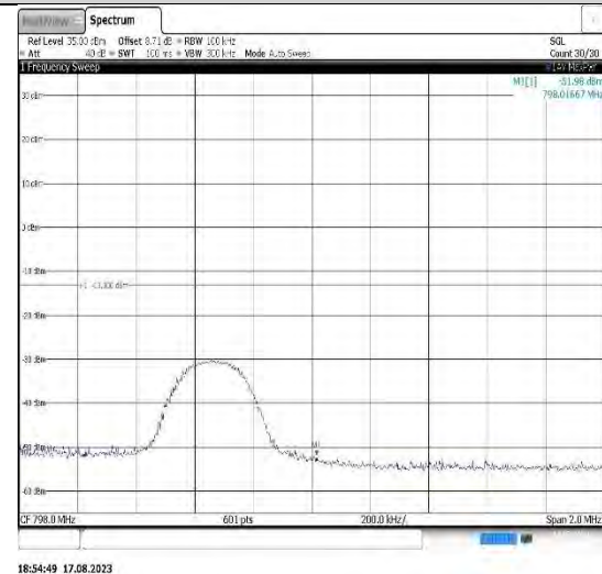
Band14-5MHz-QPSK-23355-25RB#0
