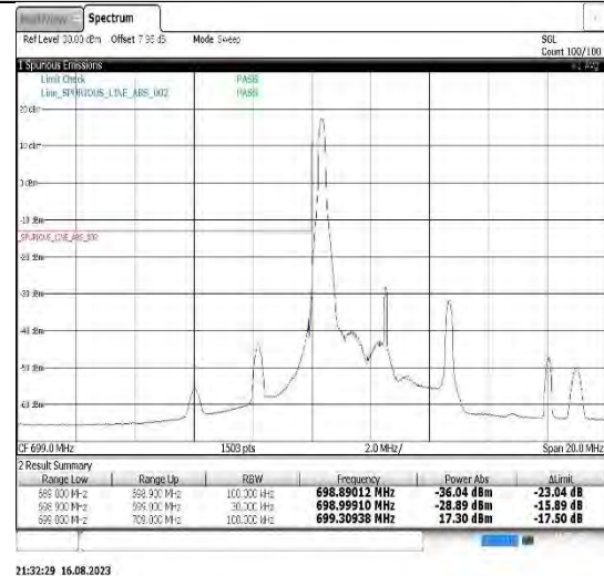
Band12-10MHz-QPSK-23060-1RB#0
