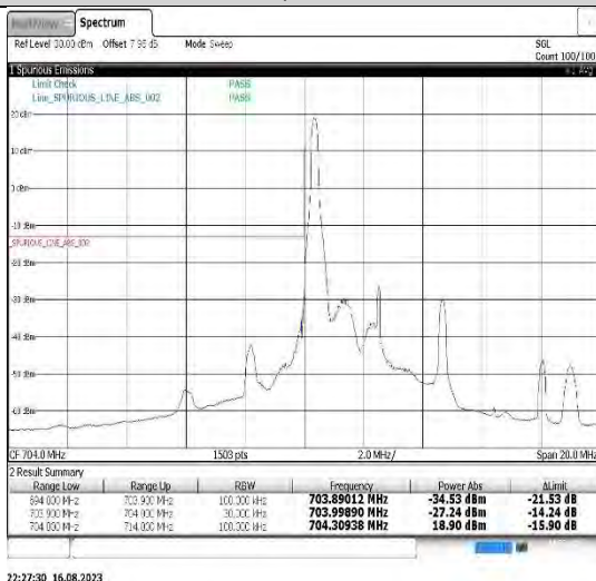
Band17-5MHz-16QAM-23755-1RB#0
