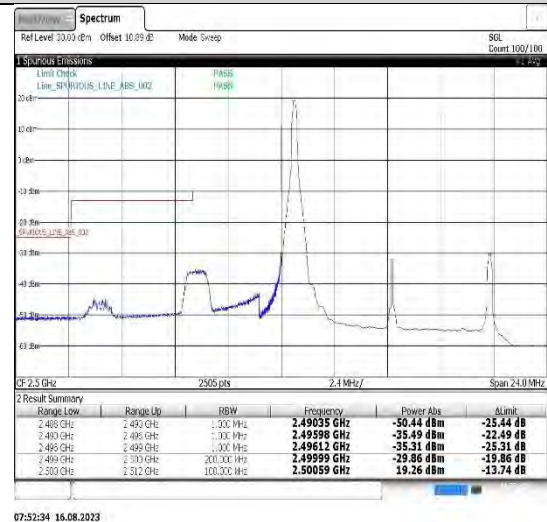
Band7-10MHz-QPSK-21400-1RB#49
