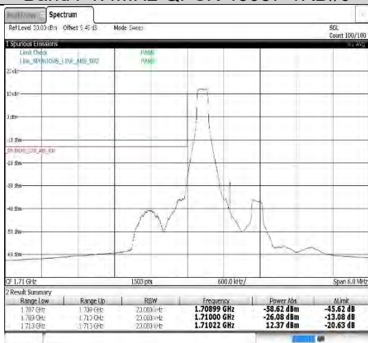
Band4-1.4MHz-QPSK-19957-1RB#0
