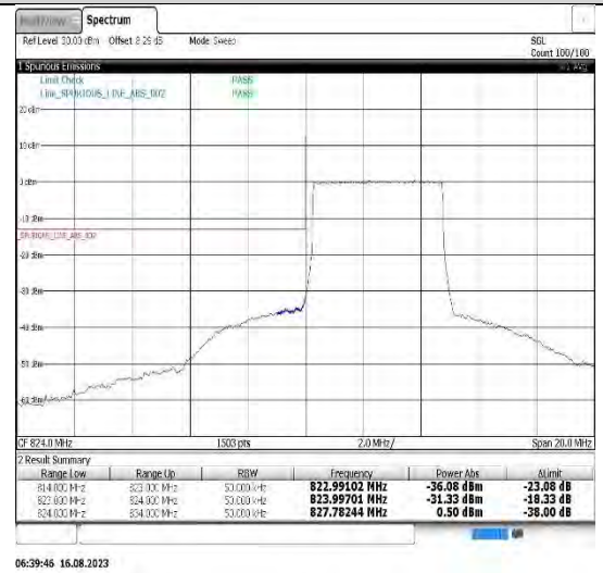
Band5-5MHz-16QAM-20625-25RB#0
