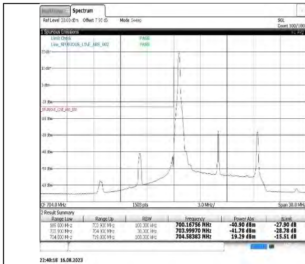
Band17-10MHz-QPSK-23800-1RB#49
