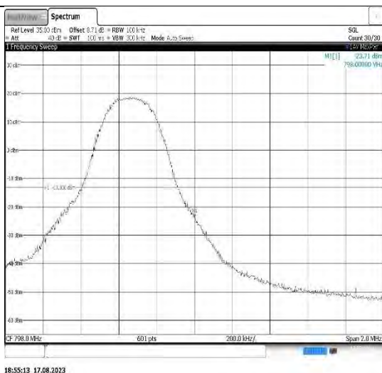
Band14-10MHz-QPSK-23330-1RB#0
