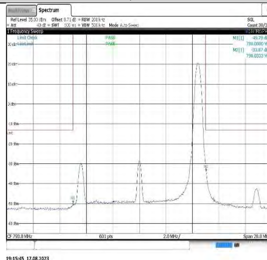
Band14-10MHz-16QAM-23330-1RB#0
