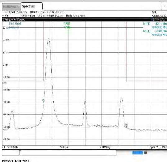
Band14-10MHz-QPSK-23330-50RB#0
