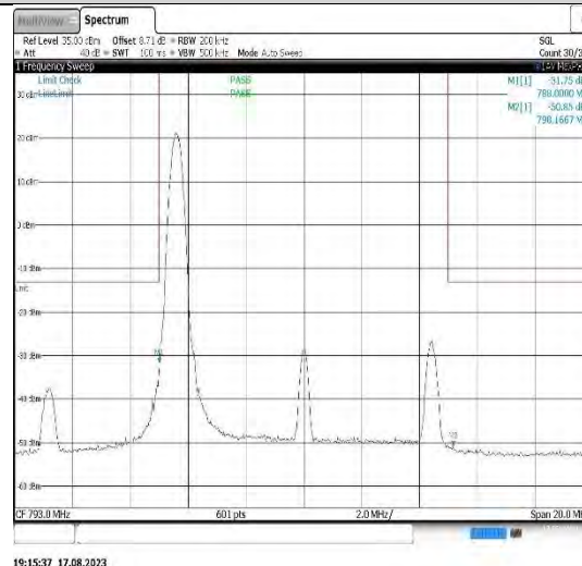
Band14-10MHz-16QAM-23330-50RB#0
