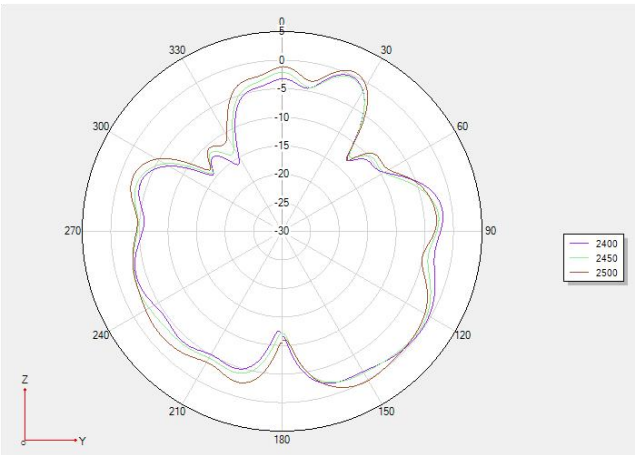
Phi 90 2Dgraph
