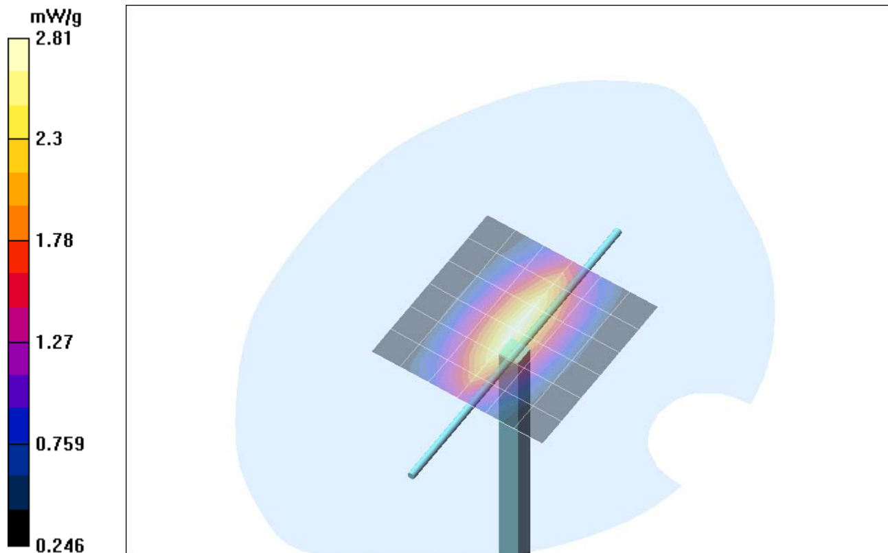
Fig. 14: Validation measurement 835MHz Body (November 25, 2004), coarse grid. Ambient Temperature: 22.0° C, Liquid Temperature: 21.0° C.
