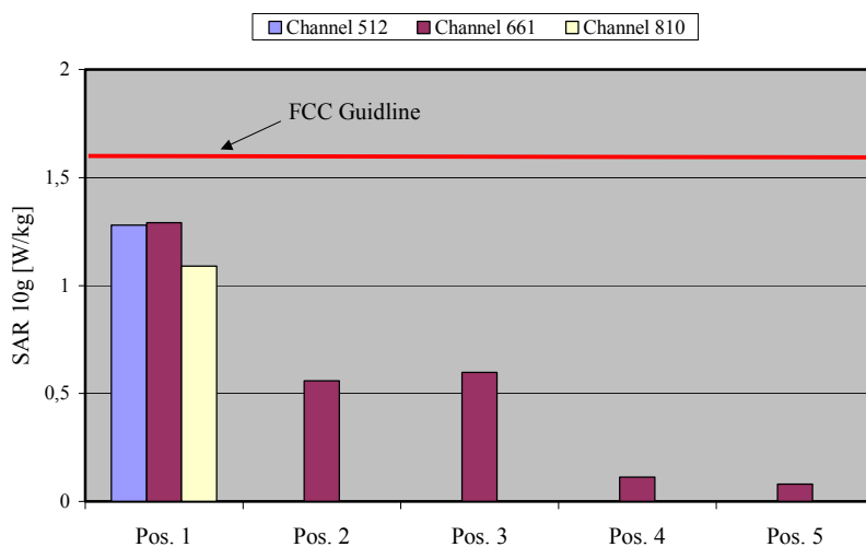
Fig. 11: The measured SAR values for the Option Fusion Quad Band Card in combination with a DELL Latitude D505 Notebook for GPRS 1900 in comparison to the FCC exposure limit.
