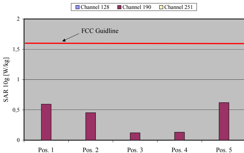
Fig. 9: The measured SAR values for the Option Fusion Quad Band Card in combination with a Packard Bell Easy Note Notebook for GPRS 850 in comparison to the FCC exposure limit.
