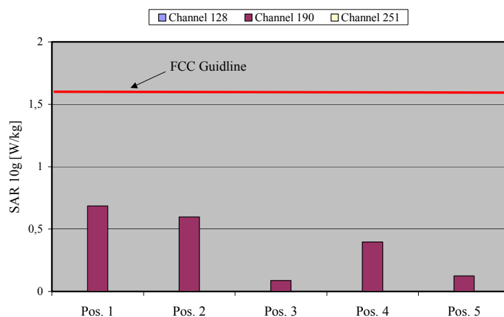
Fig. 10: The measured SAR values for the Option Fusion Quad Band Card in combination with a Acer Aspire 2020 Notebook for GPRS 850 in comparison to the FCC exposure limit.
