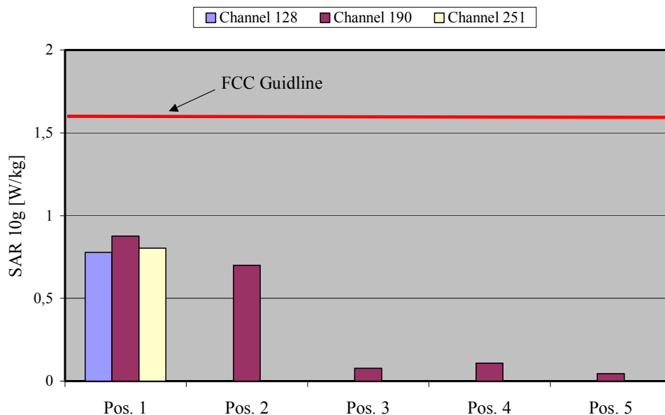
Fig. 8: The measured SAR values for the Option Fusion Quad Band Card in combination with a DELL Latitude D505 Notebook for GPRS 850 in comparison to the FCC exposure limit.
