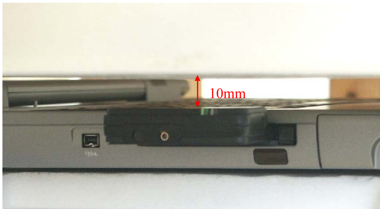
Fig. 21: Position 1 with a DELL Latitude D505 Notebook.
