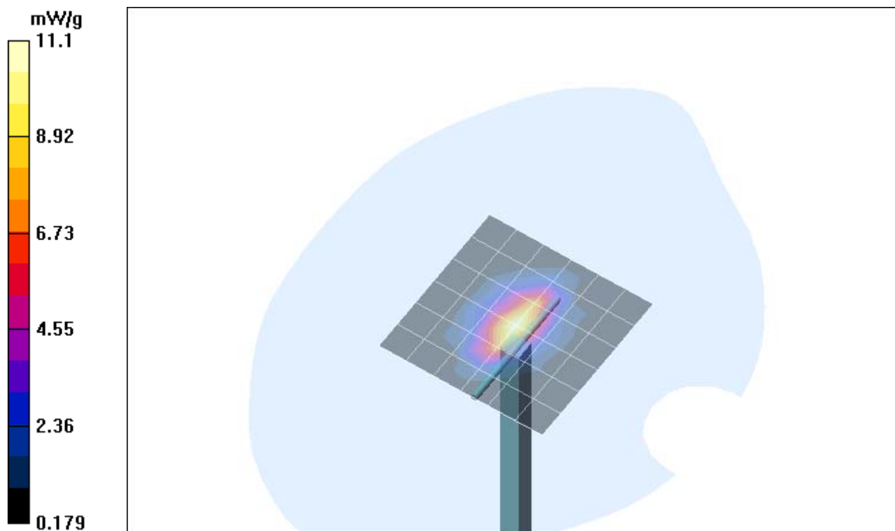
Fig. 16: Validation measurement 1900 MHz Body (November 24, 2004), coarse grid. Ambient Temperature: 22.0° C, Liquid Temperature: 21.0° C.
