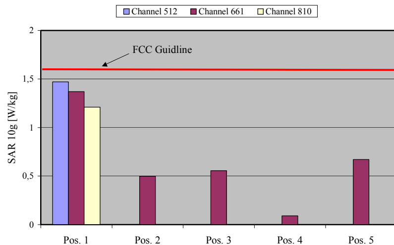
Fig. 13: The measured SAR values for the Option Fusion Quad Band Card in combination with an ACER Aspire 2020 Notebook for GPRS 1900 in comparison to the FCC exposure limit.
