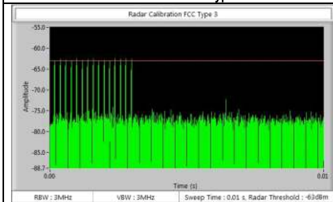
Radar Calibration - Type 3
