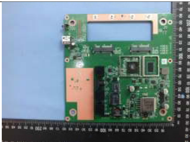
Top View – Mainboard
