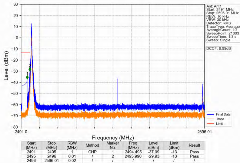
n41_30kHz_SISO_NTNV_100MHz_CP-OFDM_QPSK_2546.01MHz_Edge_1RB_Left
