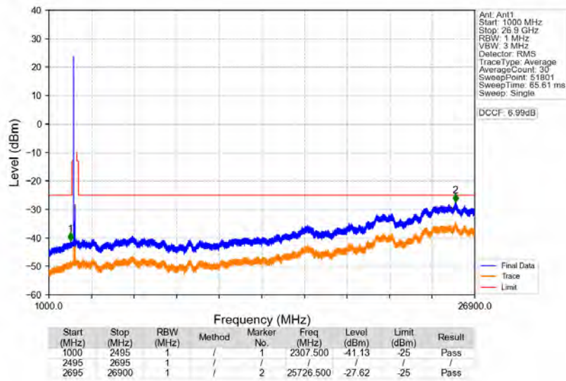
n41_30kHz_SISO_NTNV_100MHz_DFT-s-OFDM_QPSK_2546.01MHz_Edge_1RB_Left
