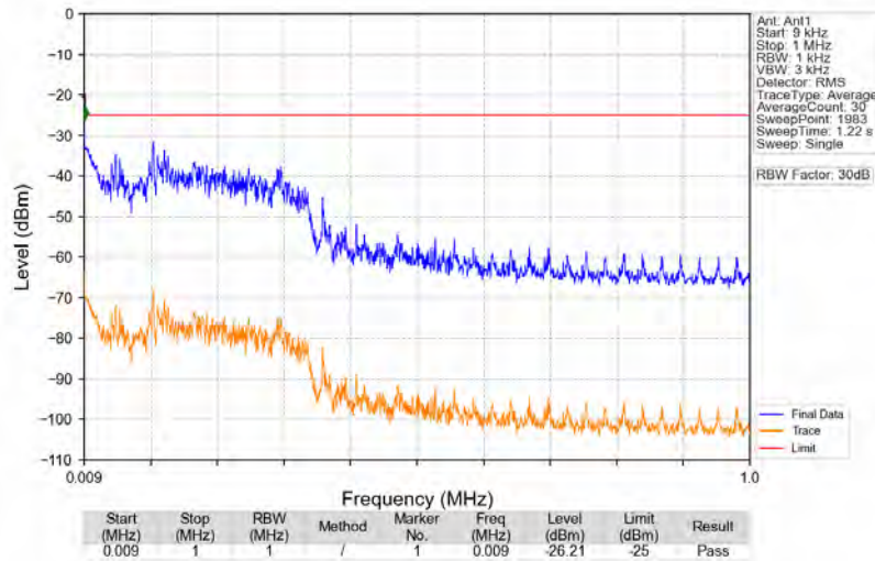
n41_30kHz_SISO_NTNV_100MHz_DFT-s-OFDM_QPSK_2546.01MHz_Edge_1RB_Left
