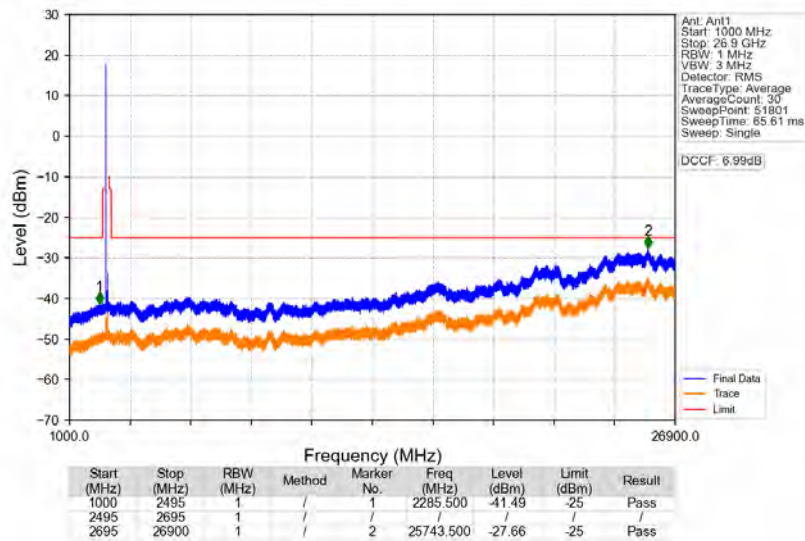
n41_30kHz_SISO_NTNV_90MHz_DFT-s-OFDM_QPSK_2592.99MHz_Edge_1RB_Left
