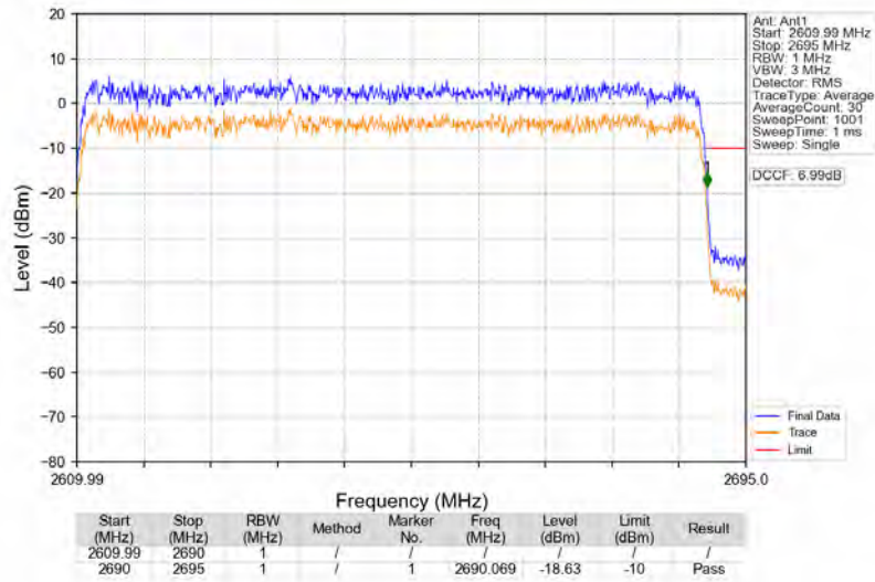
n41_30kHz_SISO_NTNV_80MHz_CP-OFDM_QPSK_2649.99MHz_Outer_Full
