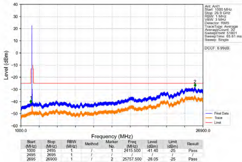
n41_30kHz_SISO_NTNV_80MHz_DFT-s-OFDM_QPSK_2592.99MHz_Edge_1RB_Left
