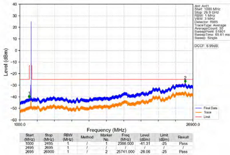
n41_30kHz_SISO_NTNV_90MHz_DFT-s-OFDM_PI/2_BPSK_2644.98MHz_Edge_1RB_Right
