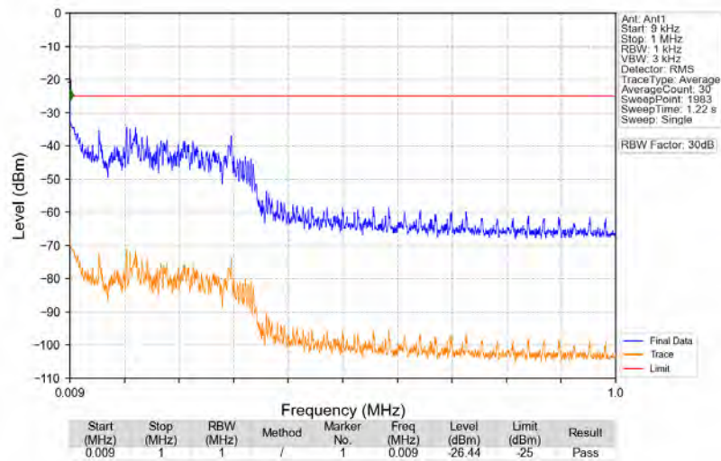
n41_30kHz_SISO_NTNV_80MHz_DFT-s-OFDM_QPSK_2649.99MHz_Edge_1RB_Right
