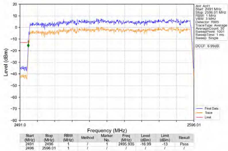
n41_30kHz_SISO_NTNV_100MHz_DFT-s-OFDM_QPSK_2546.01MHz_Outer_Full
