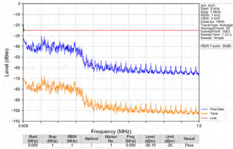
n41_30kHz_SISO_NTNV_100MHz_DFT-s-OFDM_QPSK_2592.99MHz_Edge_1RB_Left
