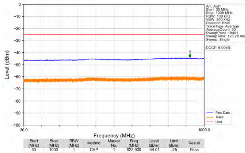
n41_30kHz_SISO_NTNV_100MHz_DFT-s-OFDM_QPSK_2640MHz_Edge_1RB_Right
