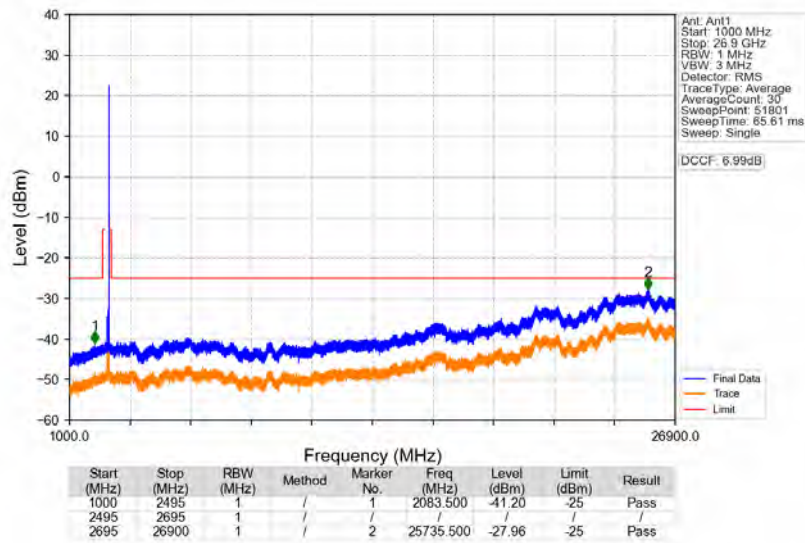
n41_30kHz_SISO_NTNV_90MHz_CP-OFDM_QPSK_2644.98MHz_Edge_1RB_Right
