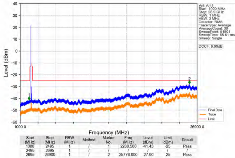
n41_30kHz_SISO_NTNV_100MHz_DFT-s-OFDM_QPSK_2592.99MHz_Edge_1RB_Left
