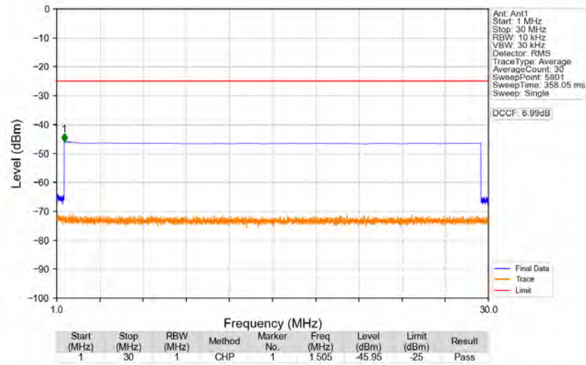
n41_30kHz_SISO_NTNV_100MHz_DFT-s-OFDM_QPSK_2592.99MHz_Edge_1RB_Left
