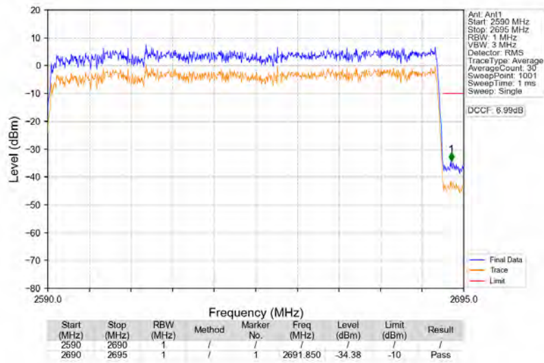
n41_30kHz_SISO_NTNV_100MHz_DFT-s-OFDM_PI/2_BPSK_2640MHz_Outer_Full
