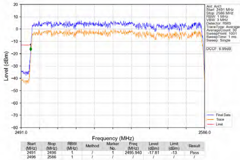
n41_30kHz_SISO_NTNV_90MHz_DFT-s-OFDM PI/2 BPSK_2541MHz_Outer_Full
