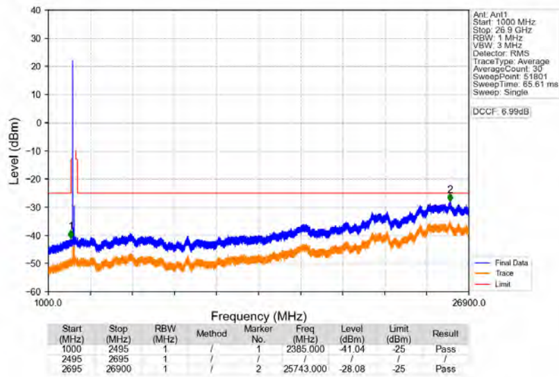
n41_30kHz_SISO_NTNV_100MHz_DFT-s-OFDM PI/2 BPSK 2546.01MHz_Edge_1RB_Left
