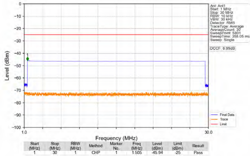
n41_30kHz_SISO_NTNV_90MHz_DFT-s-OFDM_QPSK_2592.99MHz_Edge_1RB_Left
