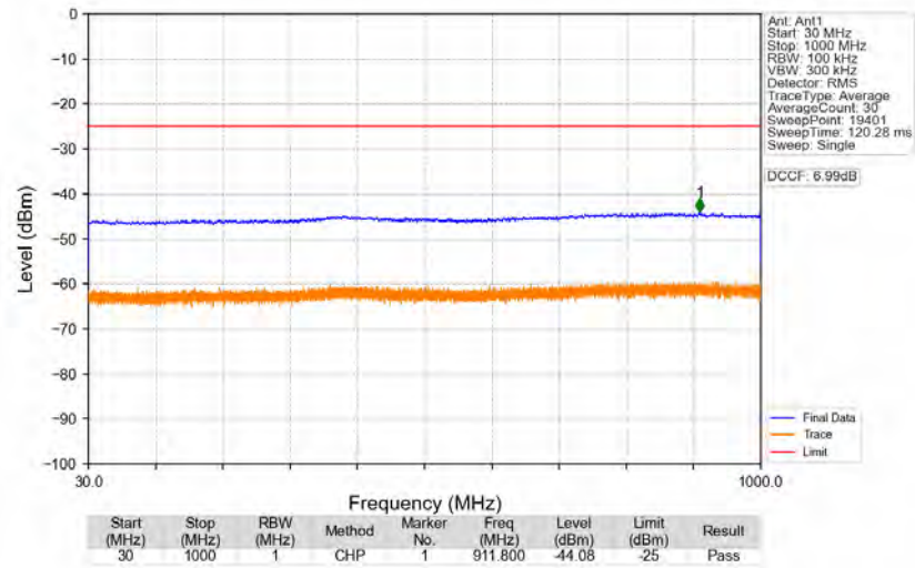
n41_30kHz_SISO_NTNV_90MHz_DFT-s-OFDM_QPSK_2541MHz_Edge_1RB_Left
