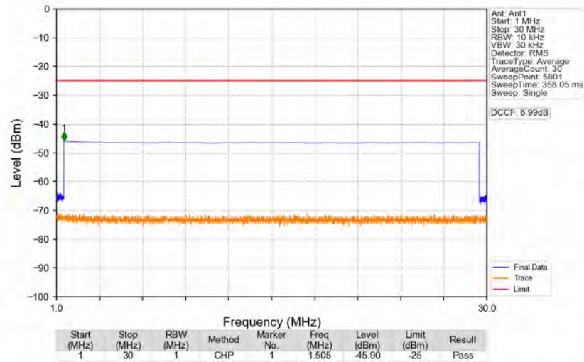
n41_30kHz_SISO_NTNV_80MHz_DFT-s-OFDM_QPSK_2592.99MHz_Edge_1RB_Left
