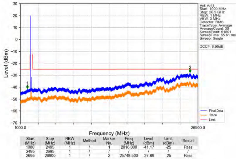
n41_30kHz_SISO_NTNV_100MHz_CP-OFDM_QPSK_2546.01MHz_Edge_1RB_Left
