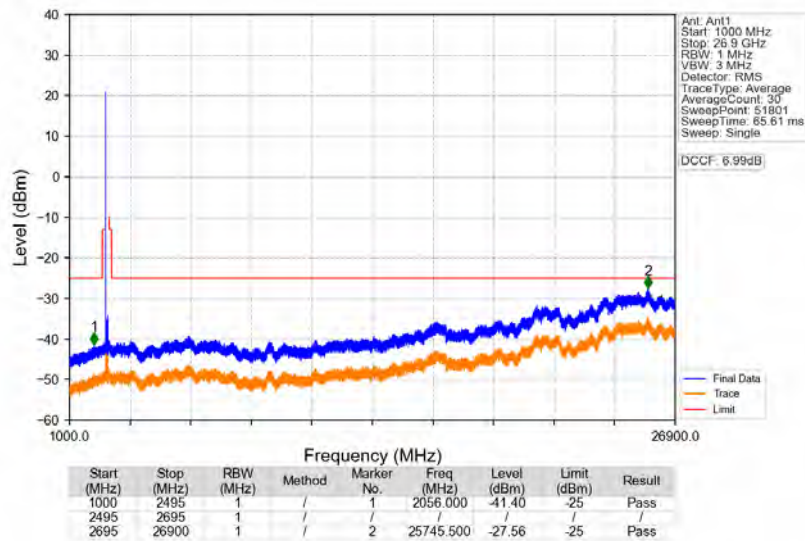
n41_30kHz_SISO_NTNV_100MHz_CP-OFDM_QPSK_2592.99MHz_Edge_1RB_Left
