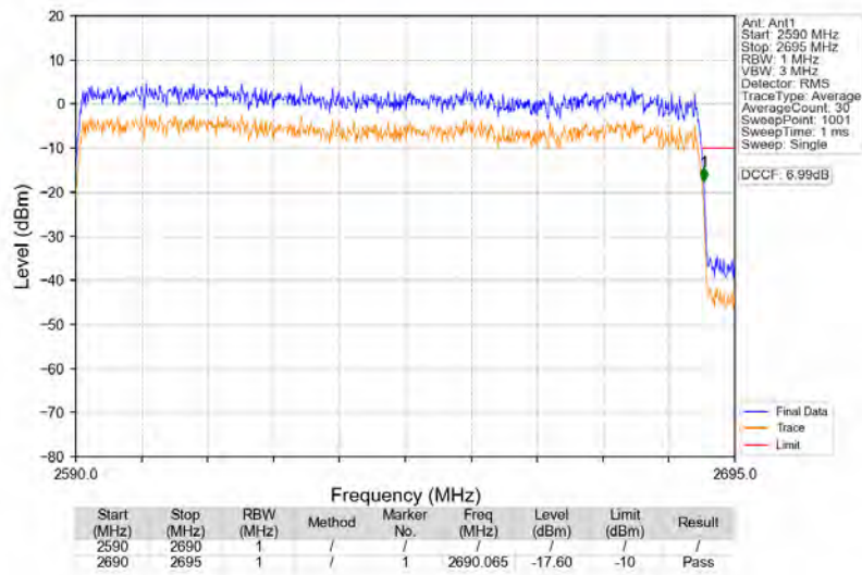
n41_30kHz_SISO_NTNV_100MHz_CP-OFDM_QPSK_2640MHz_Outer_Full
