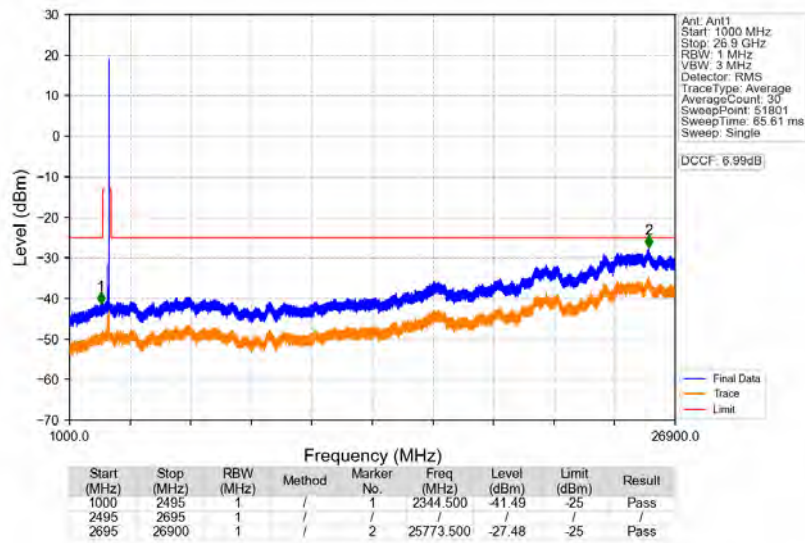
n41_30kHz_SISO_NTNV_80MHz_DFT-s-OFDM_QPSK_2649.99MHz_Edge_1RB_Right
