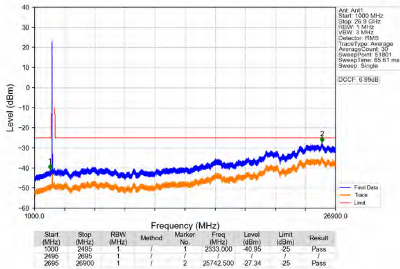
n41_30kHz_SISO_NTNV_80MHz_CP-OFDM_QPSK_2536.02MHz_Edge_1RB_Left
