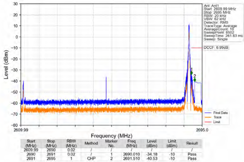
n41_30kHz_SISO_NTNV_80MHz_CP-OFDM_QPSK_2649.99MHz_Edge_1RB_Right
