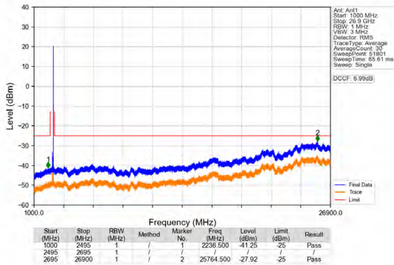
n41_30kHz_SISO_NTNV_90MHz_DFT-s-OFDM_QPSK_2644.98MHz_Edge_1RB_Right
