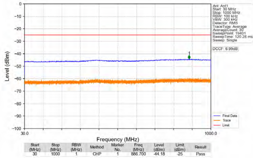
n41_30kHz_SISO_NTNV_80MHz_CP-OFDM_QPSK_2592.99MHz_Edge_1RB_Left
