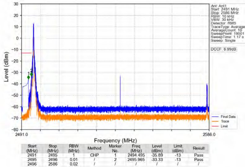
n41_30kHz_SISO_NTNV_90MHz_DFT-s-OFDM_QPSK_2541MHz_Edge_1RB_Left
