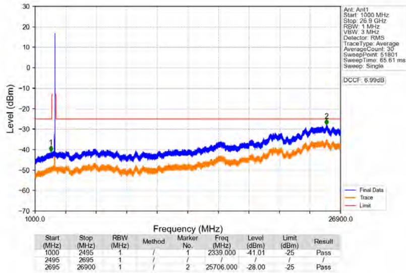
n41_30kHz_SISO_NTNV_80MHz_CP-OFDM_QPSK_2649.99MHz_Edge_1RB_Right
