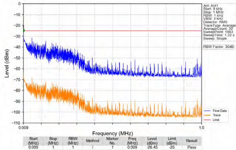
n41_30kHz_SISO_NTNV_100MHz_CP-OFDM_QPSK_2640MHz_Edge_1RB_Right
