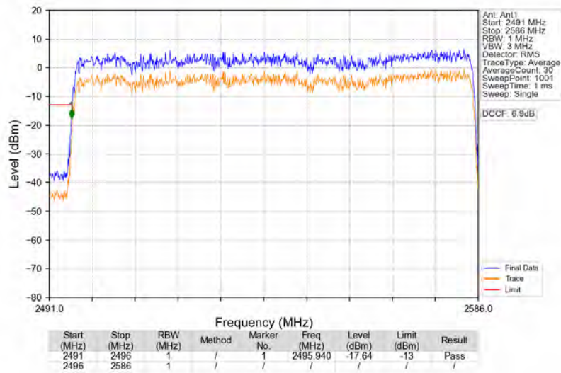
n41_30kHz_SISO_NTNV_90MHz_DFT-s-OFDM_QPSK_2541MHz_Outer_Full
