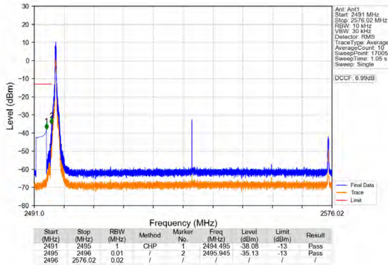
n41_30kHz_SISO_NTNV_80MHz_CP-OFDM_QPSK_2536.02MHz_Edge_1RB_Left
