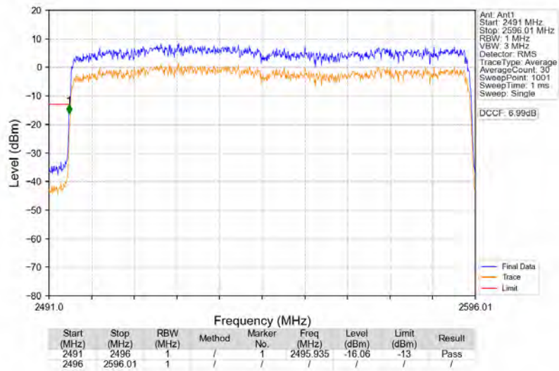
n41_30kHz_SISO_NTNV_100MHz_DFT-s-OFDM PI/2 BPSK 2546.01MHz_Outer_Full
