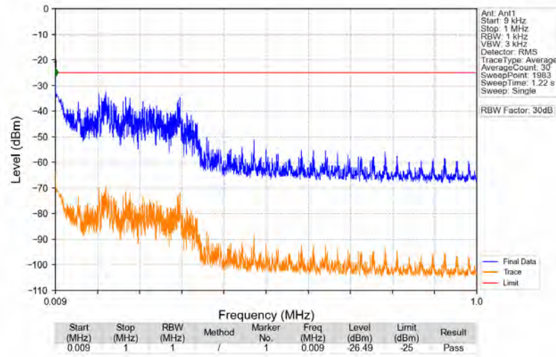
n41_30kHz_SISO_NTNV_90MHz_DFT-s-OFDM_QPSK_2592.99MHz_Edge_1RB_Left
