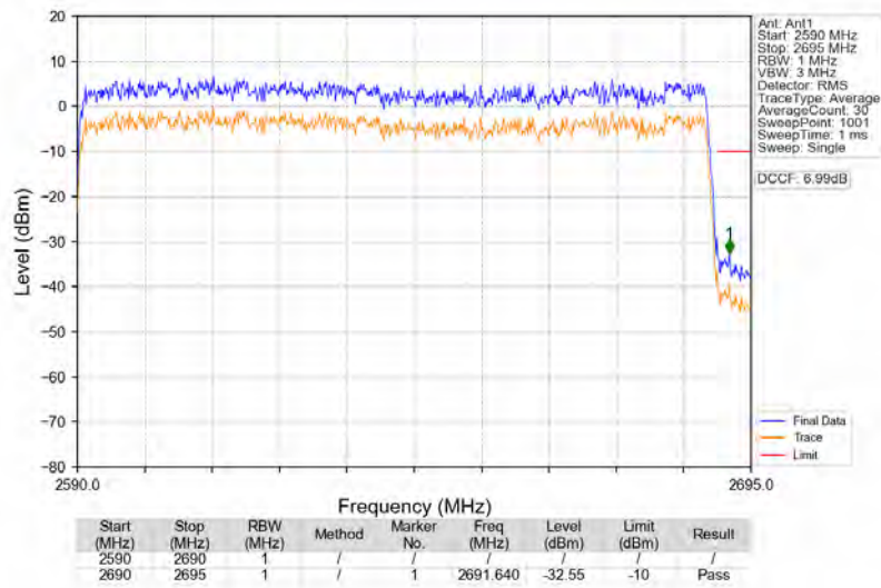
n41_30kHz_SISO_NTNV_100MHz_DFT-s-OFDM_QPSK_2640MHz_Outer_Full
