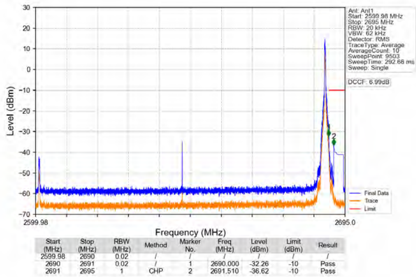
n41_30kHz_SISO_NTNV_90MHz_DFT-s-OFDM_QPSK_2644.98MHz_Edge_1RB_Right
