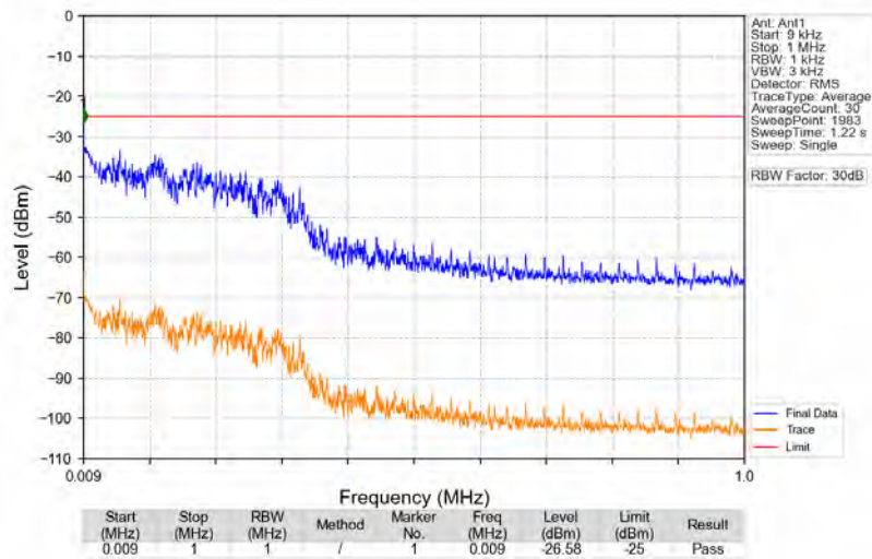
n41_30kHz_SISO_NTNV_100MHz_CP-OFDM_QPSK_2546.01MHz_Edge_1RB_Left
