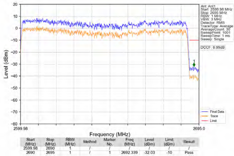
n41_30kHz_SISO_NTNV_90MHz_DFT-s-OFDM_PI/2_BPSK_2644.98MHz_Outer_Full
