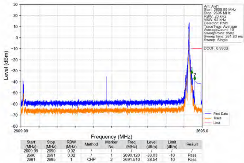
n41_30kHz_SISO_NTNV_80MHz_DFT-s-OFDM_QPSK_2649.99MHz_Edge_1RB_Right
