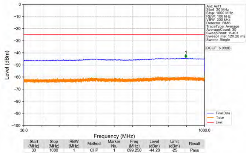
n41_30kHz_SISO_NTNV_80MHz_CP-OFDM_QPSK_2536.02MHz_Edge_1RB_Left
