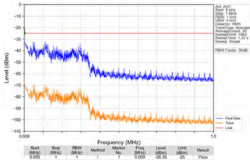
n41_30kHz_SISO_NTNV_100MHz_DFT-s-OFDM_PI/2_BPSK_2640MHz_Edge_1RB_Right
