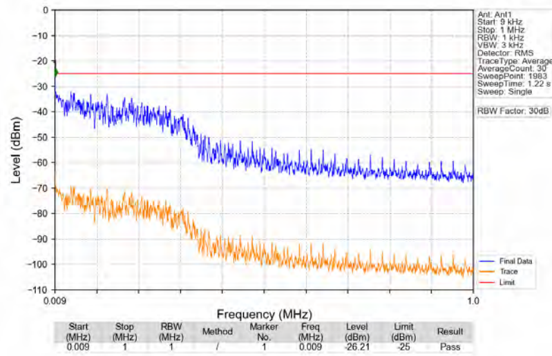
n41_30kHz_SISO_NTNV_80MHz_CP-OFDM_QPSK_2592.99MHz_Edge_1RB_Left
