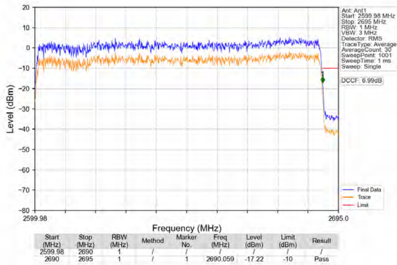
n41_30kHz_SISO_NTNV_90MHz_CP-OFDM_QPSK_2644.98MHz_Outer_Full
