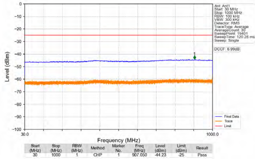
n41_30kHz_SISO_NTNV_100MHz_DFT-s-OFDM_QPSK_2592.99MHz_Edge_1RB_Left
