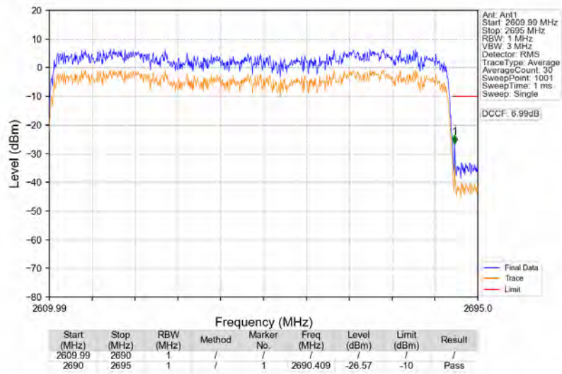
n41_30kHz_SISO_NTNV_80MHz_DFT-s-OFDM_QPSK_2649.99MHz_Outer_Full
