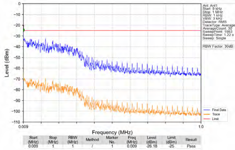
n41_30kHz_SISO_NTNV_100MHz_CP-OFDM_QPSK_2592.99MHz_Edge_1RB_Left
