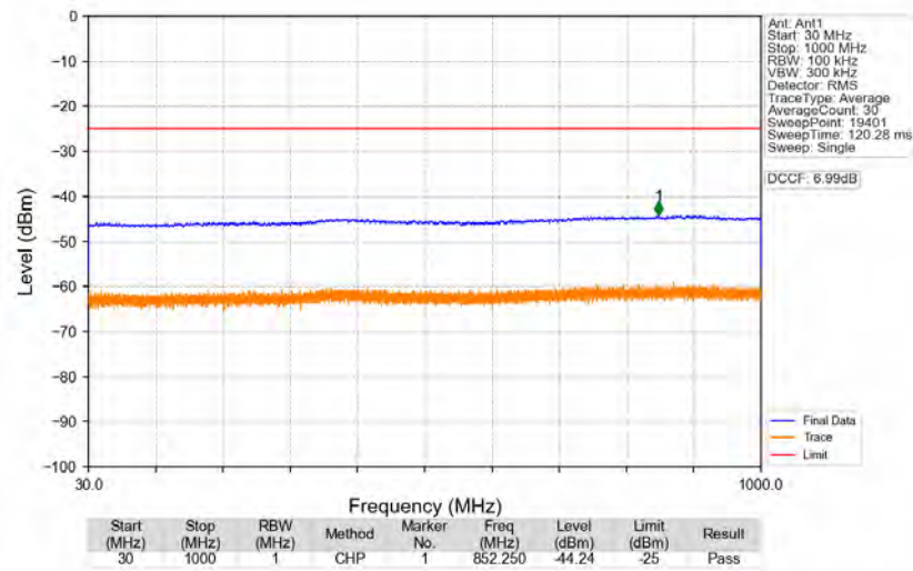
n41_30kHz_SISO_NTNV_90MHz_CP-OFDM_QPSK_2644.98MHz_Edge_1RB_Right
