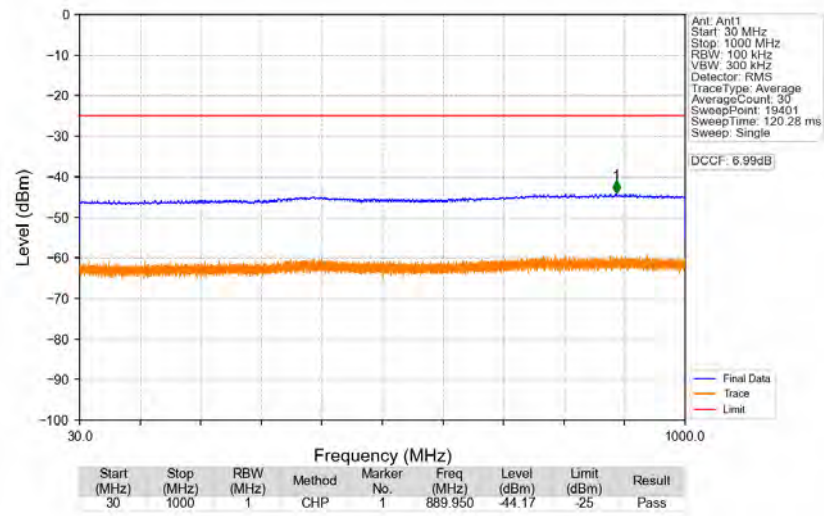
n41_30kHz_SISO_NTNV_100MHz_CP-OFDM_QPSK_2592.99MHz_Edge_1RB_Left
