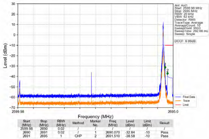
n41_30kHz_SISO_NTNV_90MHz_CP-OFDM_QPSK_2644.98MHz_Edge_1RB_Right
