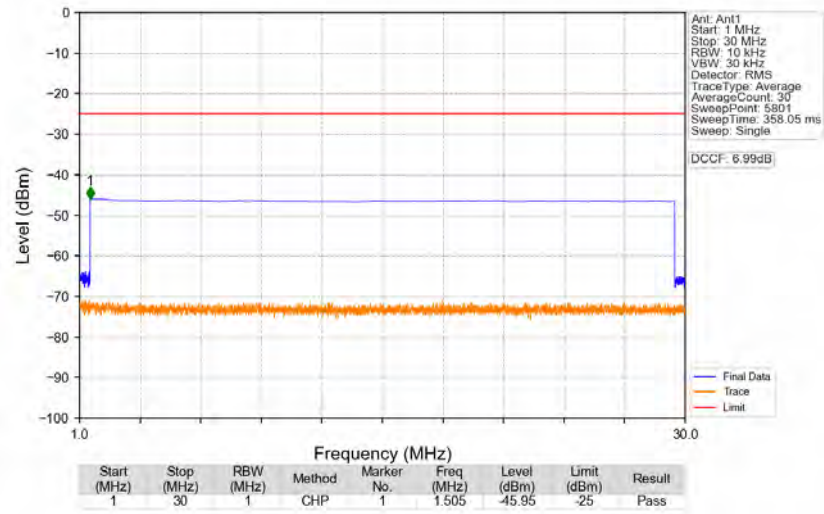
n41_30kHz_SISO_NTNV_100MHz_CP-OFDM_QPSK_2640MHz_Edge_1RB_Right
