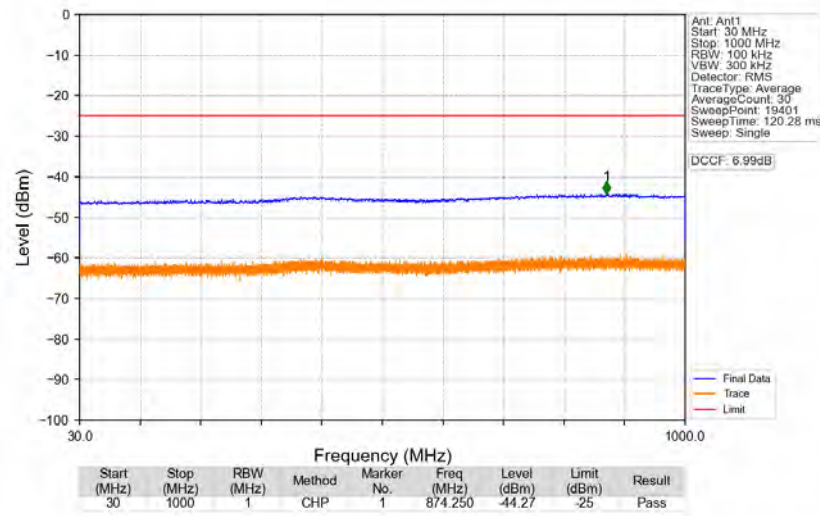
n41_30kHz_SISO_NTNV_90MHz_DFT-s-OFDM_QPSK_2592.99MHz_Edge_1RB_Left
