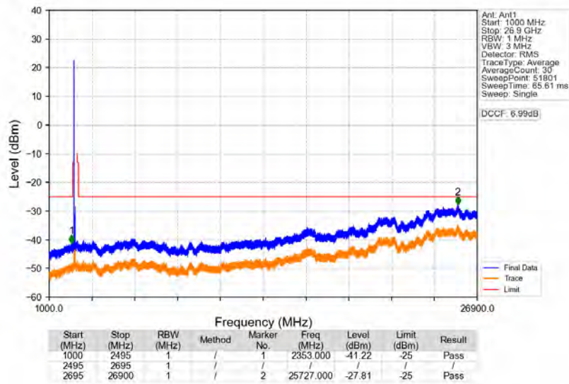
n41_30kHz_SISO_NTNV_80MHz_DFT-s-OFDM_QPSK_2536.02MHz_Edge_1RB_Left
