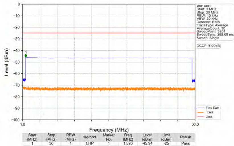
n41_30kHz_SISO_NTNV_90MHz_CP-OFDM_QPSK_2592.99MHz_Edge_1RB_Left
