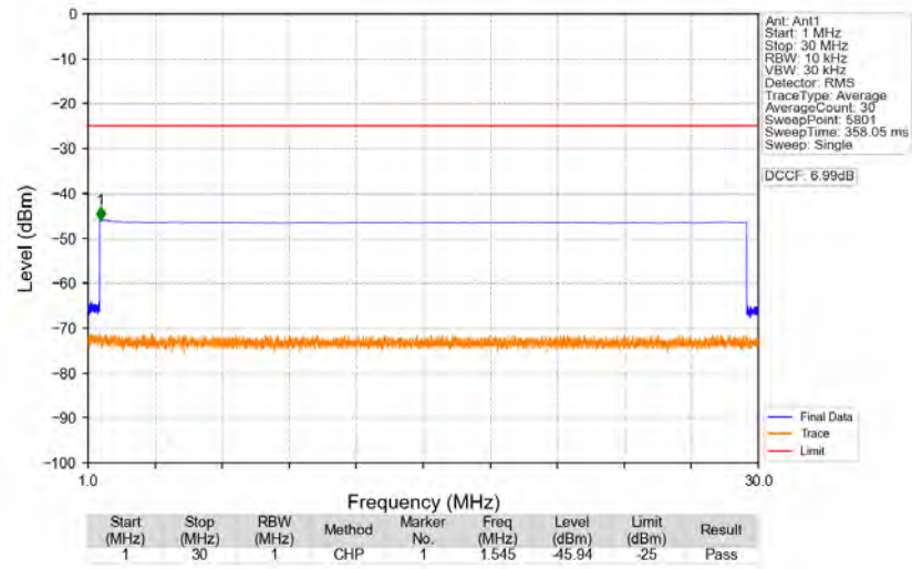
n41_30kHz_SISO_NTNV_100MHz_CP-OFDM_QPSK_2546.01MHz_Edge_1RB_Left
