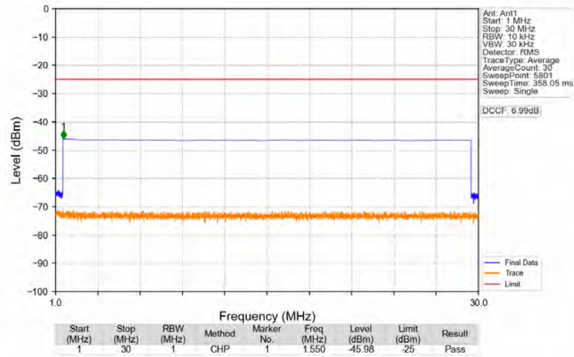
n41_30kHz_SISO_NTNV_100MHz_CP-OFDM_QPSK_2592.99MHz_Edge_1RB_Left
