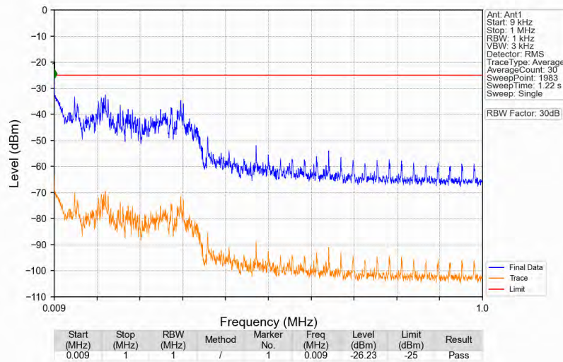
n41_30kHz_SISO_NTNV_100MHz_DFT-s-OFDM PI/2 BPSK_2546.01MHz_Edge_1RB_Left
