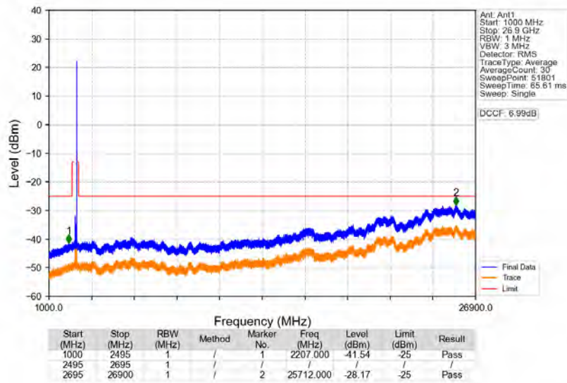
n41_30kHz_SISO_NTNV_100MHz_DFT-s-OFDM_QPSK_2640MHz_Edge_1RB_Right
