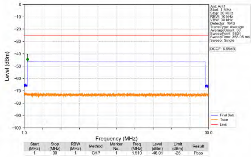
n41_30kHz_SISO_NTNV_80MHz_CP-OFDM_QPSK_2649.99MHz_Edge_1RB_Right
