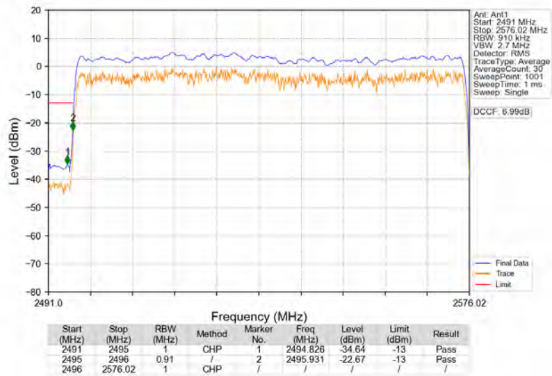
n41_30kHz_SISO_NTNV_80MHz_DFT-s-OFDM_QPSK_2536.02MHz_Outer_Full
