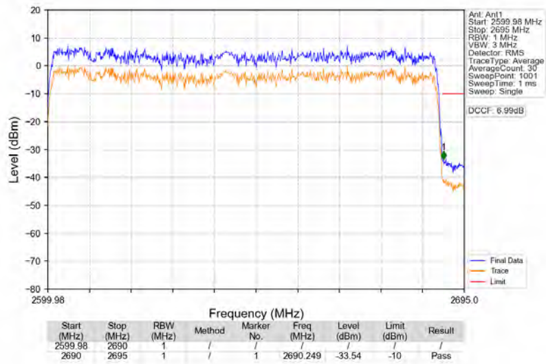
n41_30kHz_SISO_NTNV_90MHz_DFT-s-OFDM_QPSK_2644.98MHz_Outer_Full
