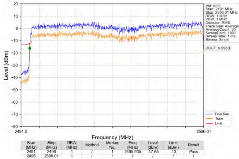
n41_30kHz_SISO_NTNV_100MHz_CP-OFDM_QPSK_2546.01MHz_Outer_Full
