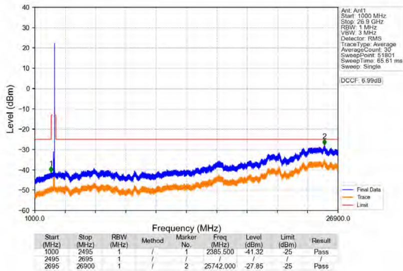
n41_30kHz_SISO_NTNV_100MHz_DFT-s-OFDM_PI/2_BPSK_2640MHz_Edge_1RB_Right
