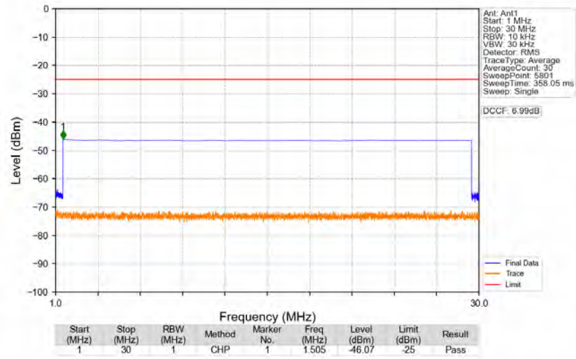
n41_30kHz_SISO_NTNV_90MHz_DFT-s-OFDM_QPSK_2541MHz_Edge_1RB_Left
