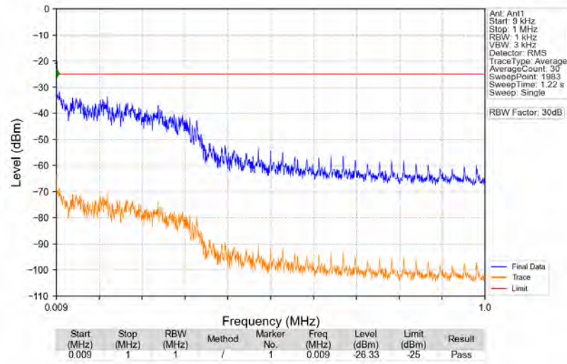
n41_30kHz_SISO_NTNV_90MHz_CP-OFDM_QPSK_2592.99MHz_Edge_1RB_Left
