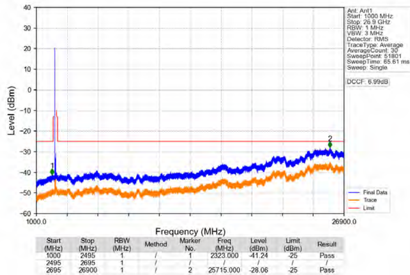
n41_30kHz_SISO_NTNV_90MHz_CP-OFDM_QPSK_2592.99MHz_Edge_1RB_Left
