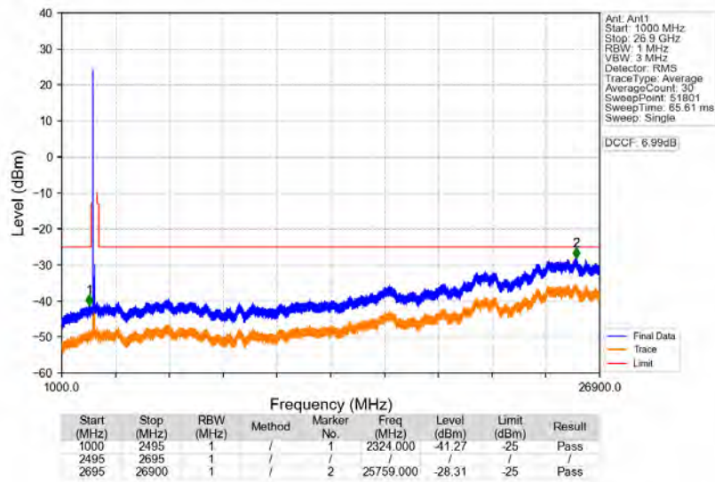
n41_30kHz_SISO_NTNV_90MHz_DFT-s-OFDM_QPSK_2541MHz_Edge_1RB_Left
