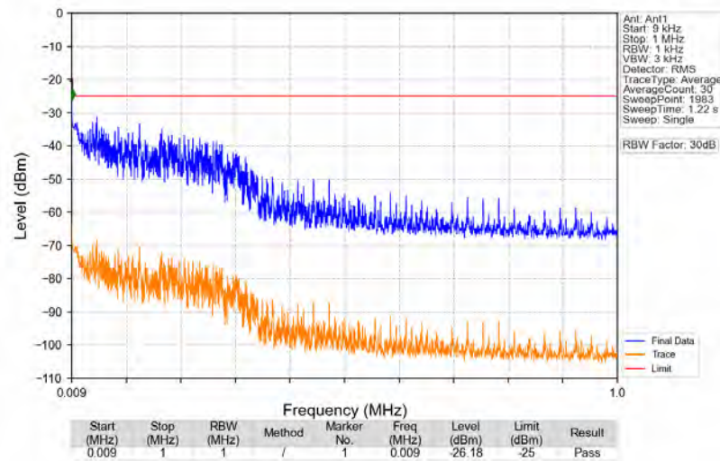
n41_30kHz_SISO_NTNV_80MHz_CP-OFDM_QPSK_2536.02MHz_Edge_1RB_Left
