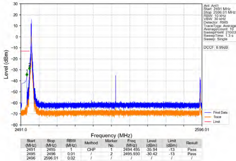
n41_30kHz_SISO_NTNV_100MHz_DFT-s-OFDM_QPSK_2546.01MHz_Edge_1RB_Left
