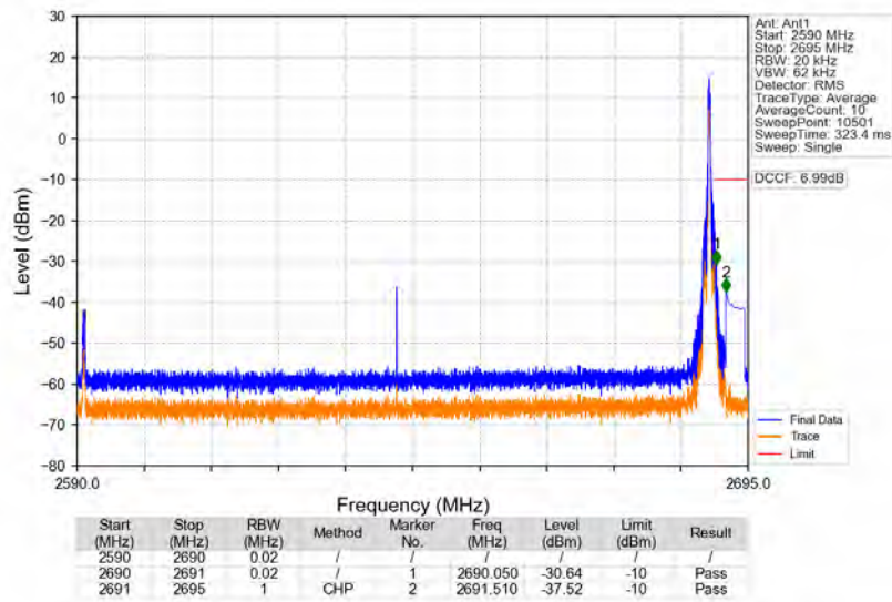
n41_30kHz_SISO_NTNV_100MHz_DFT-s-OFDM_PI/2_BPSK_2640MHz_Edge_1RB_Right
