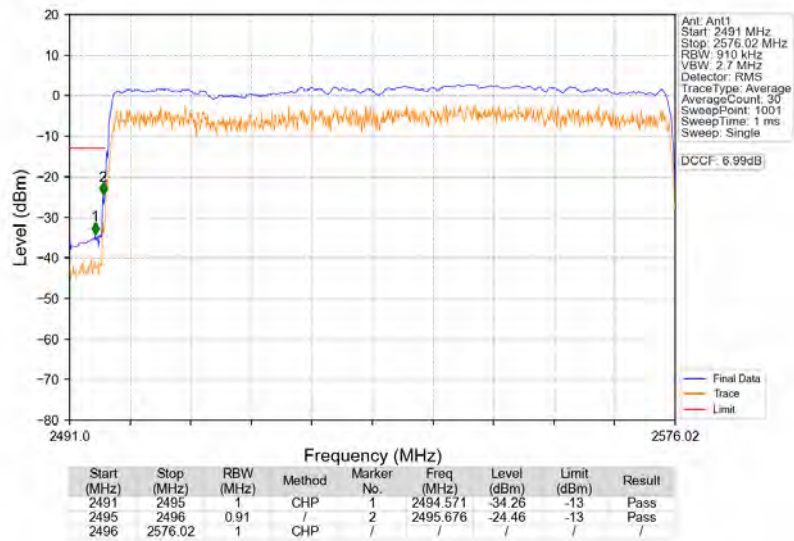
n41_30kHz_SISO_NTNV_80MHz_CP-OFDM_QPSK_2536.02MHz_Outer_Full
