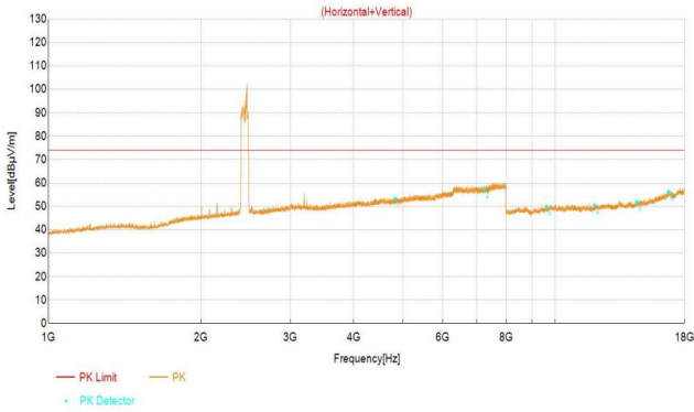
BT_3DH5_2480
