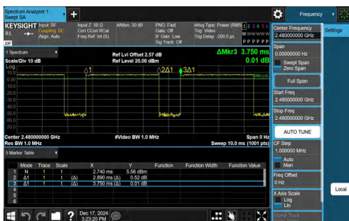
NTVN-3DH5-Ant1-2480
