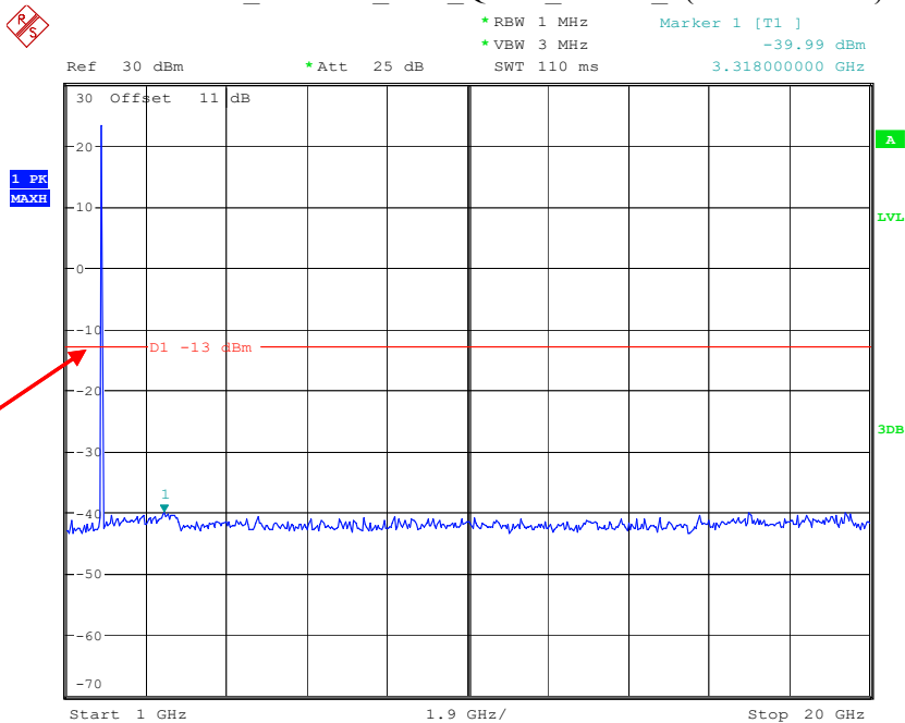
Band 2_1.4 MHz_Low_QPSK_RB1#0_2(1GHz-20GHz)
