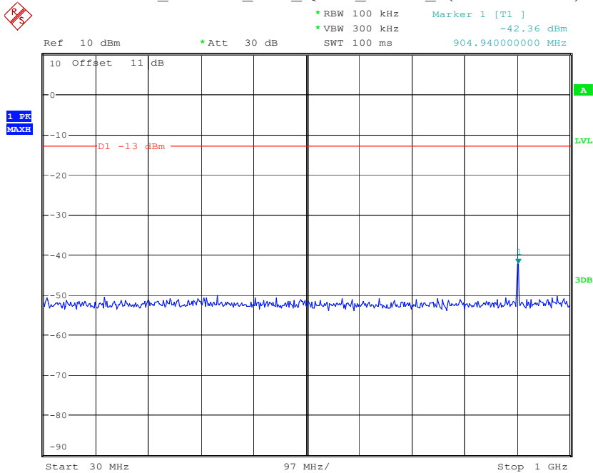
Band 2_1.4 MHz_Low_QPSK_RB1#0_1(30MHz-1GHz)
