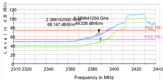
802.11g-Channel 3 Peak+ Average
