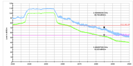
802.11g-Channel 8 Peak+ Average
