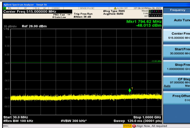
Band2-3MHz-16QAM-19185-1RB#0-30~1000MHz
