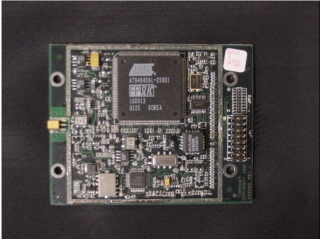
Figure 2: EUT front with shield removed
