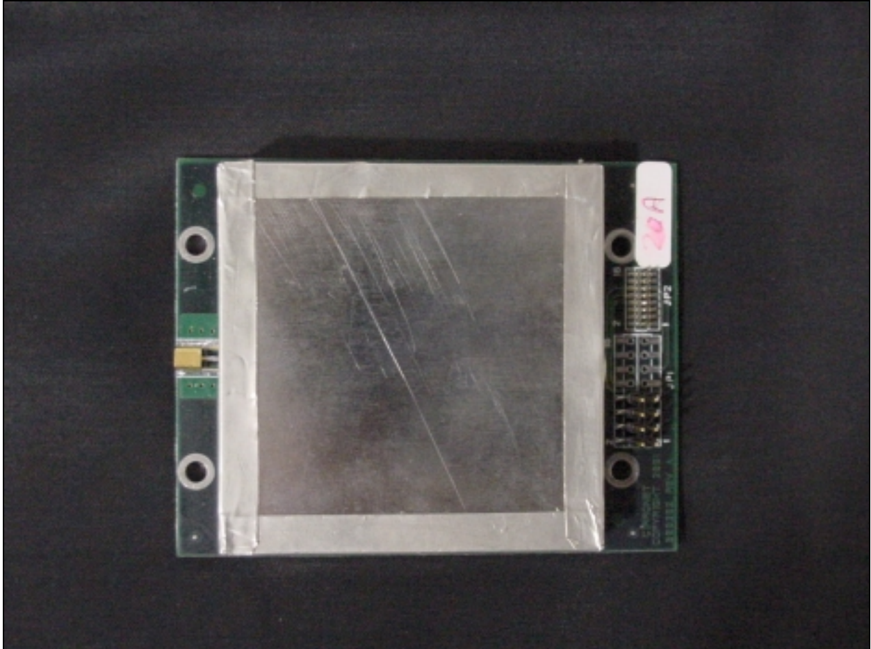
Figure 1: EUT Front with Shield
