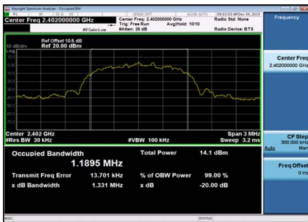
99% Bandwidth: 8DPSK,2402MHz,3DH5
