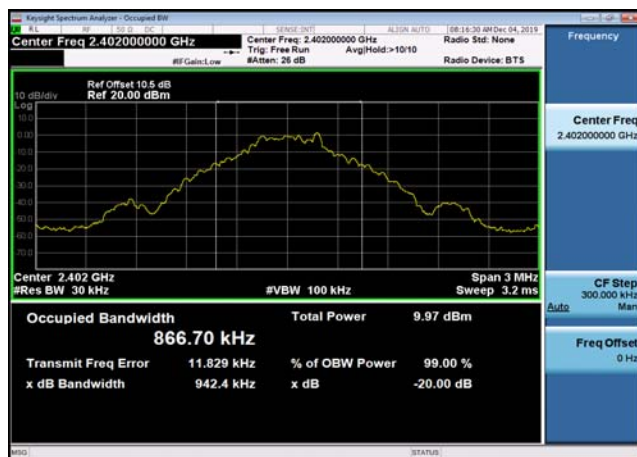
99% Bandwidth: GFSK,2402MHz,DH5
