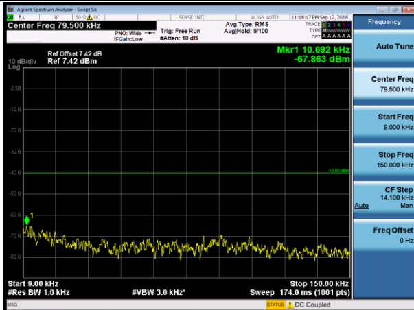
1.4MHz_LCH_QPSK_1RB#0
