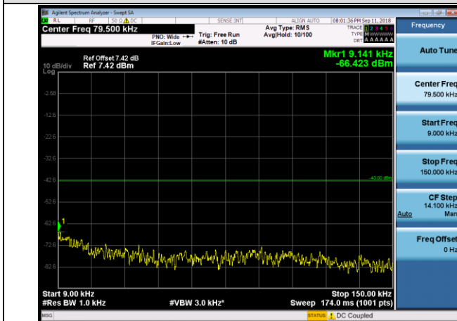
1.4MHz_LCH_QPSK_1RB#0
