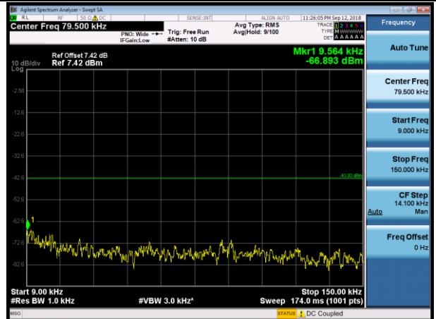
10MHz_LCH_QPSK_1RB#0
