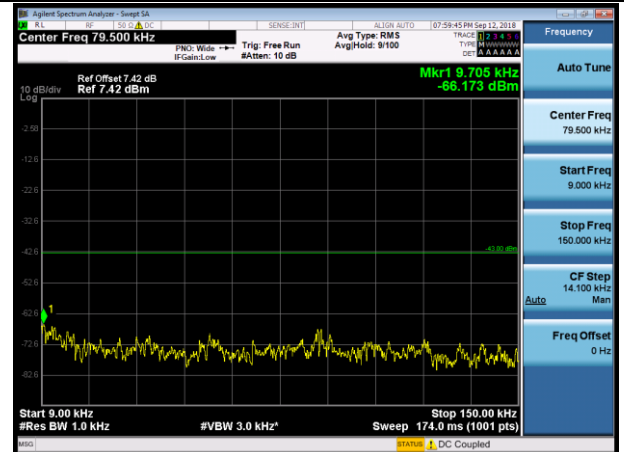
10MHz_LCH_QPSK_1RB#0
