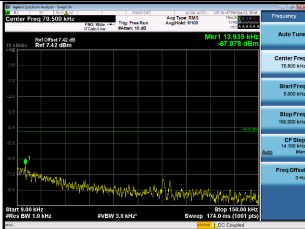
5MHz_LCH_QPSK_1RB#0
