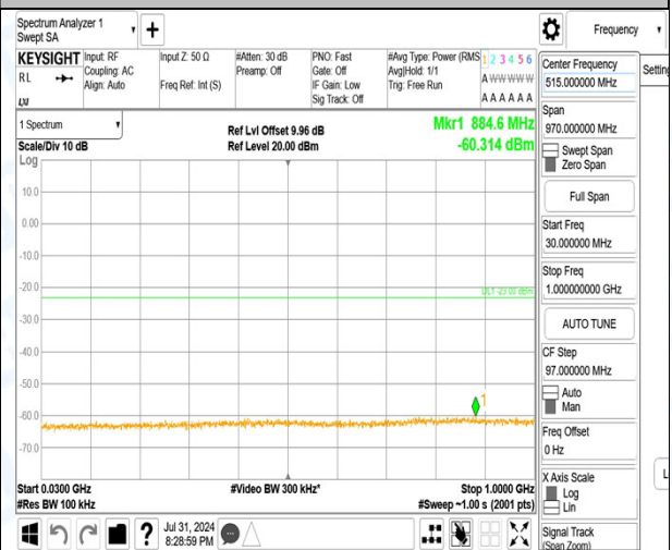
Band4_1.4MHz_16QAM_20393_6RB#0_3000~20000_3000~20000
