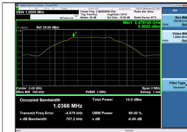
6dB bandwidth
