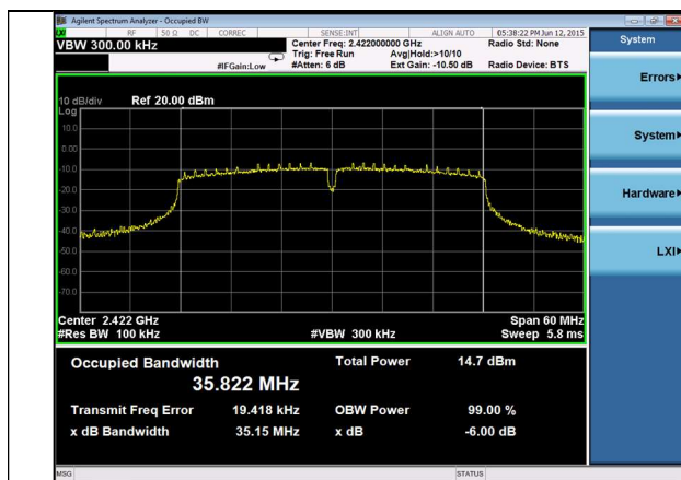
802.11n (HT40) 6dB bandwidth
