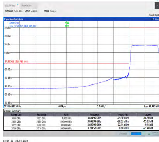
1-N77-3700-3980-PC2-30-10-L-6-CP-QPSK-Outer _Full-24@0-Ant1-PASS-see graph
