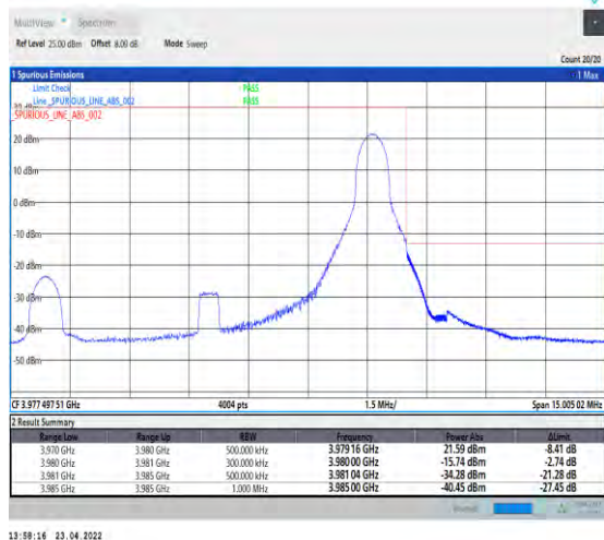
1-N77-3700-3980-PC2-30-10-H-5-CP-QPSK-Edge_1R B_Right-1@23-Ant1-PASS-see graph
