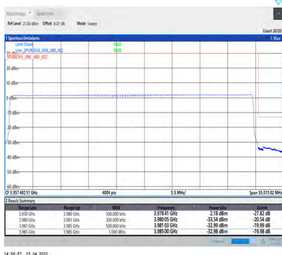
1-N77-3700-3980-PC2-30-50-H-6-CP-QPSK-Outer _Full-133@0-Ant1-PASS-see graph
