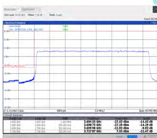
1-N77-3700-3980--30-40-L-3-DFT-PI2BPSK-Outer_Full-100@0-Ant1-PASS-see graph
