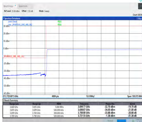
1-N77-3700-3980-PC2-30-90-L-6-CP-QPSK-Outer _Full-245@0-Ant1-PASS-see graph
