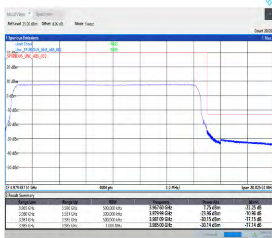
1-N77-3700-3980-PC2-30-15-H-6-CP-QPSK-Outer _Full-38@0-Ant1-PASS-see graph
