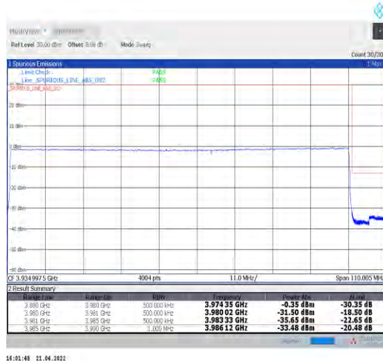
1-N77-3700-3980--30-100-H-6-CP-QPSK-Outer_F ull-273@0-Ant1-PASS-see graph
