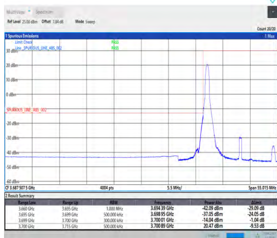
1-N77-3700-3980-PC2-30-15-L-4-CP-QPSK-Edge_1R B_Left-1@0-Ant1-PASS-see graph
