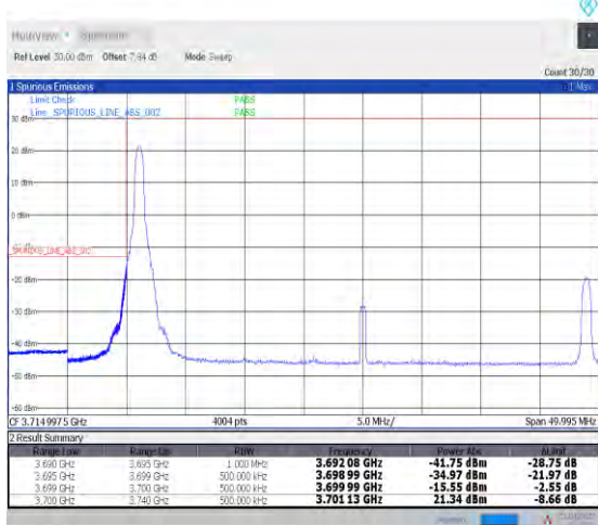
1-N77-3700-3980--30-40-L-1-DFT-PI2BPSK-Edge_1R_B_Left-1@0-Ant1-PASS-see graph
