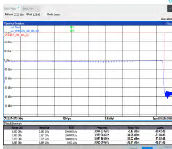
1-N77-3700-3980-PC2-30-90-H-6-CP-QPSK-Outer _Full-245@0-Ant1-PASS-see graph
