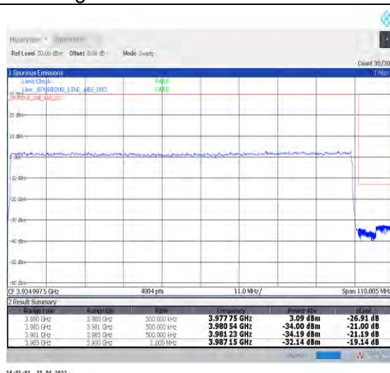
1-N77-3700-3980--30-100-H-3-DFT-PI2BPSK-Out er_Full-270@0-Ant1-PASS-see graph
