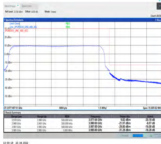
1-N77-3700-3980-PC2-30-10-H-6-CP-QPSK-Outer _Full-24@0-Ant1-PASS-see graph
