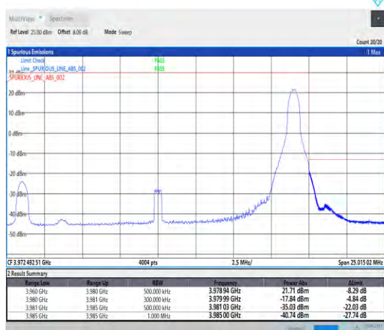
1-N77-3700-3980-PC2-30-20-H-5-CP-QPSK-Edge_1R B_Right-1@50-Ant1-PASS-see graph
