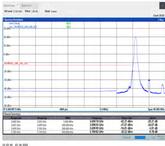
1-N77-3700-3980-PC2-30-10-L-4-CP-QPSK-Edge_1R B_Left-1@0-Ant1-PASS-see graph
