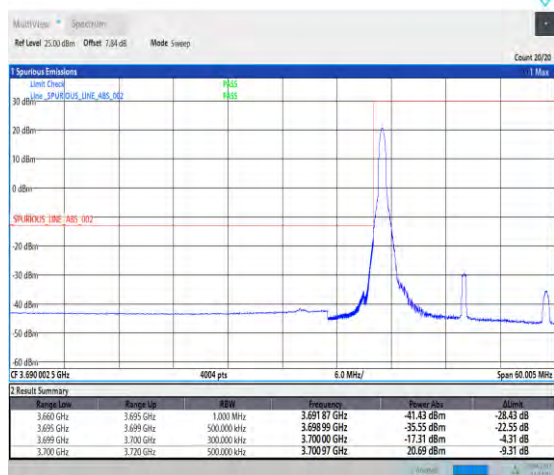
1-N77-3700-3980-PC2-30-20-L-4-CP-QPSK-Edge_1R B_Left-1@0-Ant1-PASS-see graph
