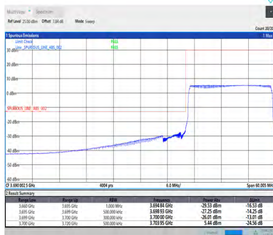
1-N77-3700-3980-PC2-30-20-L-6-CP-QPSK-Outer _Full-51@0-Ant1-PASS-see graph
