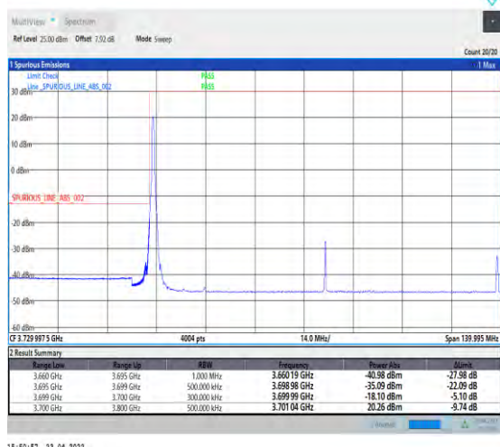
1-N77-3700-3980-PC2-30-100-L-4-CP-QPSK-Edge_1 RB_Left-1@0-Ant1-PASS-see graph
