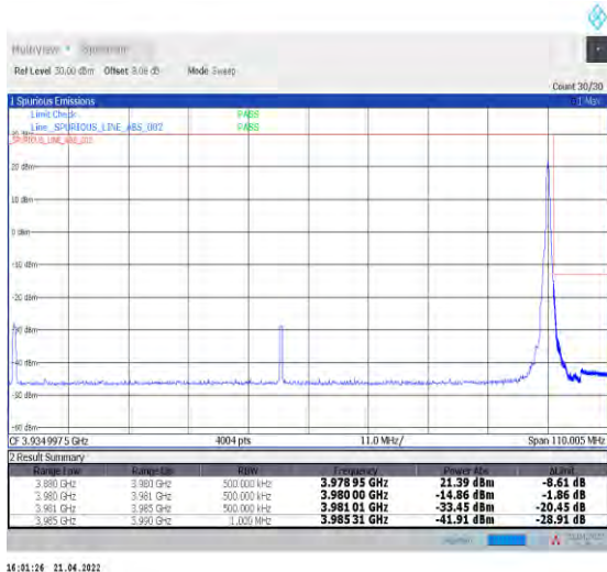
1-N77-3700-3980--30-100-H-5-CP-QPSK-Edge_1RB_ Right-1@272-Ant1-PASS-see graph
