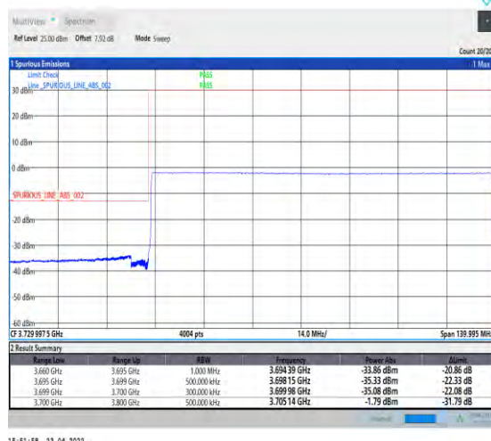
1-N77-3700-3980-PC2-30-100-L-6-CP-QPSK-Out er_Full-273@0-Ant1-PASS-see graph
