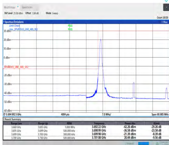
1-N77-3700-3980-PC2-30-30-L-4-CP-QPSK-Edge_1R B_Left-1@0-Ant1-PASS-see graph
