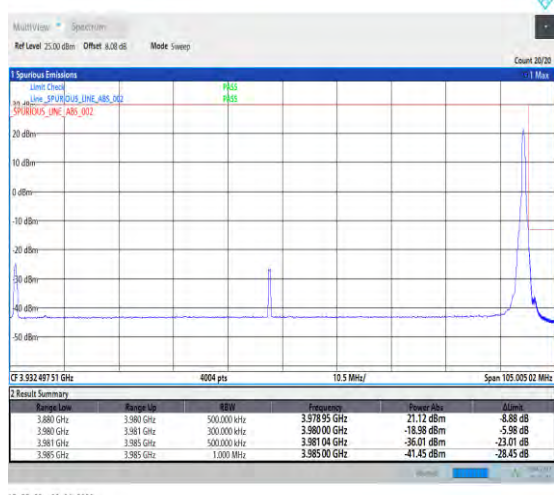
1-N77-3700-3980-PC2-30-100-H-5-CP-QPSK-Edge_1 RB_Right-1@272-Ant1-PASS-see graph
