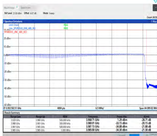
1-N77-3700-3980-PC2-30-60-H-6-CP-QPSK-Outer _Full-162@0-Ant1-PASS-see graph
