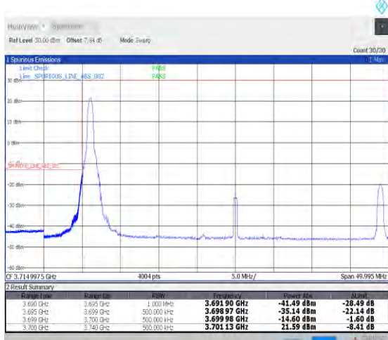
1-N77-3700-3980--30-40-L-4-CP-QPSK-Edge_1RB_L_eff-1@0-Ant1-PASS-see graph
