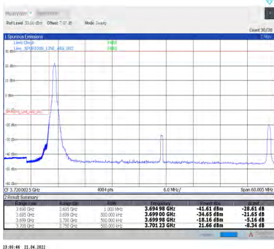
1-N77-3700-3980--30-50-L-4-CP-QPSK-Edge_1RB_L_eff-1@0-Ant1-PASS-see graph
