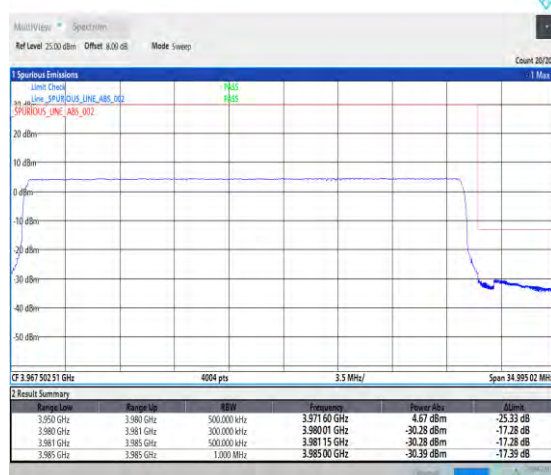
1-N77-3700-3980-PC2-30-30-H-6-CP-QPSK-Outer _Full-78@0-Ant1-PASS-see graph
