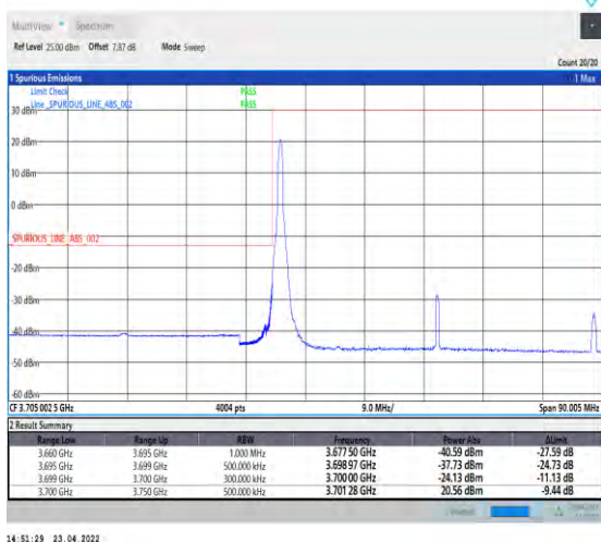
1-N77-3700-3980-PC2-30-50-L-4-CP-QPSK-Edge_1R B_Left-1@0-Ant1-PASS-see graph
