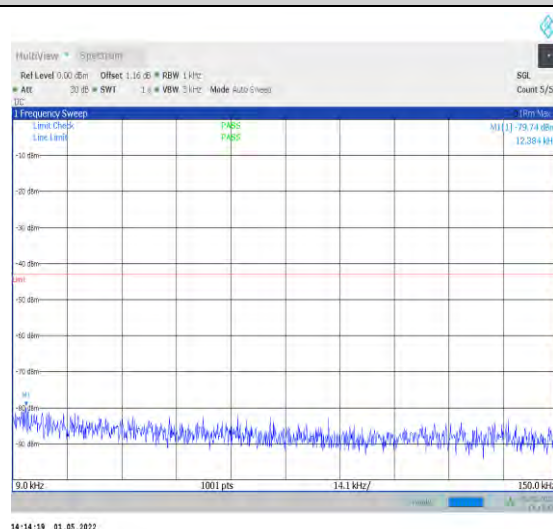
1-N77-3700-3980-PC2-30-100-L-1-DFT-QPSK-Edge _1RB_Left-1@0-6000-26000-Ant1--42.53--13-PASS
