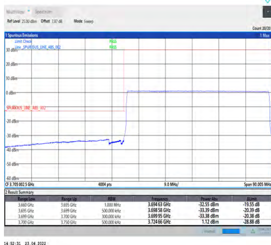
1-N77-3700-3980-PC2-30-50-L-6-CP-QPSK-Outer _Full-133@0-Ant1-PASS-see graph
