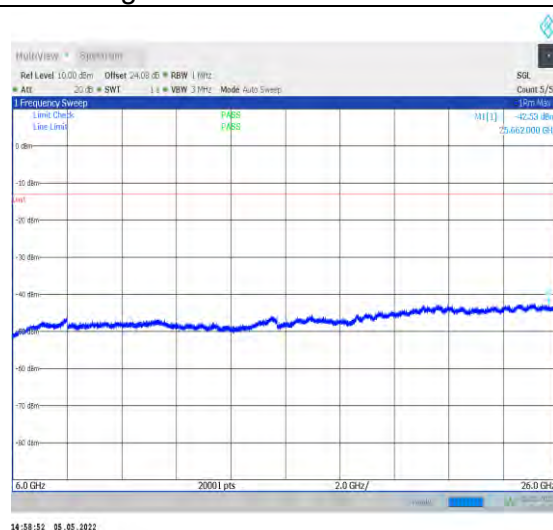
1-N77-3700-3980-PC2-30-100-L-1-DFT-QPSK-Edge _1RB_Left-1@0-6000-26000-Ant1--42.53--13-PASS
