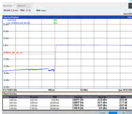
1-N77-3700-3980-PC2-30-60-L-6-CP-QPSK-Outer _Full-162@0-Ant1-PASS-see graph
