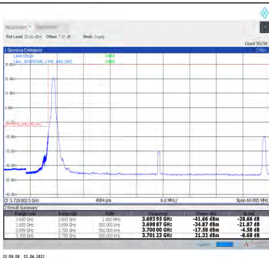
1-N77-3700-3980--30-50-L-1-DFT-PI2BPSK-Edge_1R_B_Left-1@0-Ant1-PASS-see graph
