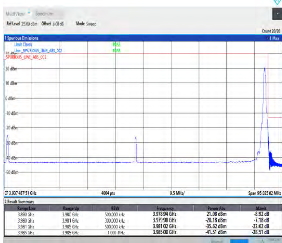
1-N77-3700-3980-PC2-30-90-H-5-CP-QPSK-Edge_1R B_Right-1@244-Ant1-PASS-see graph
