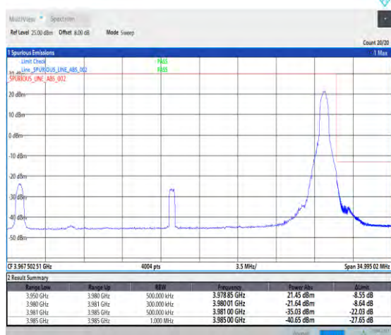
1-N77-3700-3980-PC2-30-30-H-5-CP-QPSK-Edge_1R B_Right-1@77-Ant1-PASS-see graph
