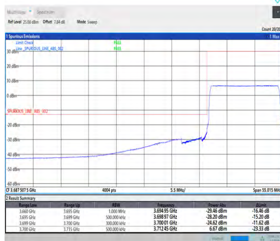
1-N77-3700-3980-PC2-30-15-L-6-CP-QPSK-Outer _Full-38@0-Ant1-PASS-see graph
