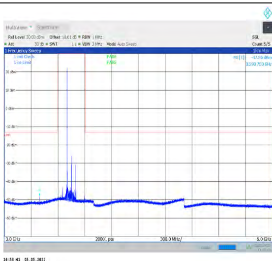
1-N77-3700-3980-PC2-30-100-L-1-DFT-QPSK-Edge _1RB_Left-1@0-3000-6000-Ant1--47.86--13-PASS
