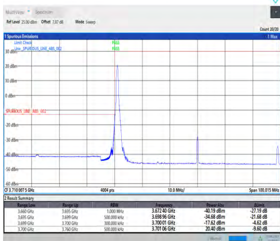
1-N77-3700-3980-PC2-30-60-L-4-CP-QPSK-Edge_1R B_Left-1@0-Ant1-PASS-see graph
