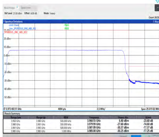
1-N77-3700-3980-PC2-30-20-H-6-CP-QPSK-Outer _Full-51@0-Ant1-PASS-see graph
