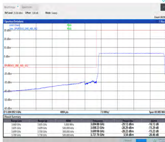
1-N77-3700-3980-PC2-30-30-L-6-CP-QPSK-Outer _Full-78@0-Ant1-PASS-see graph
