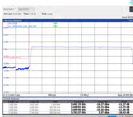
1-N77-3700-3980--30-40-L-6-CP-QPSK-Outer_Ful_I-106@0-Ant1-PASS-see graph
