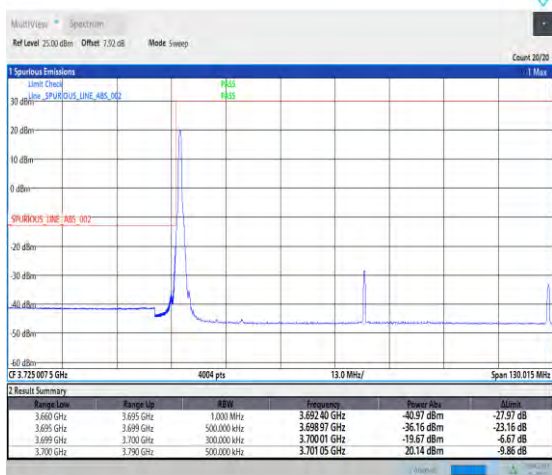
1-N77-3700-3980-PC2-30-90-L-4-CP-QPSK-Edge_1R B_Left-1@0-Ant1-PASS-see graph
