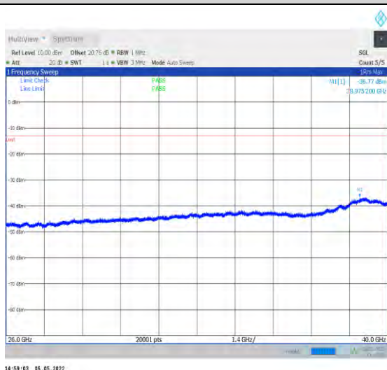
1-N77-3700-3980-PC2-30-100-L-1-DFT-QPSK-Edge _1RB_Left-1@0-26000-40000-Ant1--36.77--13-PAS S
