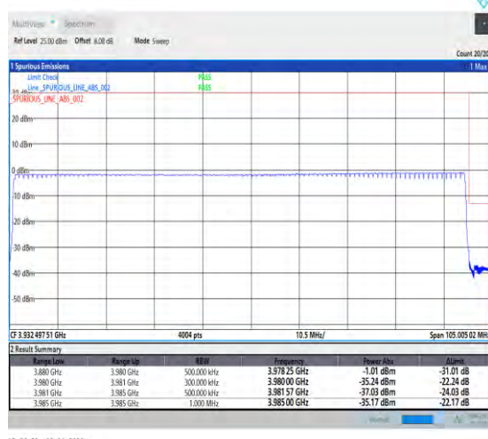
1-N77-3700-3980-PC2-30-100-H-6-CP-QPSK-Out er_Full-273@0-Ant1-PASS-see graph
