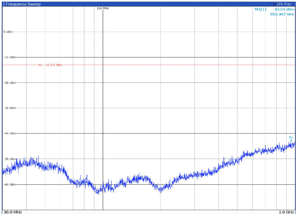
Channel: TOP, Modulation: 64QAM, BW=60MHz, Range: 30MHz - 1GHz, Polarization: Horizontal
