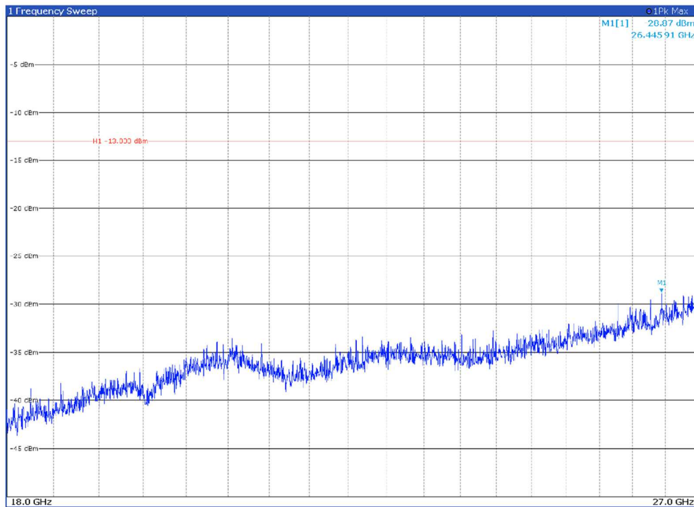
Channel: MIDDLE, Modulation: 64QAM, BW=60MHz, Range: 18GHz - 27GHz, Polarization: Vertical
