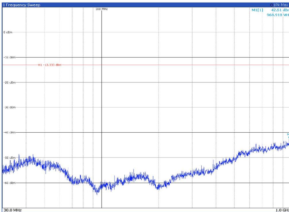
Channel: MIDDLE, Modulation: 64QAM, BW=70MHz, Range: 30MHz - 1GHz, Polarization: Horizontal
