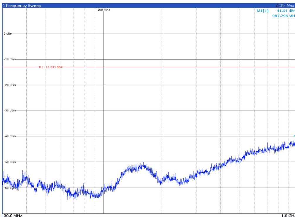
Channel: MIDDLE, Modulation: 64QAM, BW=70MHz, Range: 30MHz - 1GHz, Polarization: Vertical
