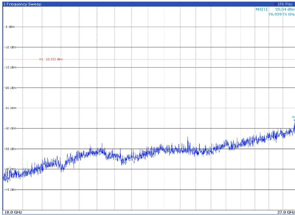
Channel: MIDDLE, Modulation: 64QAM, BW=60MHz, Range: 18GHz - 27GHz, Polarization: Horizontal
