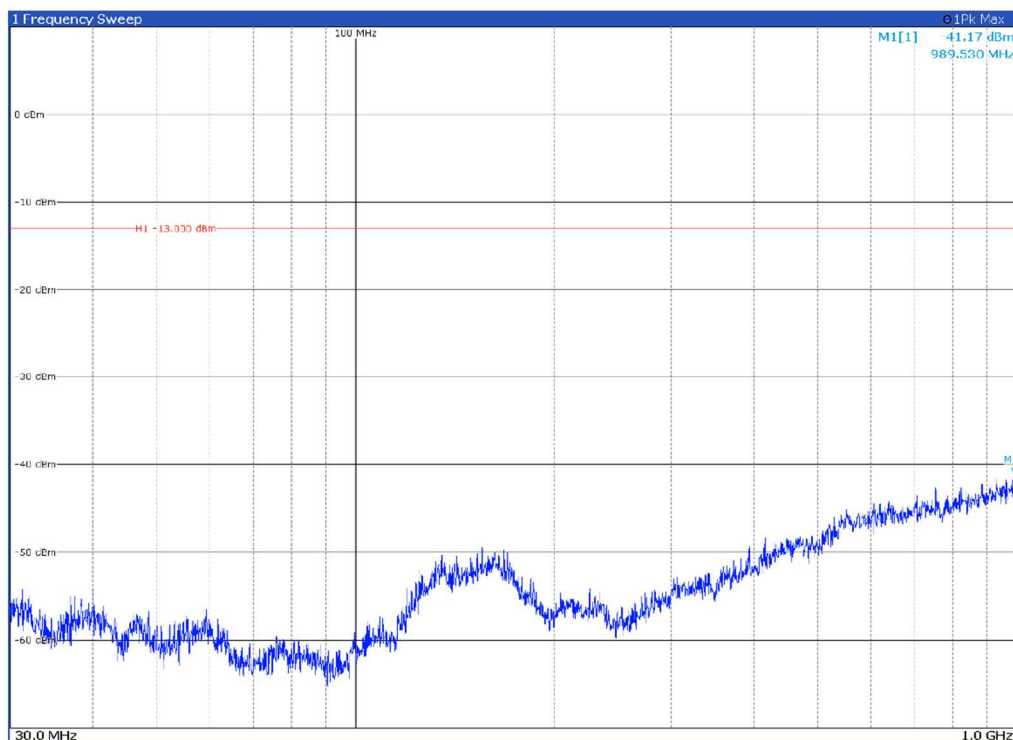
Channel: MIDDLE, Modulation: 64QAM, BW=60MHz, Range: 30MHz - 1GHz, Polarization: Vertical
