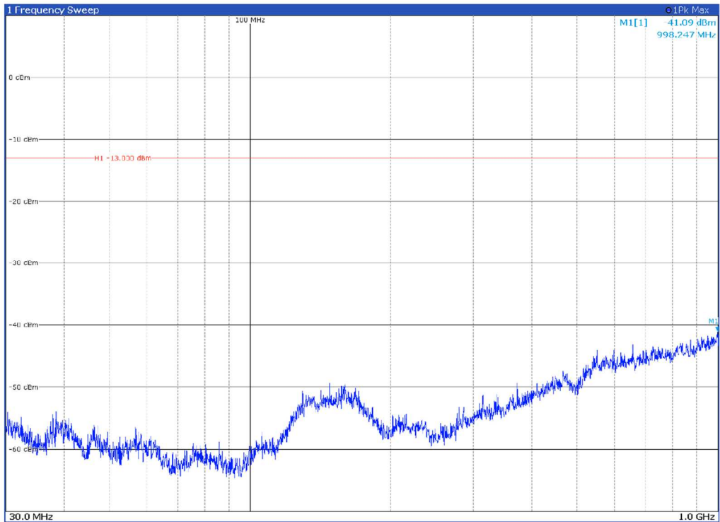
Channel: TOP, Modulation: 64QAM, BW=60MHz, Range: 30MHz - 1GHz, Polarization: Vertical
