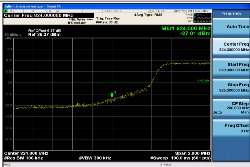
Band5-10MHz-16QAM-20450-50RB#0
