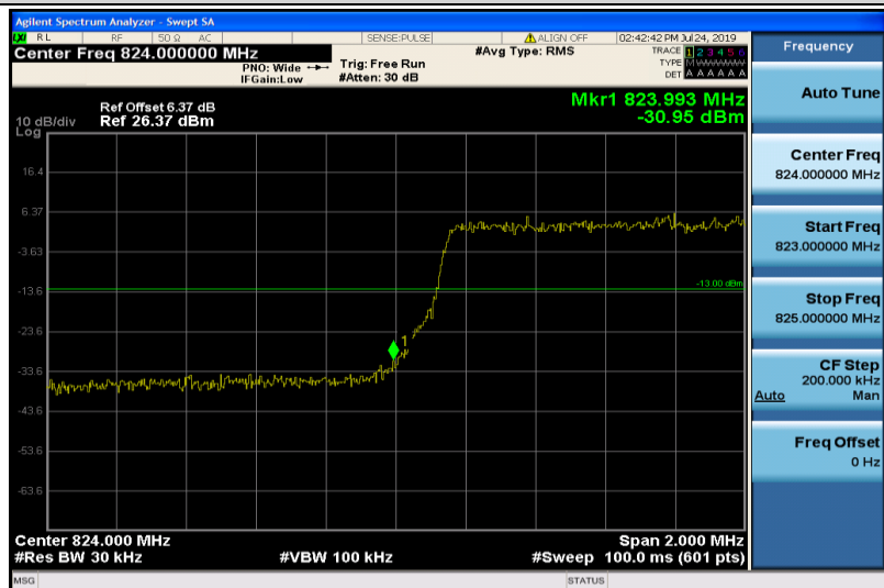
Band5-3MHz-16QAM-20415-15RB#0
