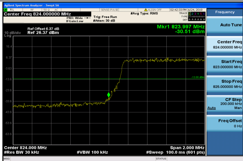
Band5-3MHz-QPSK-20415-15RB#0
