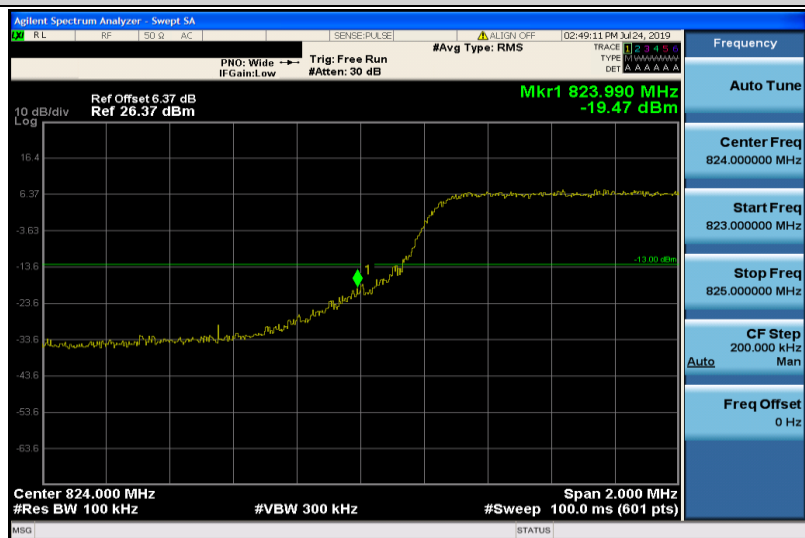
Band5-5MHz-QPSK-20425-25RB#0
