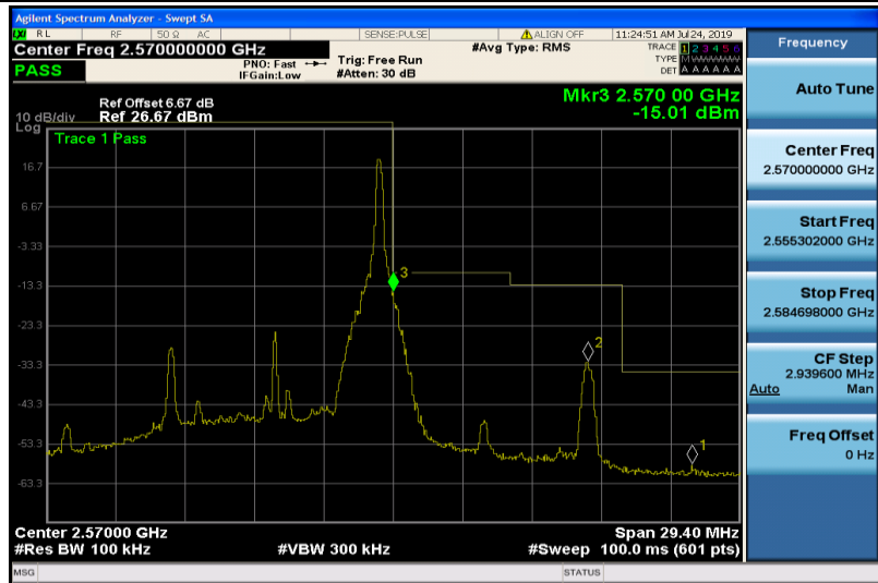
Band7-10MHz-16QAM-21400-1RB#49
