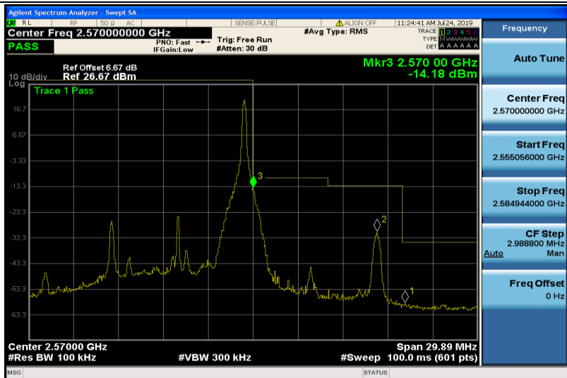
Band7-10MHz-QPSK-21400-1RB#49
