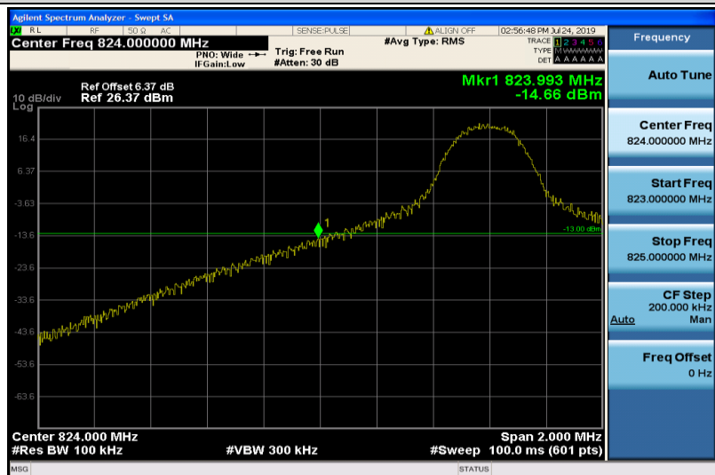
Band5-10MHz-16QAM-20450-1RB#0
