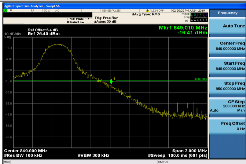
Band5-5MHz-16QAM-20625-1RB#24
