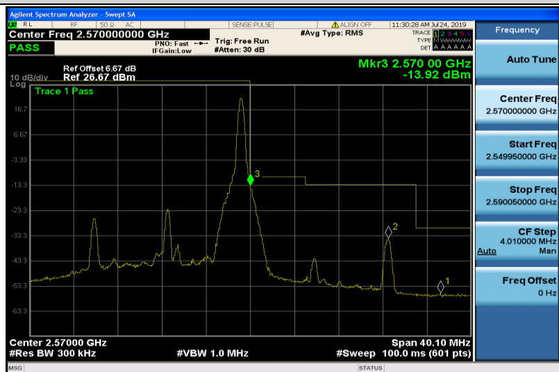
Band7-15MHz-QPSK-21375-1RB#74
