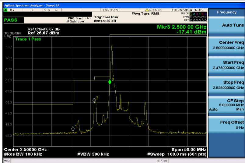
Band7-5MHz-16QAM-20775-1RB#0
