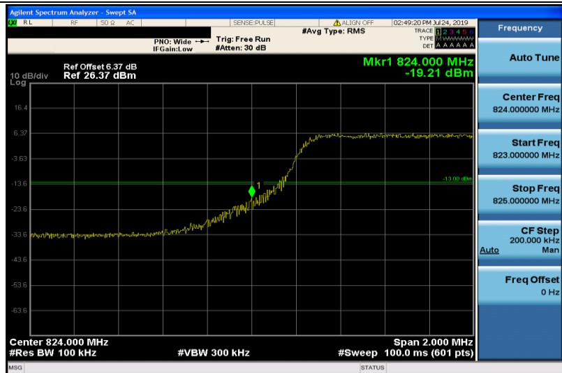
Band5-5MHz-16QAM-20425-25RB#0
