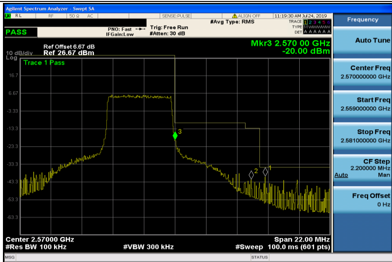
Band7-5MHz-16QAM-21425-25RB#0
