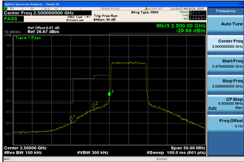
Band7-10MHz-16QAM-20800-50RB#0
