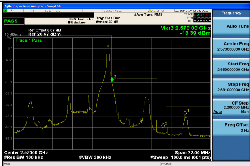
Band7-5MHz-QPSK-21425-1RB#24
