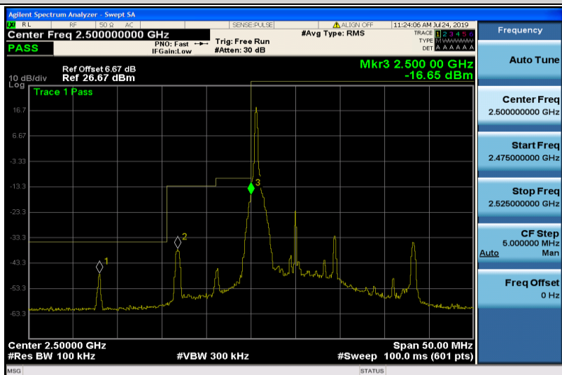
Band7-10MHz-16QAM-20800-1RB#0
