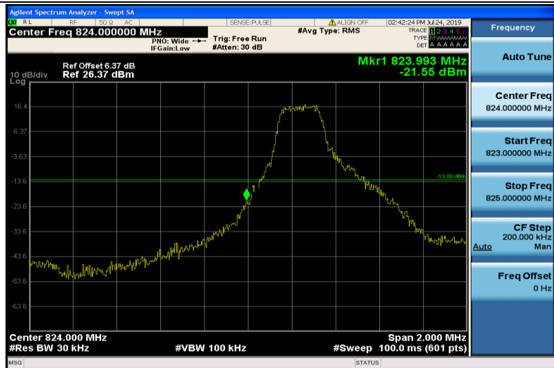
Band5-3MHz-16QAM-20415-1RB#0
