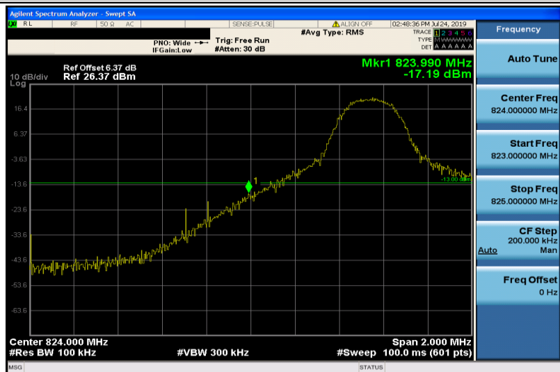
Band5-5MHz-QPSK-20425-1RB#0
