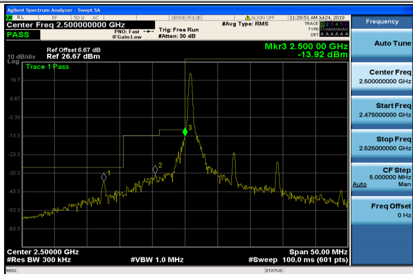
Band7-15MHz-16QAM-20825-1RB#0
