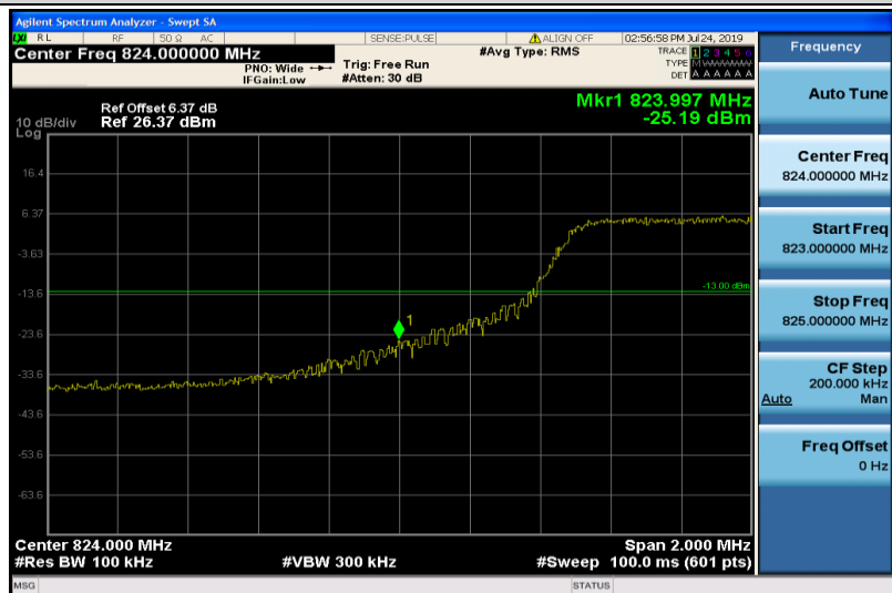
Band5-10MHz-QPSK-20450-50RB#0
