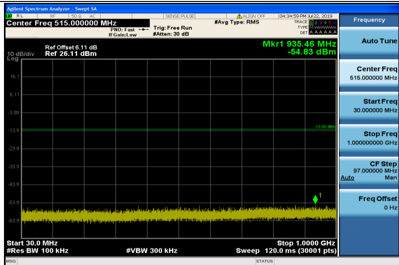
Band2-1.4MHz-16QAM-18607-1RB#0-30~1000MHz
