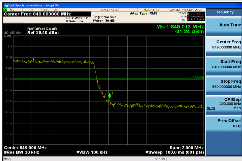
Band5-3MHz-16QAM-20635-15RB#0
