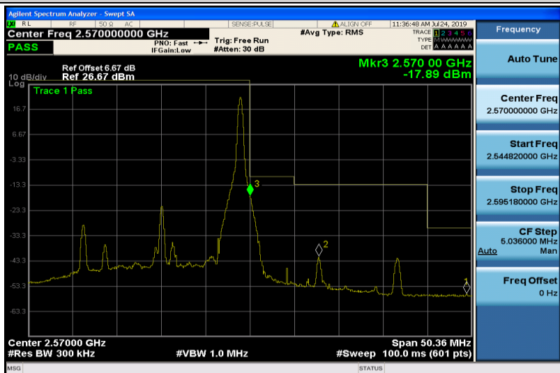
Band7-20MHz-QPSK-21350-1RB#99
