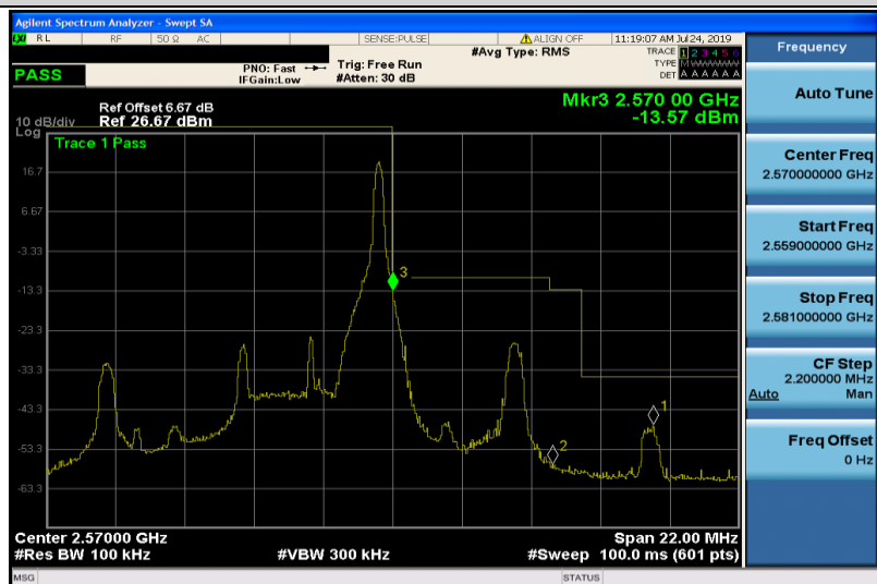
Band7-5MHz-16QAM-21425-1RB#24
