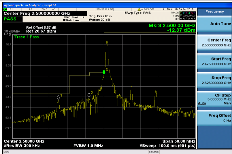
Band7-15MHz-QPSK-20825-1RB#0
