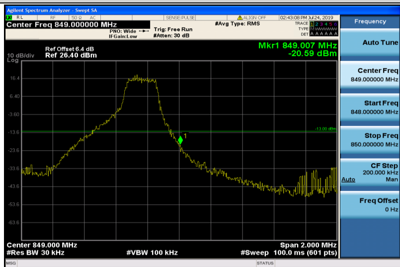
Band5-3MHz-16QAM-20635-1RB#14
