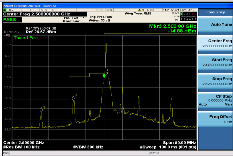
Band7-10MHz-QPSK-20800-1RB#0
