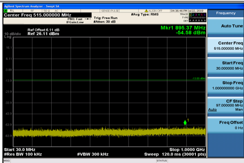
Band2-1.4MHz-16QAM-18900-1RB#0-30~1000MHz
