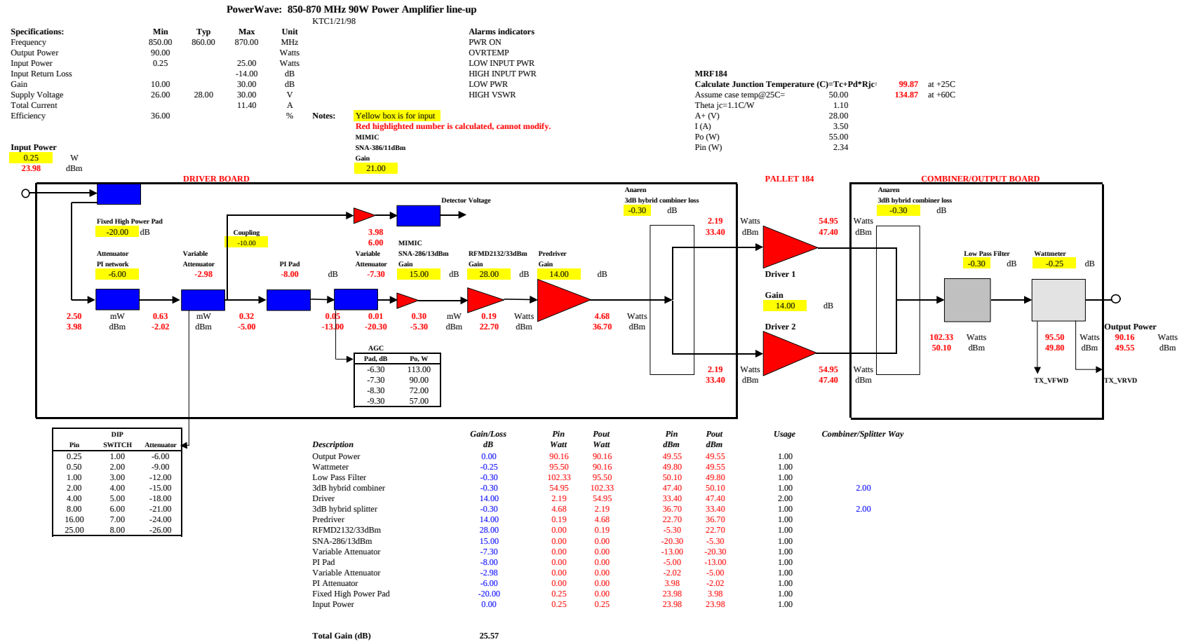
Figure 4-2. K10 Block diagram
