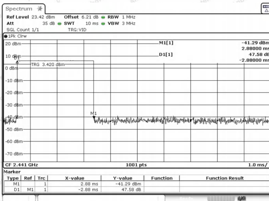
Dwell_Time_(Hopping)_NVNT_ANT1_1-DH5_2441_One_Burst_Time
