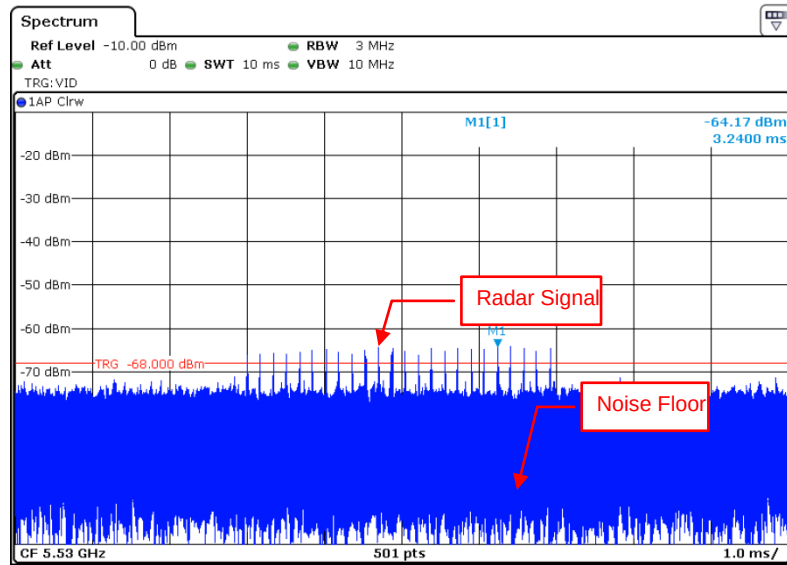
Radar Signal 2
