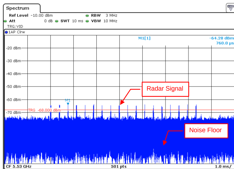
Radar Signal 3
