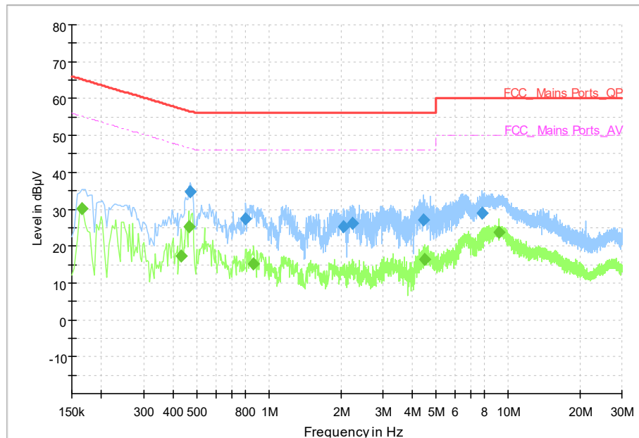
Fig.66 AC Power line Conducted Emission (Traffic)
