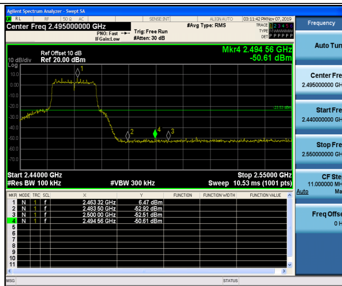
11N20SISO_Ant2_High_2462
