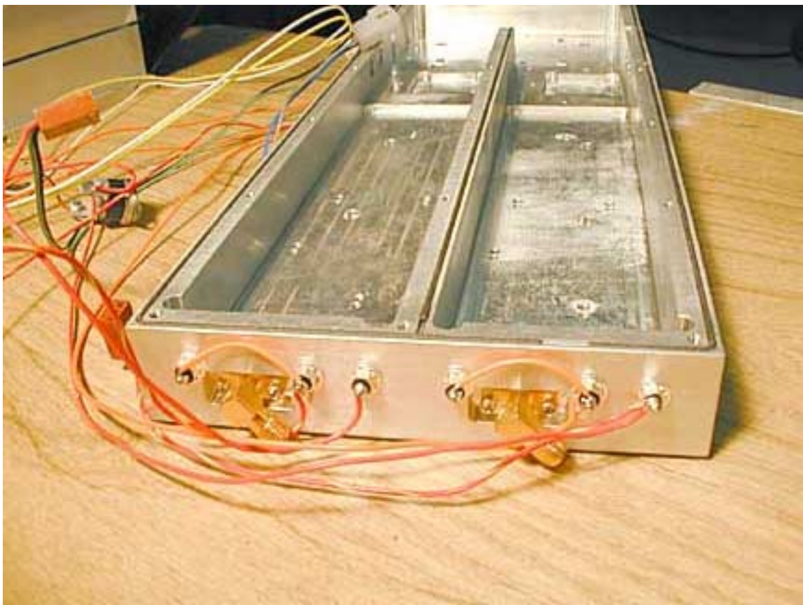
RF Enclosure Front
