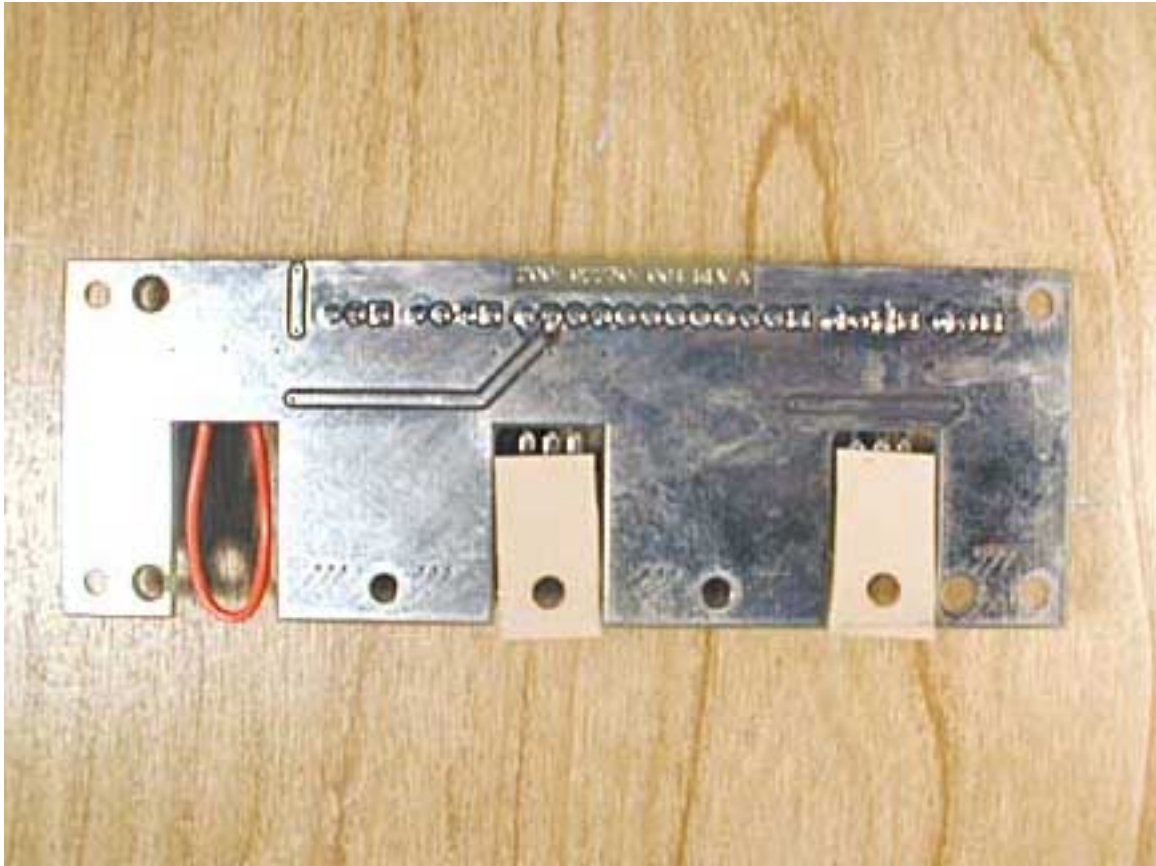
500-02230 PCB Back
