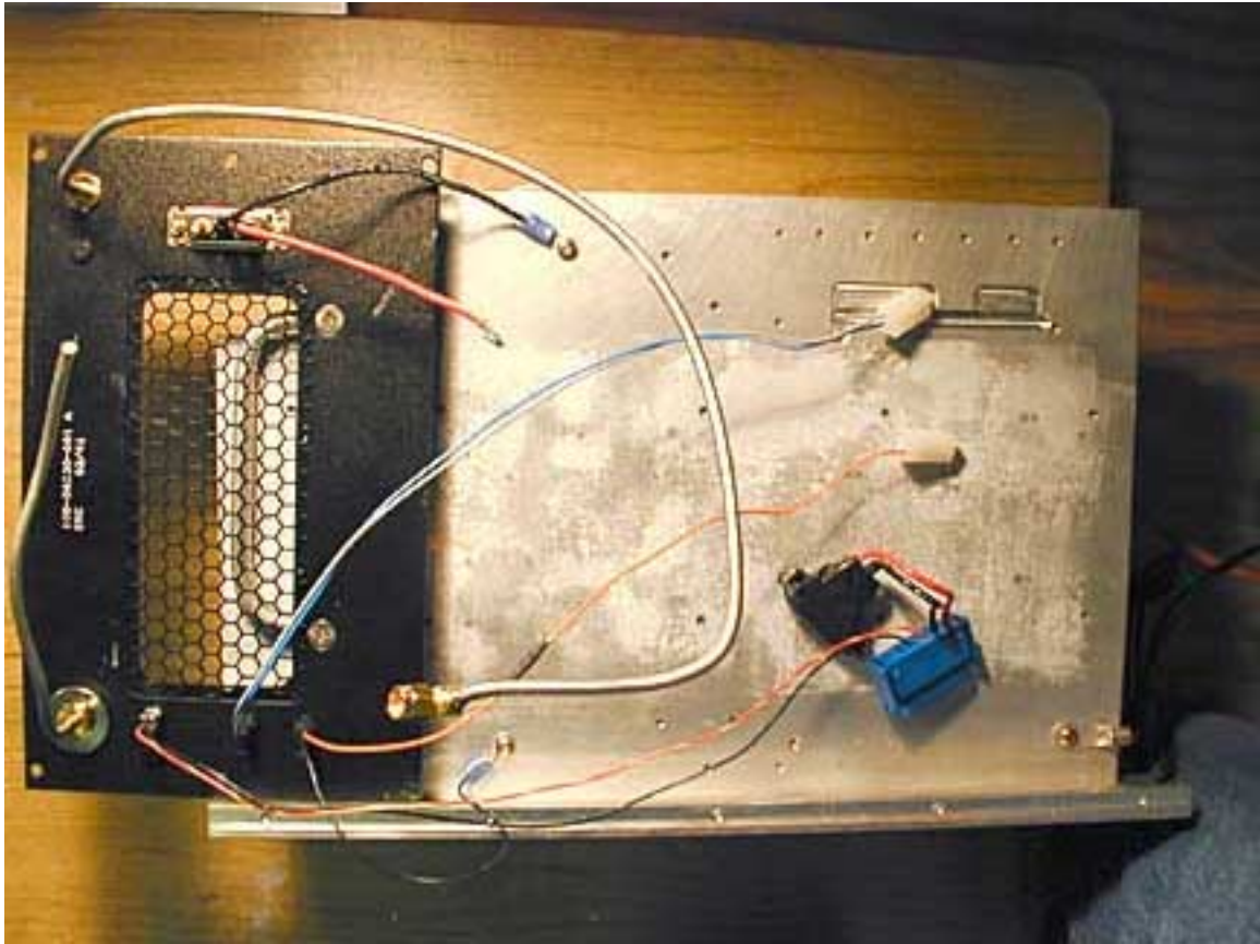
Backside of RF Front Panel
