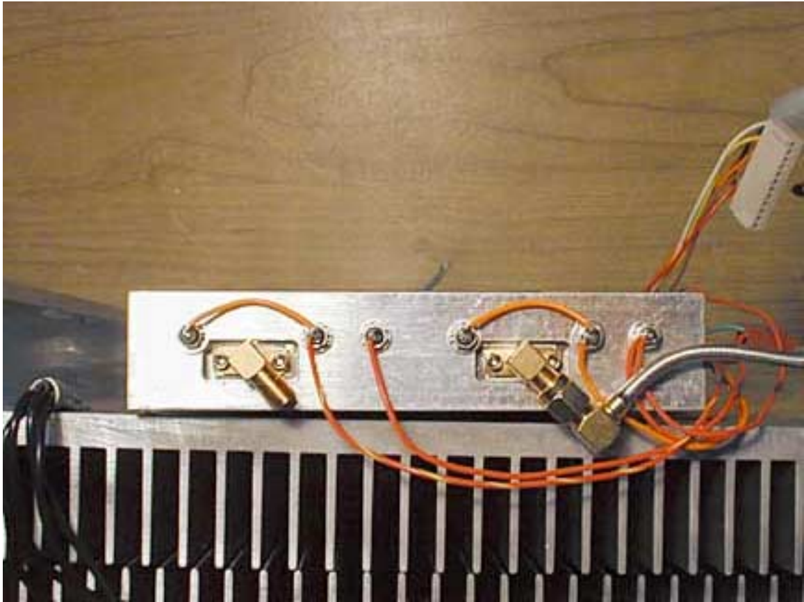
RF Input of RF Enclosure
