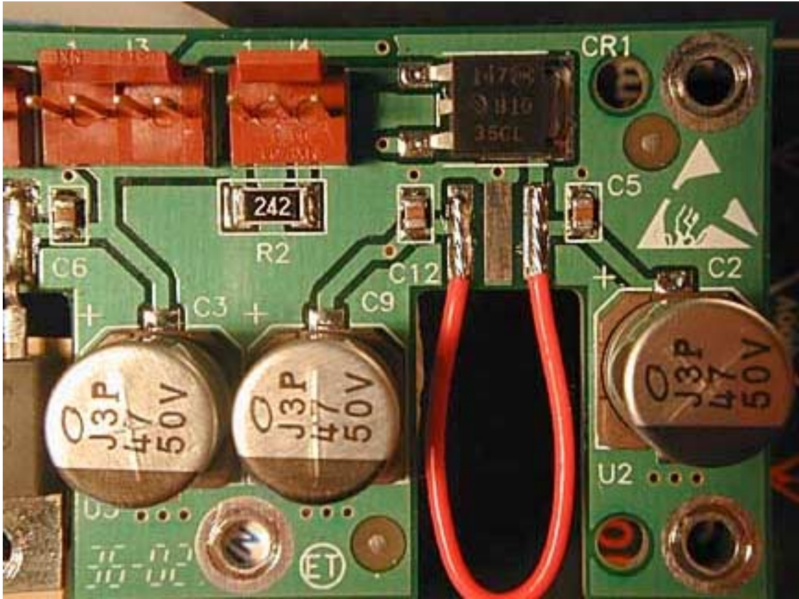
500-02230 PCB Section 3
