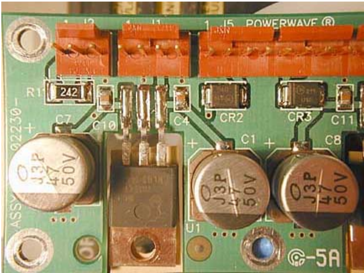
500-02230 PCB Section 1
