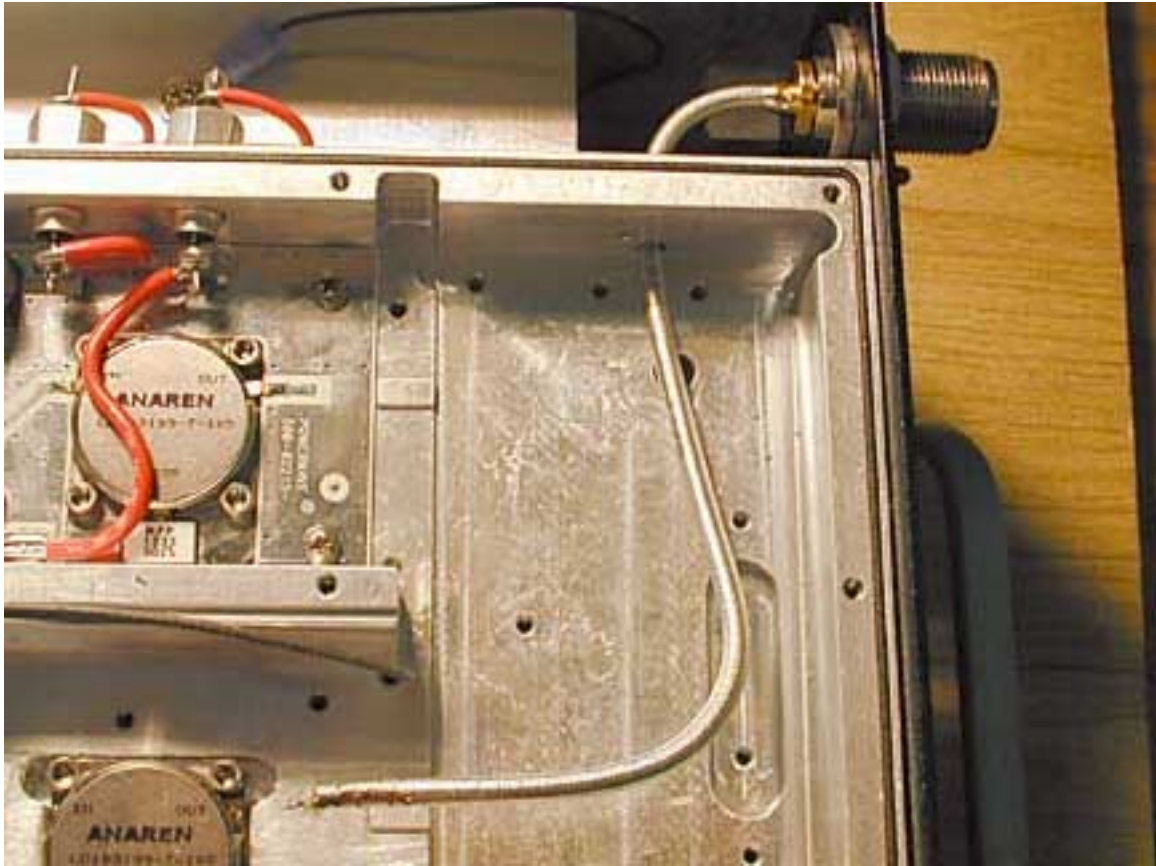
RF Output Cable
