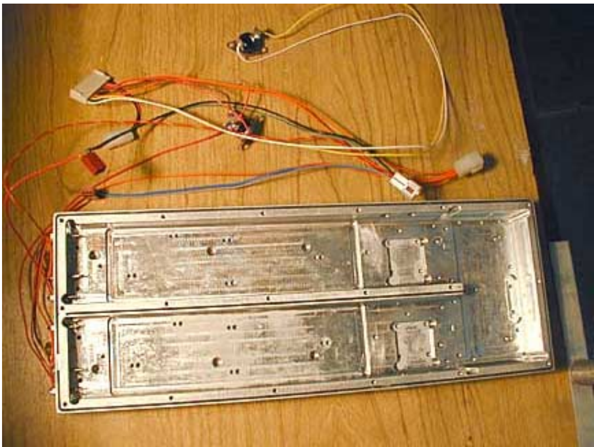
RF Enclosure Top
