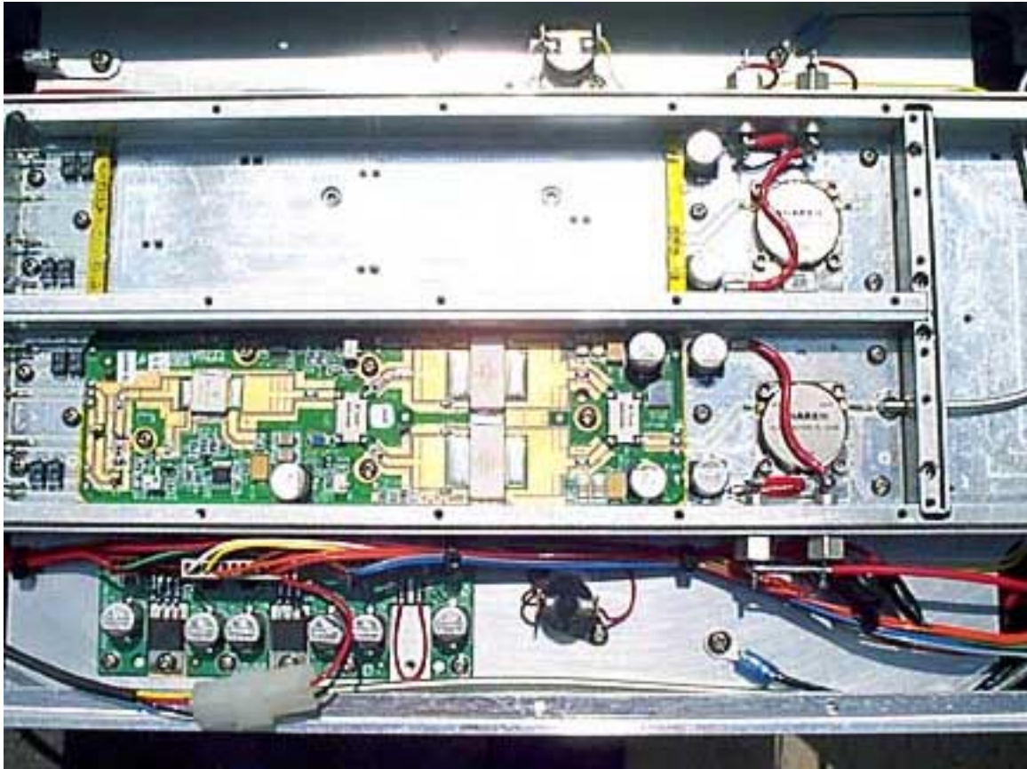
RF Section Top Exposed
