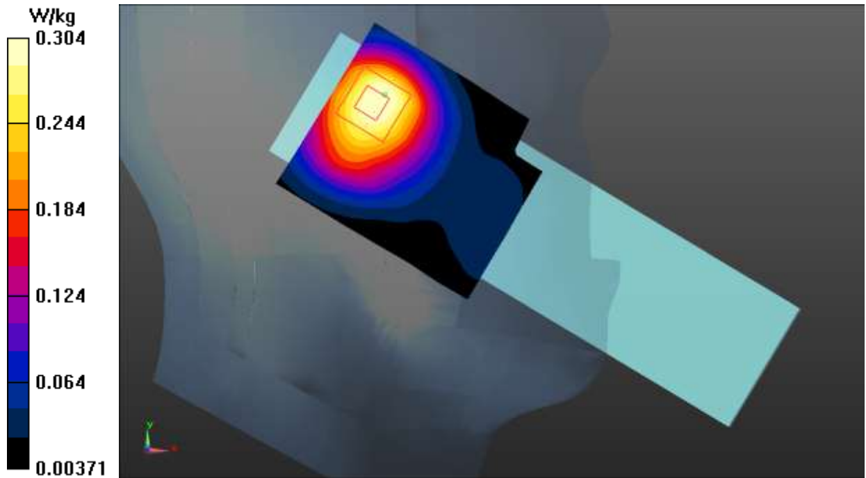
Fig.13 WCDMA Band 4
