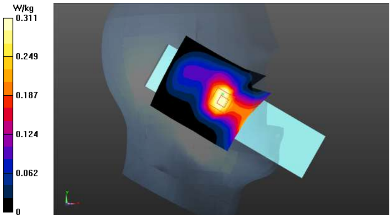
Fig.23 LTE Band 25
