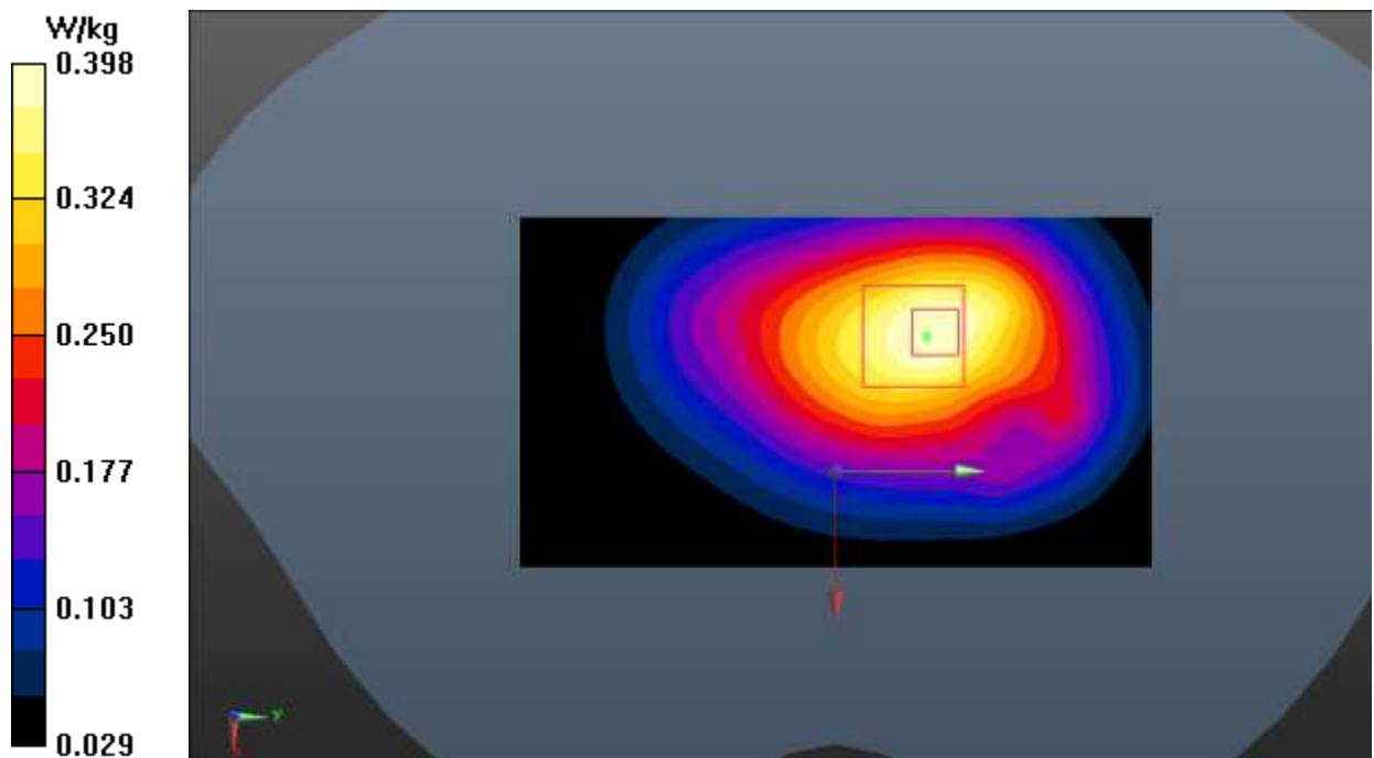
Fig.20 LTE Band 12
