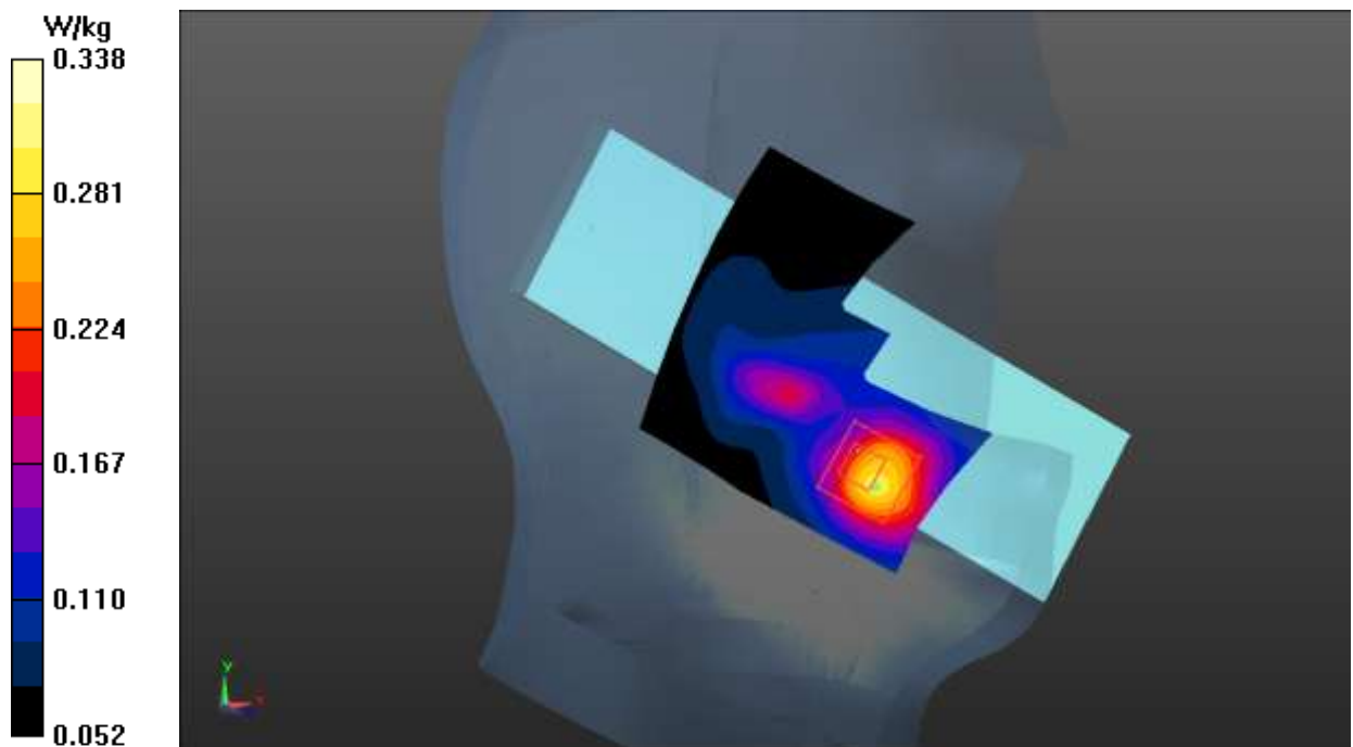
Fig.27 LTE Band 41
