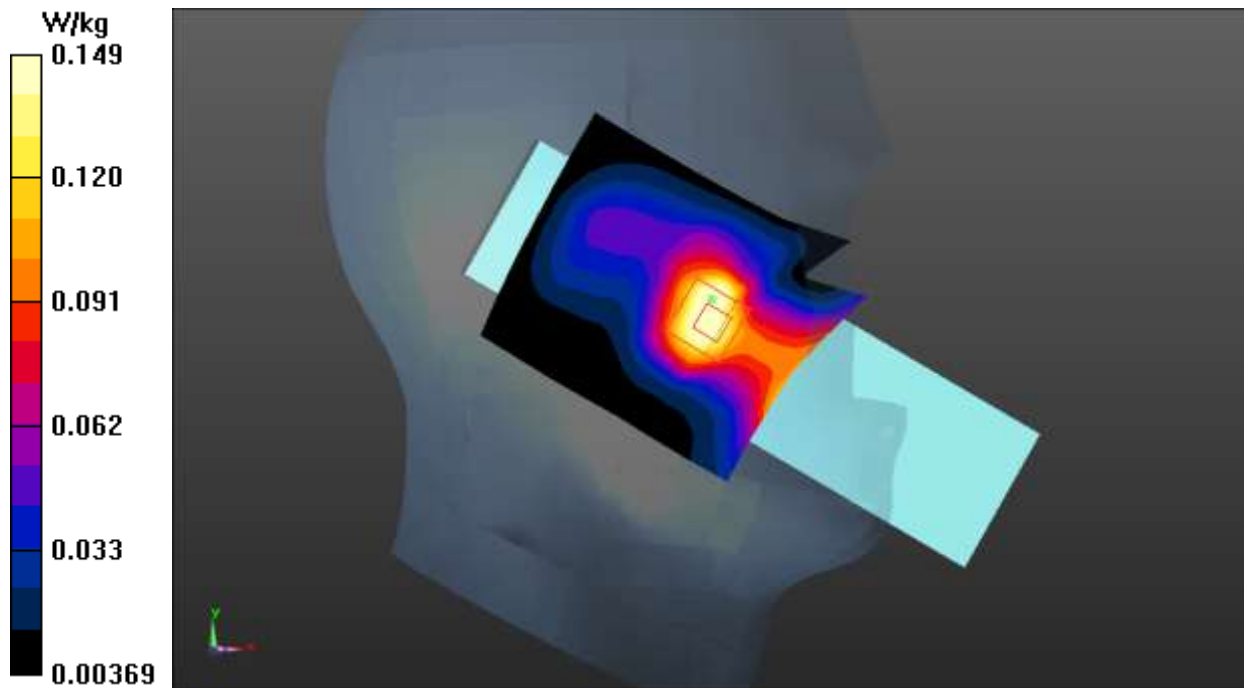
Fig.11 WCDMA Band 2
