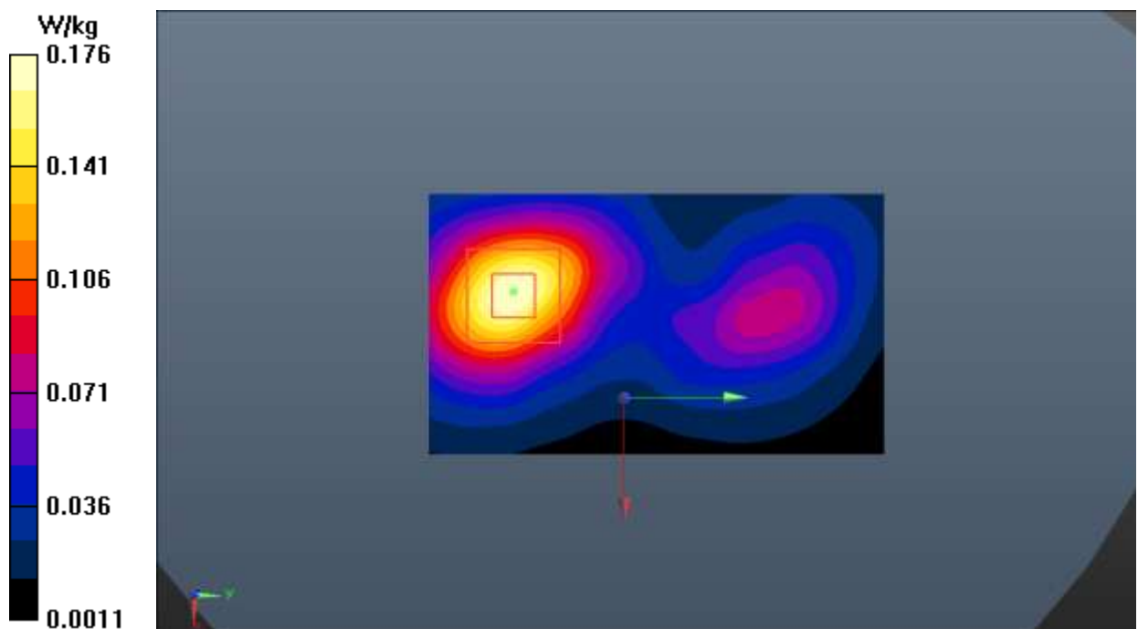
Fig.34 WLAN 2.4G
