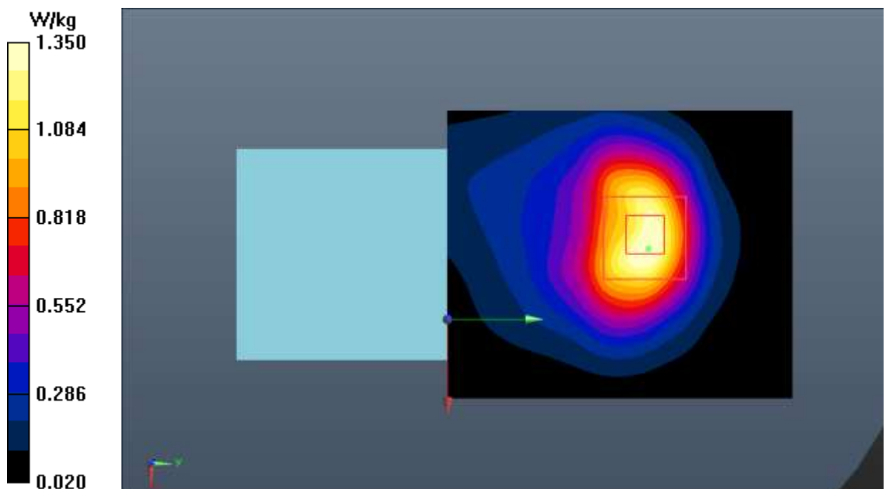
Fig.24 LTE Band 25
