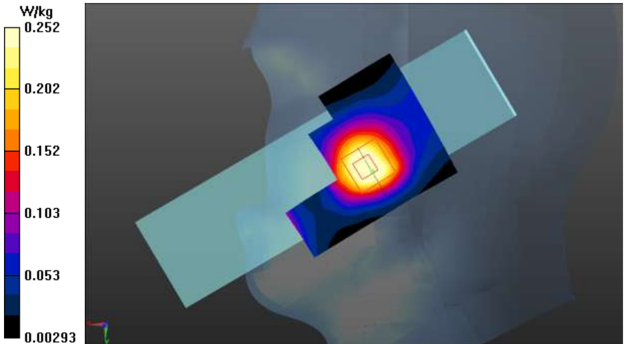
Fig.29 LTE Band 66
