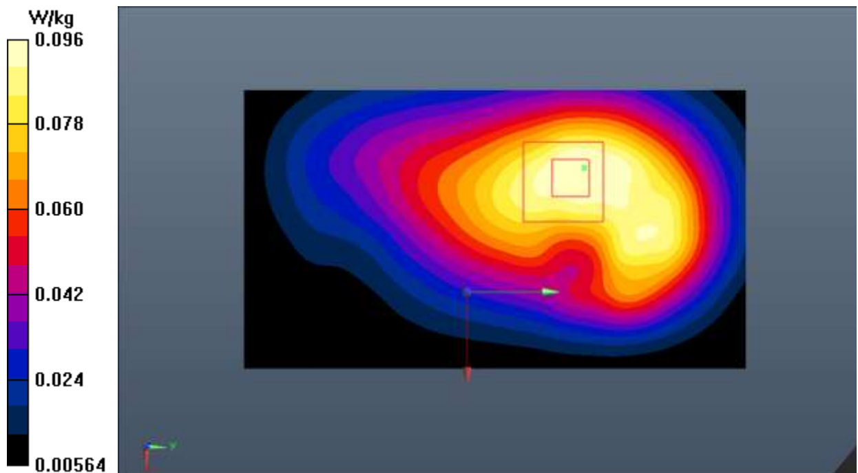
Fig.22 LTE Band 13
