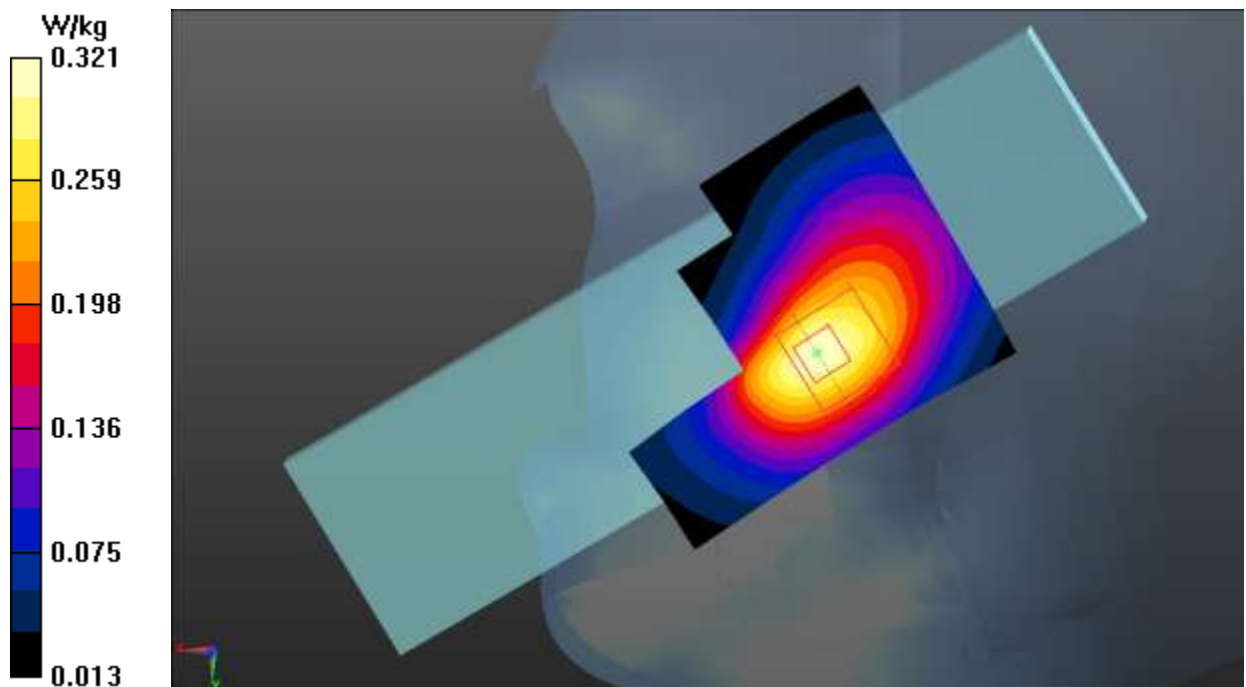
Fig.25 LTE Band 26
