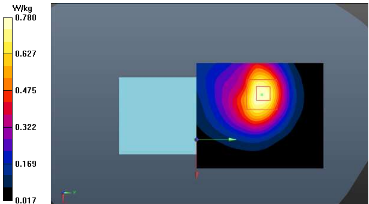
Fig.8 CDMA BC1
