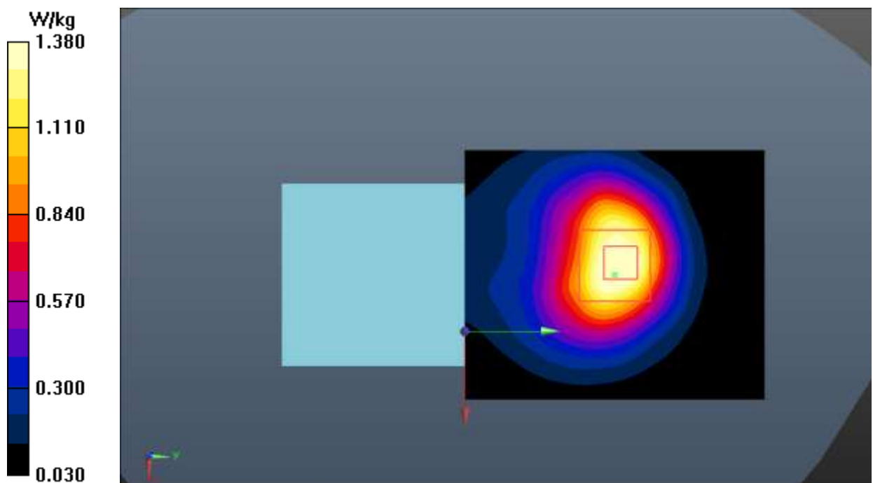
Fig.30 LTE Band 66
