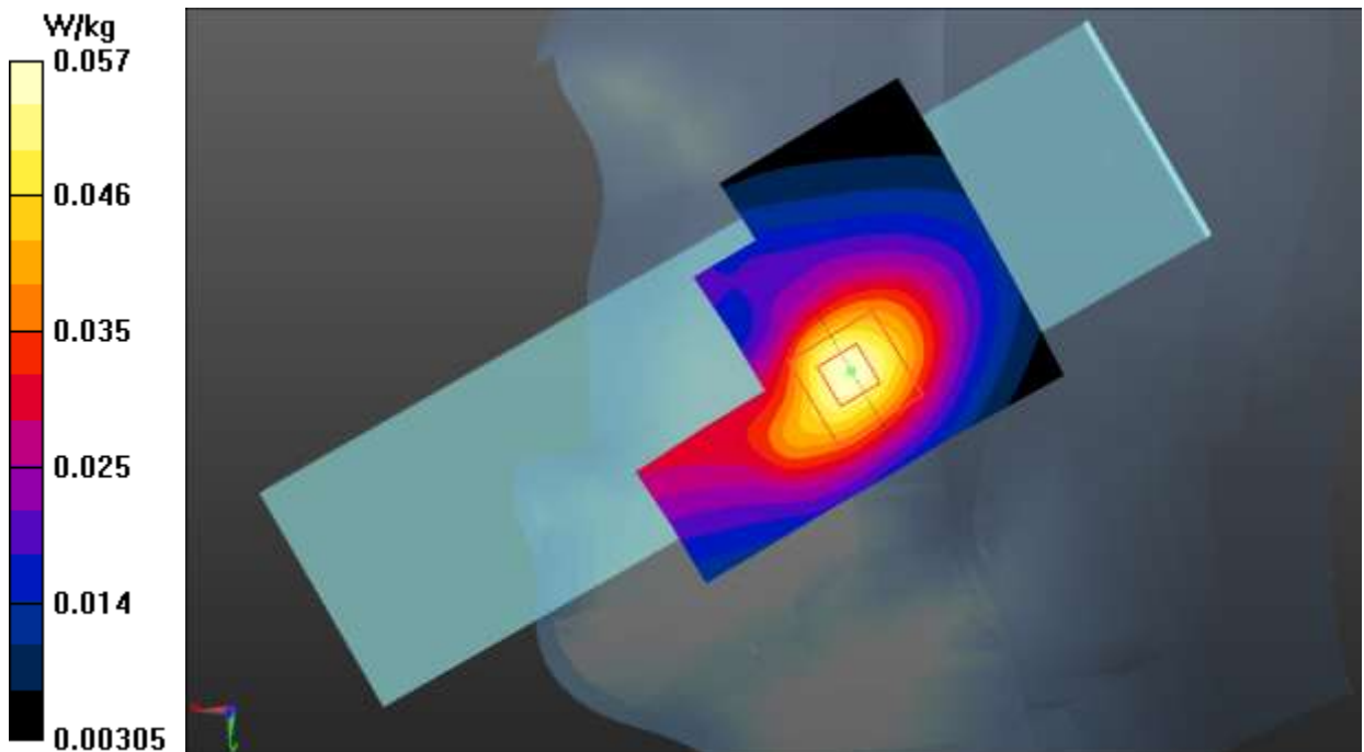
Fig.31 LTE Band 71
