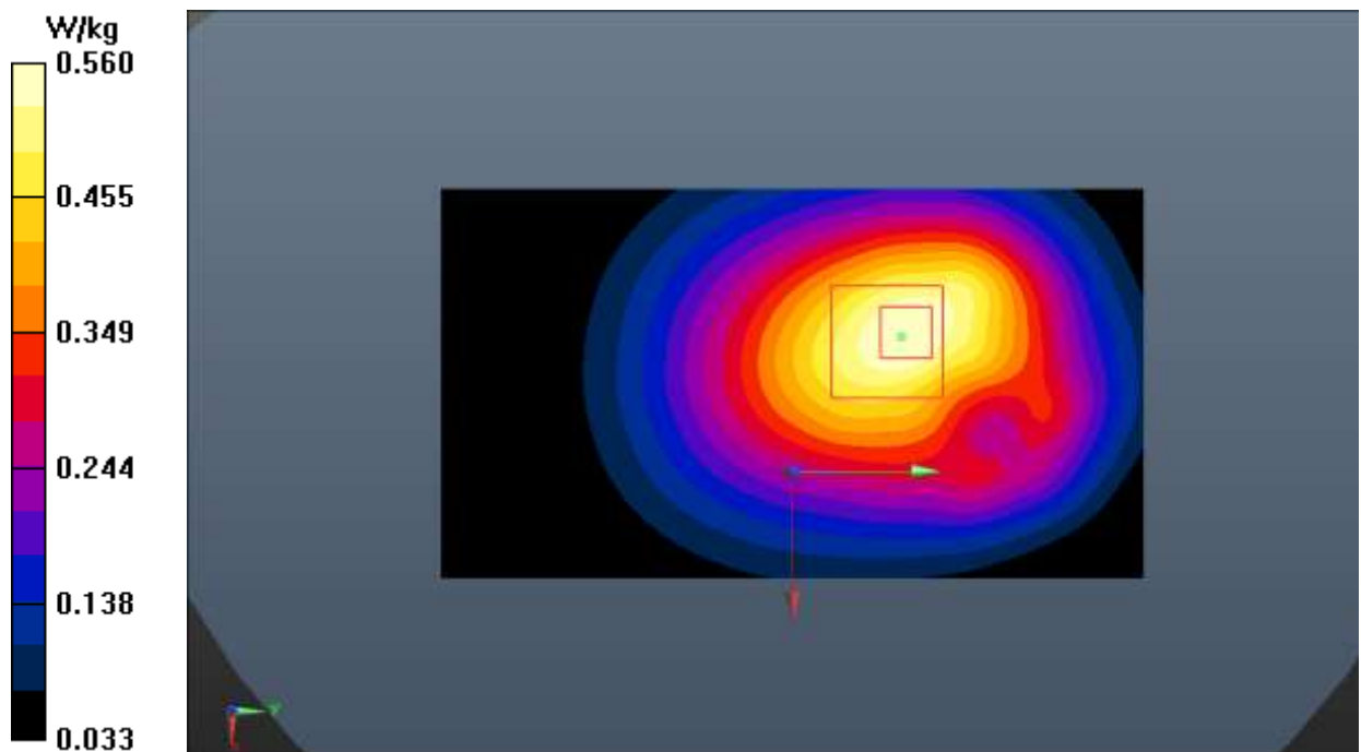
Fig.16 WCDMA Band 5
