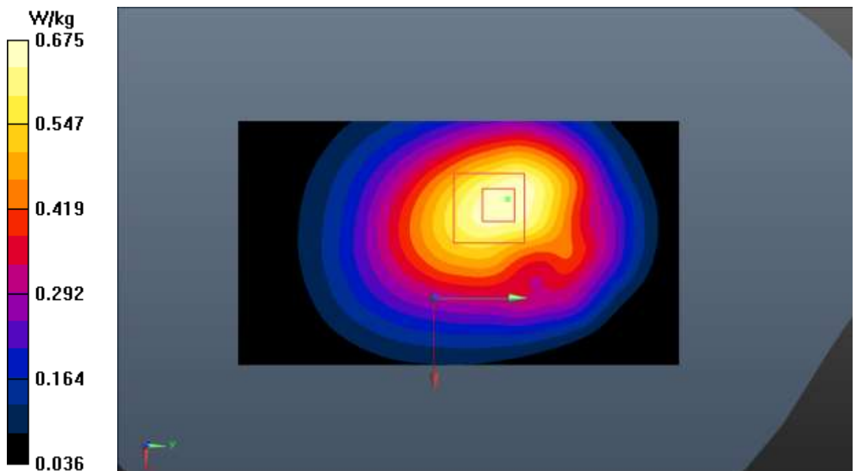
Fig.18 LTE Band 5
