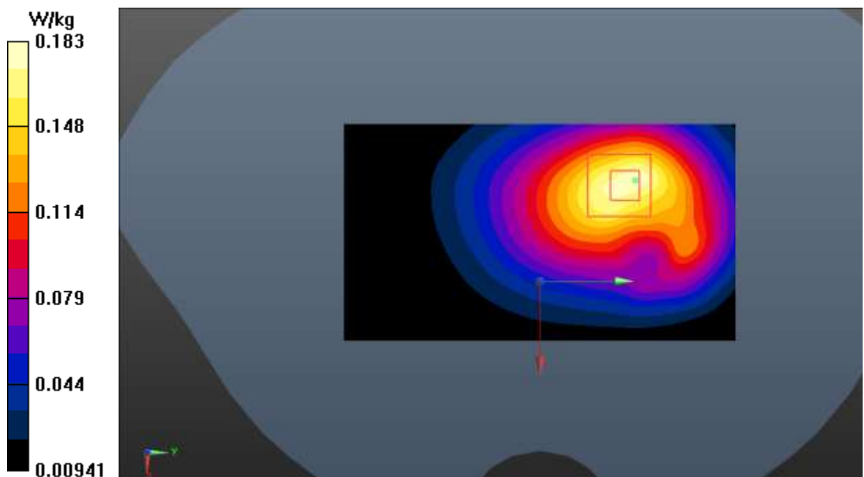
Fig.32 LTE Band 71
