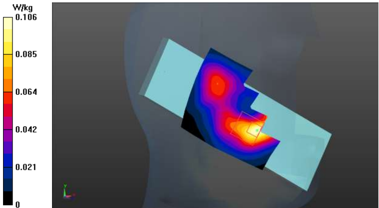
Fig.33 WLAN 2.4G
