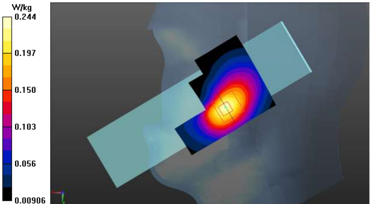
Fig.17 LTE Band 5
