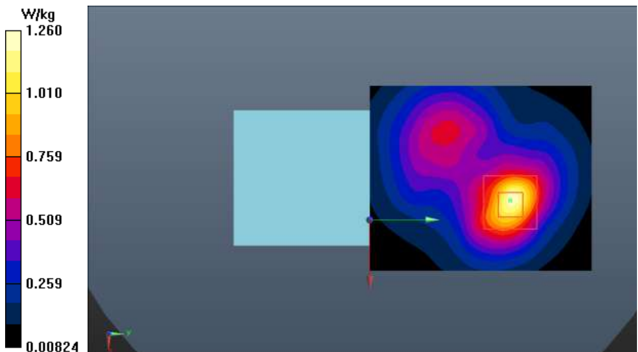
Fig.28 LTE Band 41
