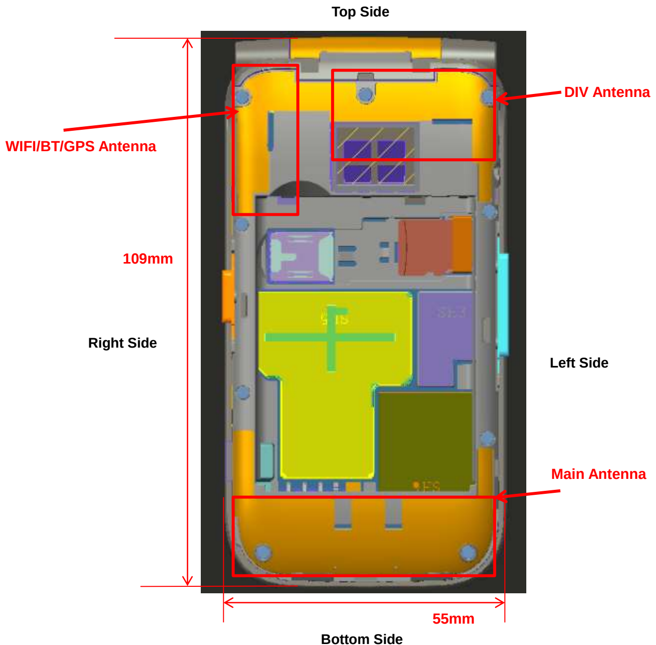
Picture 12.1 Antenna Locations (Back View)
