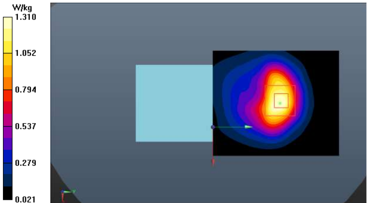
Fig.12 WCDMA Band 2
