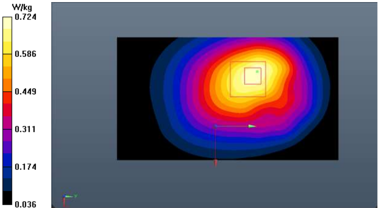
Fig.26 LTE Band 26
