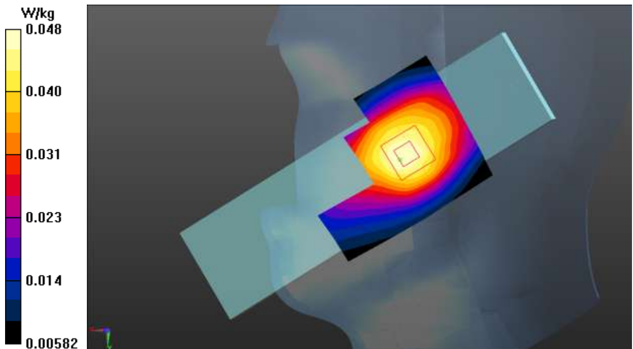
Fig.21 LTE Band 13
