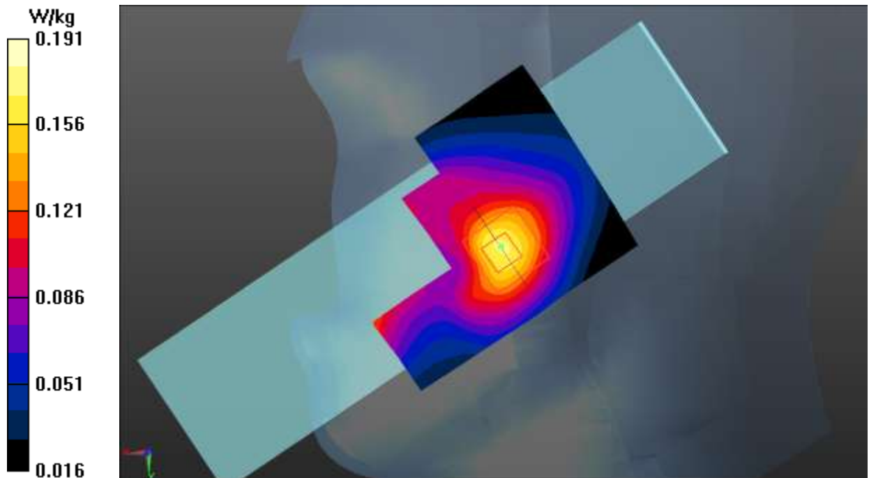
Fig.1 GSM 850
