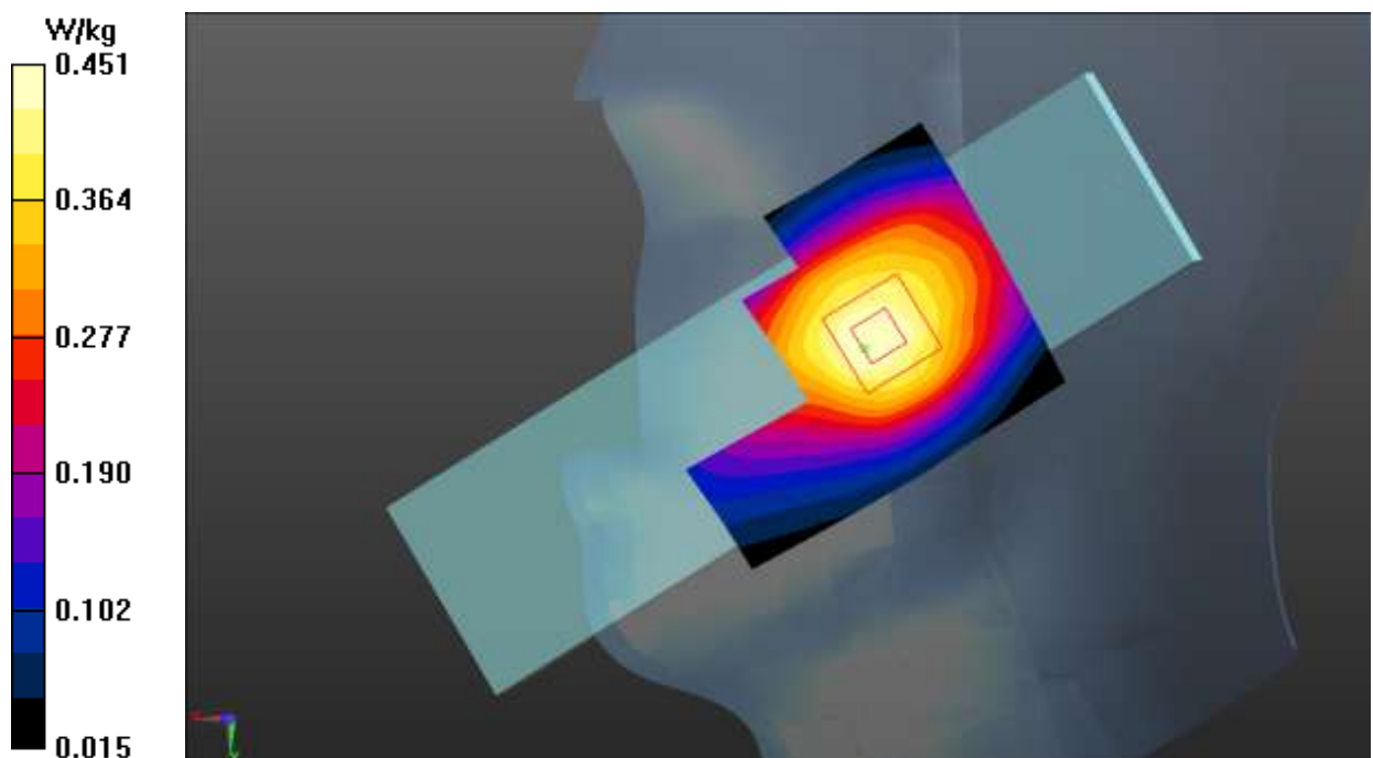
Fig.15 WCDMA Band 5
