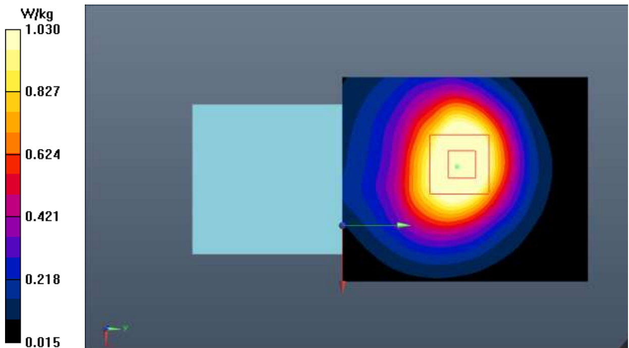
Fig.14 WCDMA Band 4
